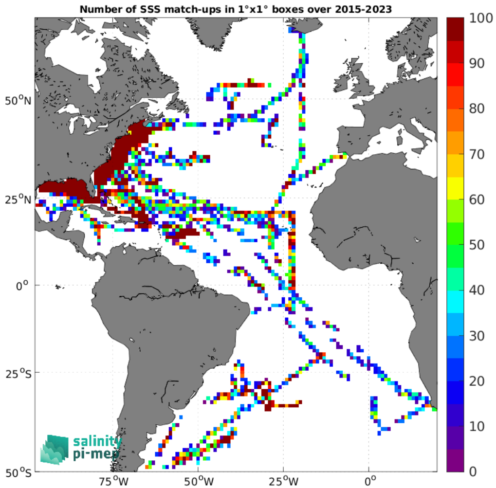
Figure 4: Number of SSS match-ups between TSG (SAMOS) SSS and the SMAP SSS L2 v5 - 40 km (RSS) SSS product for the Atlantic Ocean Pi-MEP region over 1^\circ \times 1^\circ boxes and for the full satellite product period.
