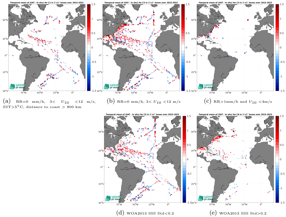
Figure 12: Temporal mean gridded over spatial boxes of size 1^\circ \times 1^\circ of \Delta SSS (SMAP SSS L2 v5 - 40 km (RSS) - TSG (SAMOS)) for 5 different subdatasets corresponding to:RR=0 mm/h, 3 < U_{10} < 12 m/s, SST >5^\circ\text{C} , distance to coast > 800 km (a), RR=0 mm/h, 3 < U_{10} < 12 m/s (b), RR >1 mm/h and U_{10} < 4 m/s (c), WOA2013 SSS Std <0.2 (d), WOA2013 SSS Std >0.2 (e).
