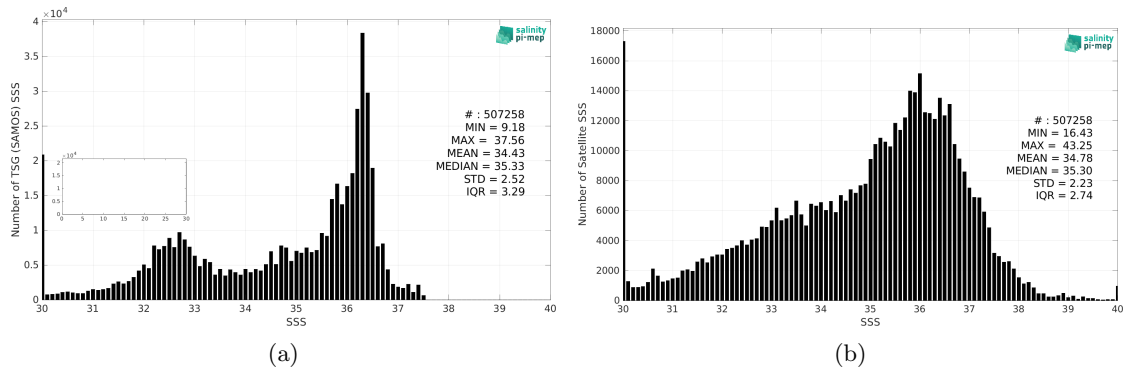
Figure 2: Histograms of SSS from TSG (SAMOS) (a) and SMAP SSS L2 v5 - 40 km (RSS) (b) considering all match-up pairs per bins of 0.1 over the Atlantic Ocean Pi-MEP region and for the full satellite product period.
