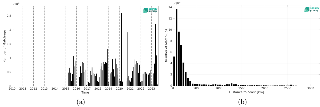
Figure 1: Number of match-ups between TSG (SAMOS) and SMAP SSS L2 v5 - 40 km (RSS) SSS as a function of time (a) and as function of the distance to coast (b) over the Atlantic Ocean Pi-MEP region and for the full satellite product period.
