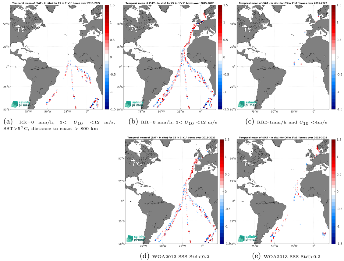
Figure 12: Temporal mean gridded over spatial boxes of size 1^\circ \times 1^\circ of \Delta SSS (SMAP SSS L2 v5 - 40 km (RSS) - TSG (Polarstern)) for 5 different subdatasets corresponding to:RR=0 mm/h, 3 < U_{10} < 12 m/s, SST >5^\circ\text{C} , distance to coast > 800 km (a), RR=0 mm/h, 3 < U_{10} < 12 m/s (b), RR >1 mm/h and U_{10} < 4 m/s (c), WOA2013 SSS Std <0.2 (d), WOA2013 SSS Std >0.2 (e).
