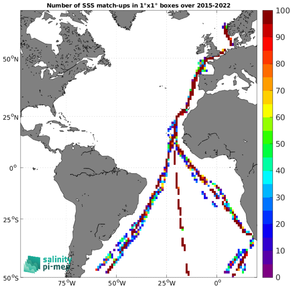
Figure 4: Number of SSS match-ups between TSG (Polarstern) SSS and the SMAP SSS L2 v5 - 40 km (RSS) SSS product for the Atlantic Ocean Pi-MEP region over 1°×1° boxes and for the full satellite product period.
