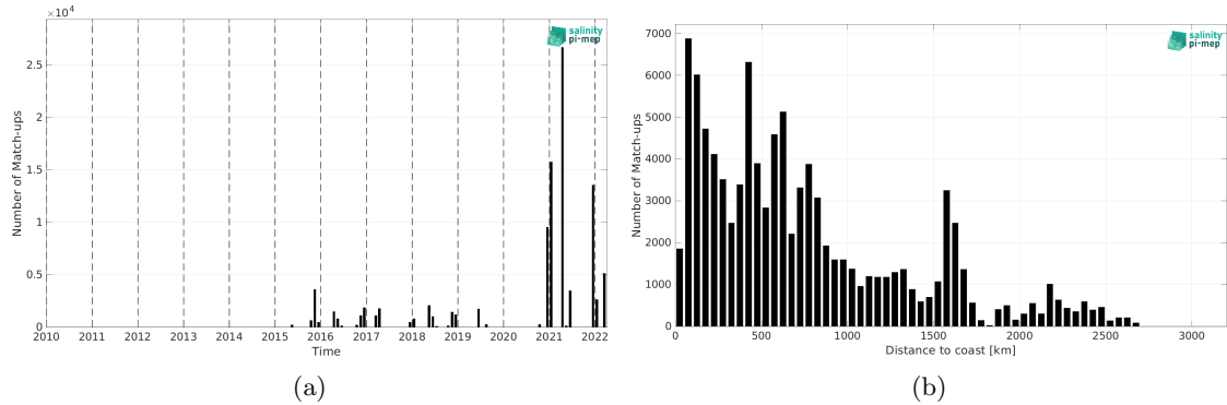
Figure 1: Number of match-ups between TSG (Polarstern) and SMAP SSS L2 v5 - 40 km (RSS) SSS as a function of time (a) and as function of the distance to coast (b) over the Atlantic Ocean Pi-MEP region and for the full satellite product period.
