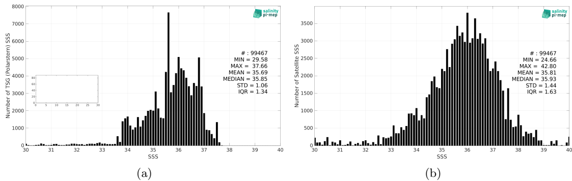
Figure 2: Histograms of SSS from TSG (Polarstern) (a) and SMAP SSS L2 v5 - 40 km (RSS) (b) considering all match-up pairs per bins of 0.1 over the Atlantic Ocean Pi-MEP region and for the full satellite product period.
