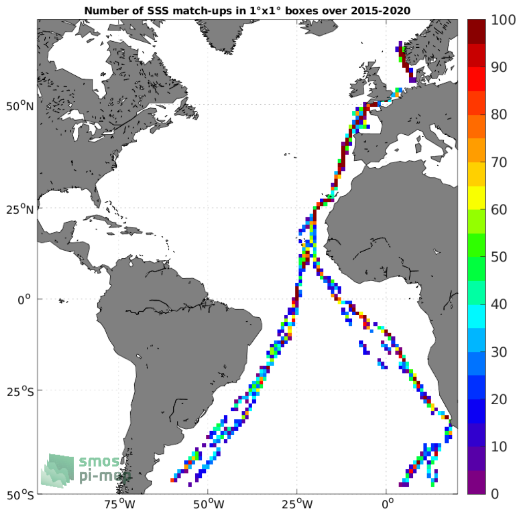
Figure 4: Number of SSS match-ups between TSG (Polarstern) SSS and the SMAP SSS L2 v5 - 40 km (RSS) SSS product for the Atlantic Ocean Pi-MEP region over 1°x1° boxes and for the full satellite product period.
