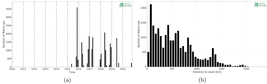
Figure 1: Number of match-ups between TSG (Polarstern) and SMAP SSS L2 v5 - 40 km (RSS) SSS as a function of time (a) and as function of the distance to coast (b) over the Atlantic Ocean Pi-MEP region and for the full satellite product period.
