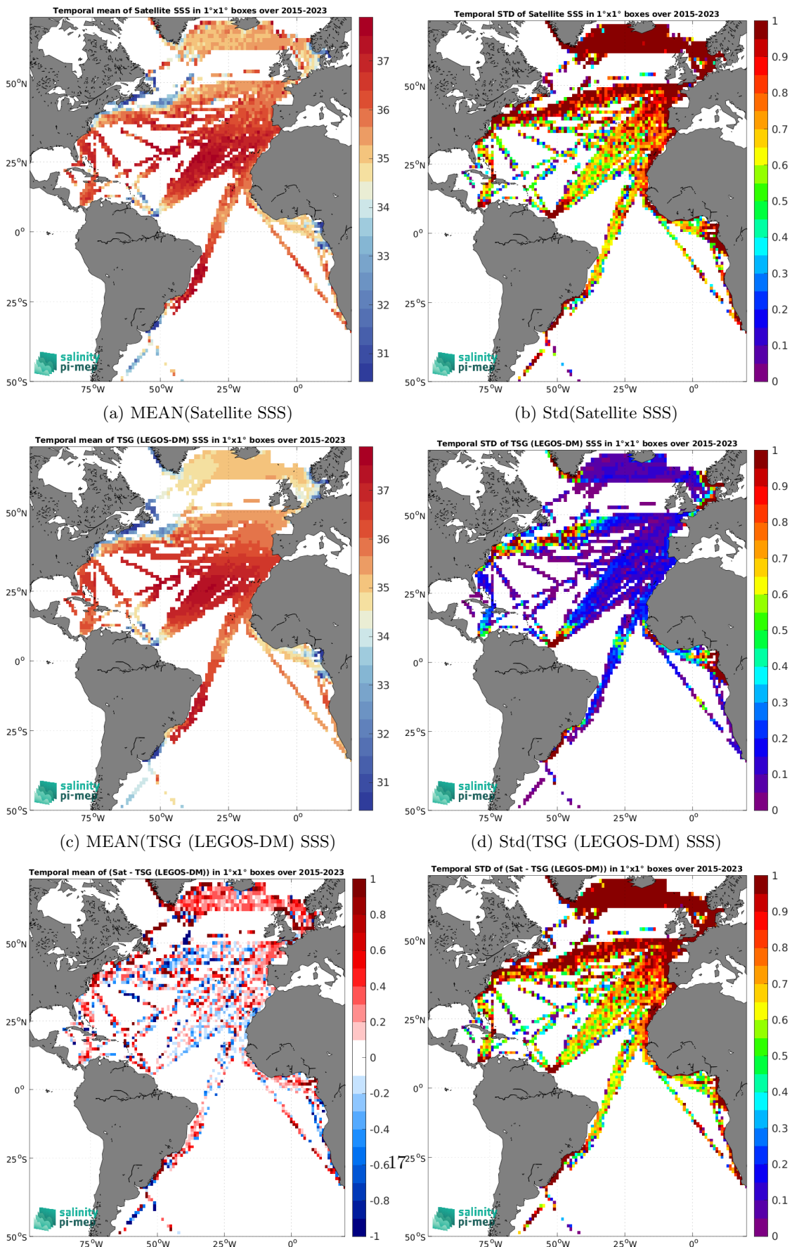
(e) MEAN( \Delta SSS) (Satellite - TSG (LEGOS-DM)) (f) Std( \Delta SSS) (Satellite - TSG (LEGOS-DM)) Figure 6: Temporal mean (left) and Std (right) of SSS from SMAP SSS L2 v5 - 40 km (RSS) (top), TSG (LEGOS-DM) (middle), and of \Delta SSS (Satellite - TSG (LEGOS-DM)). Only match-pairs are used to generate these maps.
