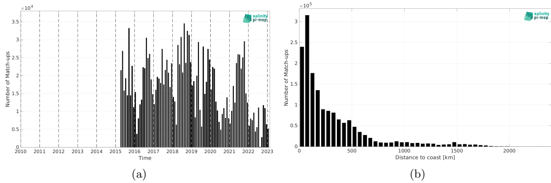
Figure 1: Number of match-ups between TSG (LEGOS-DM) and SMAP SSS L2 v5 - 40 km (RSS) SSS as a function of time (a) and as function of the distance to coast (b) over the Atlantic Ocean Pi-MEP region and for the full satellite product period.
