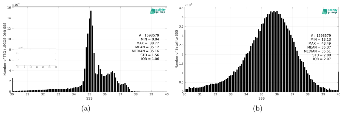
Figure 2: Histograms of SSS from TSG (LEGOS-DM) (a) and SMAP SSS L2 v5 - 40 km (RSS) (b) considering all match-up pairs per bins of 0.1 over the Atlantic Ocean Pi-MEP region and for the full satellite product period.
