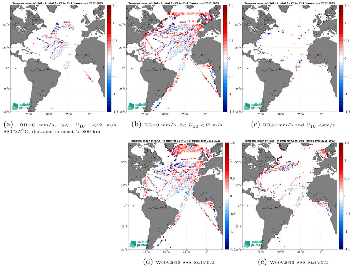
Figure 12: Temporal mean gridded over spatial boxes of size 1^\circ \times 1^\circ of \Delta SSS (SMAP SSS L2 v5 - 40 km (RSS) - TSG (LEGOS-DM)) for 5 different subdatasets corresponding to:RR=0 mm/h, 3 < U_{10} < 12 m/s, SST >5^\circ\text{C} , distance to coast > 800 km (a), RR=0 mm/h, 3 < U_{10} < 12 m/s (b), RR >1 mm/h and U_{10} < 4 m/s (c), WOA2013 SSS Std <0.2 (d), WOA2013 SSS Std >0.2 (e).
