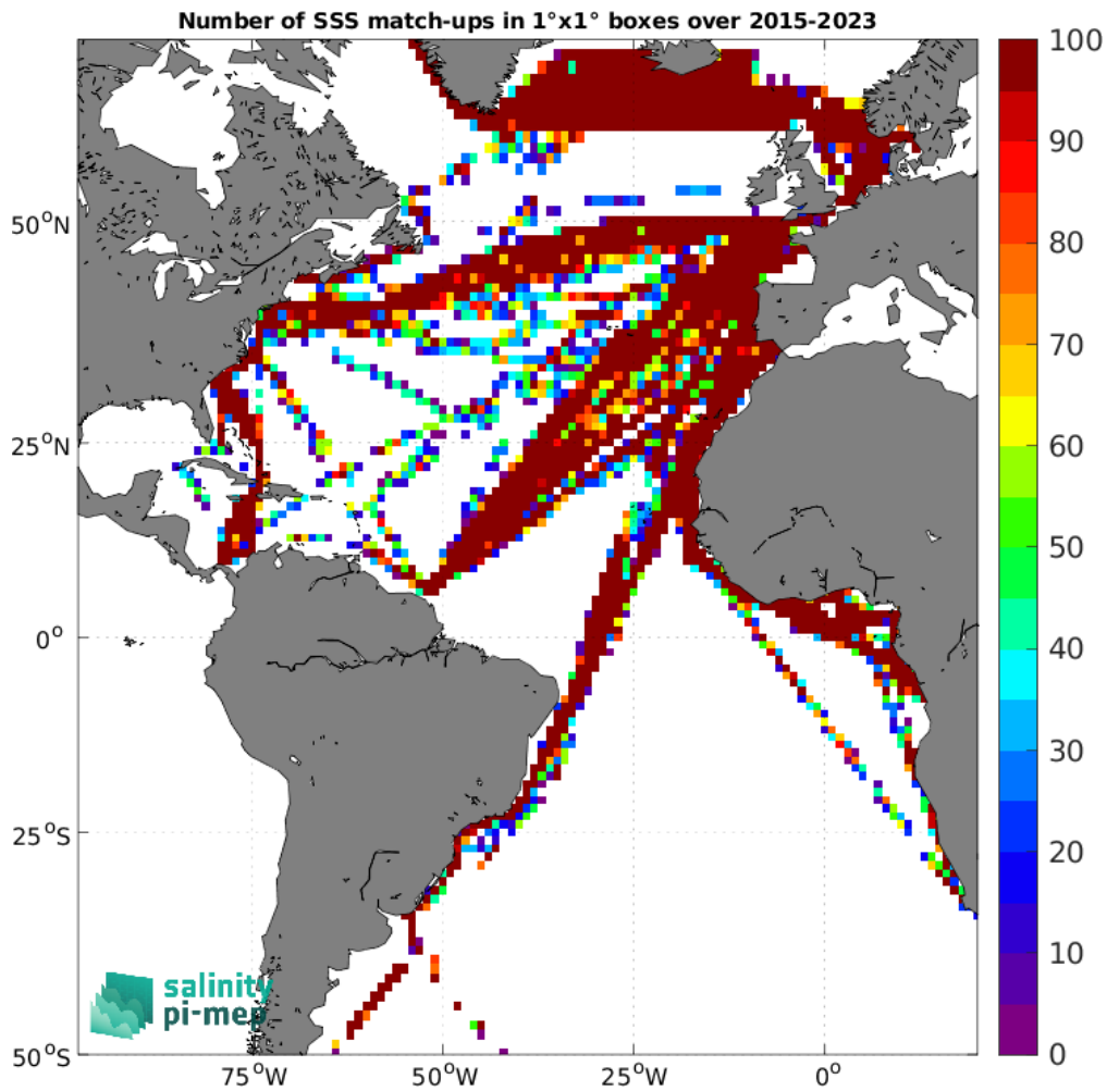
Figure 4: Number of SSS match-ups between TSG (LEGOS-DM) SSS and the SMAP SSS L2 v5 - 40 km (RSS) SSS product for the Atlantic Ocean Pi-MEP region over 1^\circ \times 1^\circ boxes and for the full satellite product period.
