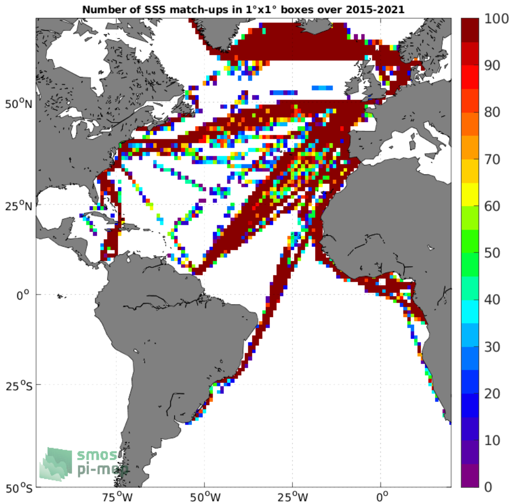
Figure 4: Number of SSS match-ups between TSG (LEGOS-DM) SSS and the SMAP SSS L2 v5 - 40 km (RSS) SSS product for the Atlantic Ocean Pi-MEP region over 1°x1° boxes and for the full satellite product period.
