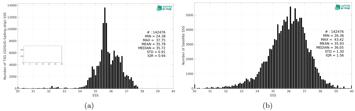
Figure 2: Histograms of SSS from TSG (GOSUD-Sailing-ship) (a) and SMAP SSS L2 v5 - 40 km (RSS) (b) considering all match-up pairs per bins of 0.1 over the Atlantic Ocean Pi-MEP region and for the full satellite product period.
