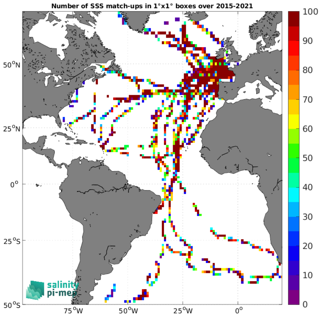
Figure 4: Number of SSS match-ups between TSG (GOSUD-Sailing-ship) SSS and the SMAP SSS L2 v5 - 40 km (RSS) SSS product for the Atlantic Ocean Pi-MEP region over 1°×1° boxes and for the full satellite product period.
