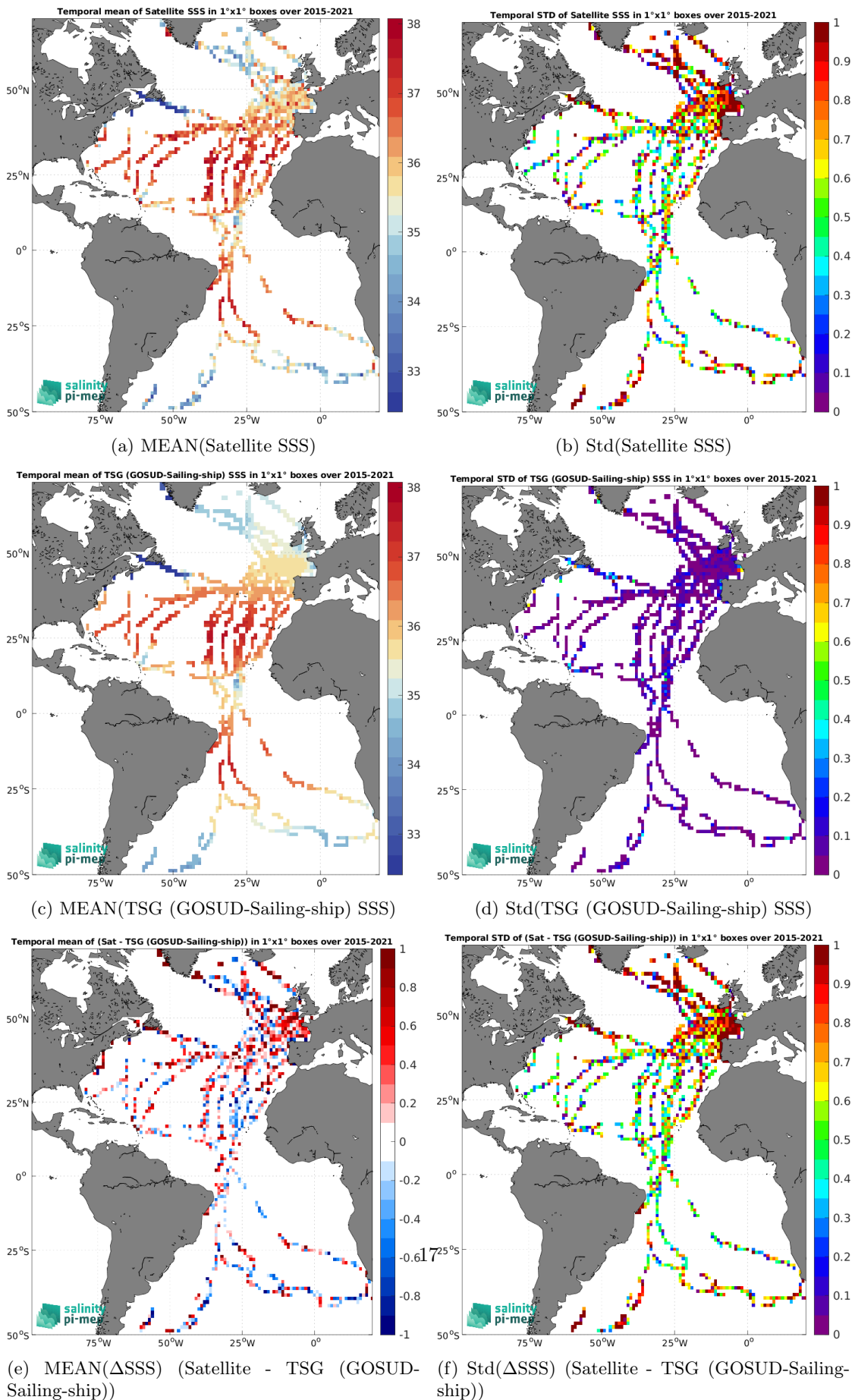
Figure 6: Temporal mean (left) and Std (right) of SSS from SMAP SSS L2 v5 - 40 km (RSS) (top), TSG (GOSUD-Sailing-ship) (middle), and of \Delta SSS (Satellite - TSG (GOSUD-Sailing-ship)). Only match-up pairs are used to generate these maps.
