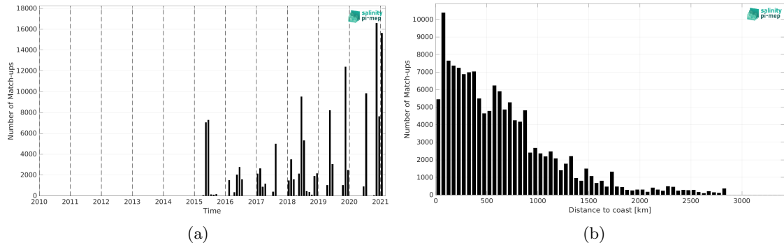
Figure 1: Number of match-ups between TSG (GOSUD-Sailing-ship) and SMAP SSS L2 v5 - 40 km (RSS) SSS as a function of time (a) and as function of the distance to coast (b) over the Atlantic Ocean Pi-MEP region and for the full satellite product period.
