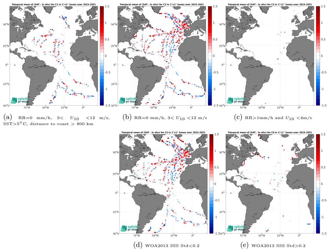
Figure 12: Temporal mean gridded over spatial boxes of size 1^\circ \times 1^\circ of \Delta\text{SSS} (SMAP SSS L2 v5 - 40 km (RSS) - TSG (GOSUD-Sailing-ship)) for 5 different subdatasets corresponding to:RR=0 mm/h, 3 < U_{10} < 12 m/s, SST>5°C, distance to coast > 800 km (a), RR=0 mm/h, 3 < U_{10} < 12 m/s (b), RR>1mm/h and U_{10} < 4 m/s (c), WOA2013 SSS Std<0.2 (d), WOA2013 SSS Std>0.2 (e).
