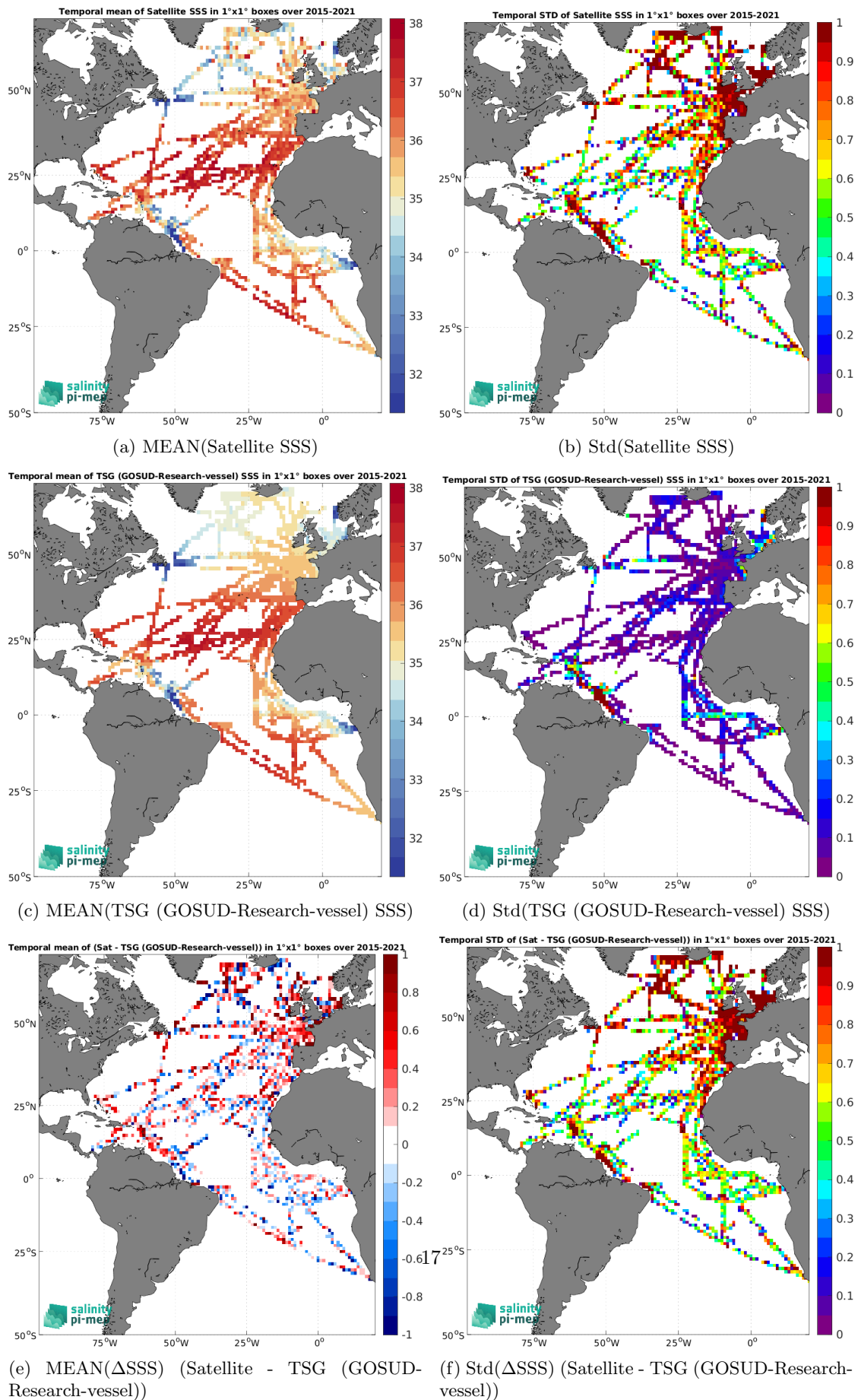
Figure 6: Temporal mean (left) and Std (right) of SSS from SMAP SSS L2 v5 - 40 km (RSS) (top), TSG (GOSUD-Research-vessel) (middle), and of \Delta SSS (Satellite - TSG (GOSUD-Research-vessel)). Only match-up pairs are used to generate these maps.
