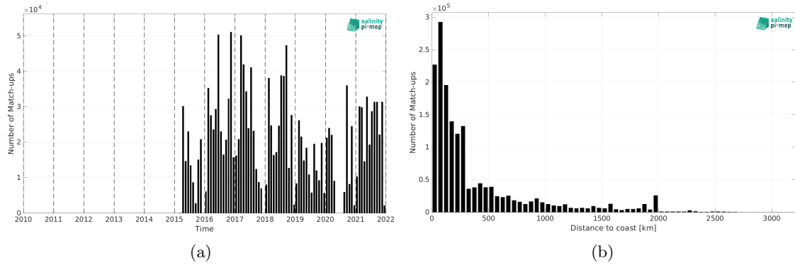
Figure 1: Number of match-ups between TSG (GOSUD-Research-vessel) and SMAP SSS L2 v5 - 40 km (RSS) SSS as a function of time (a) and as function of the distance to coast (b) over the Atlantic Ocean Pi-MEP region and for the full satellite product period.
