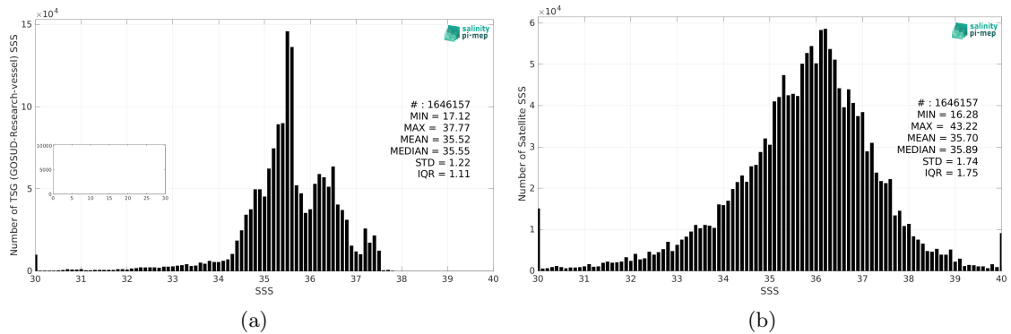
Figure 2: Histograms of SSS from TSG (GOSUD-Research-vessel) (a) and SMAP SSS L2 v5 - 40 km (RSS) (b) considering all match-up pairs per bins of 0.1 over the Atlantic Ocean Pi-MEP region and for the full satellite product period.
