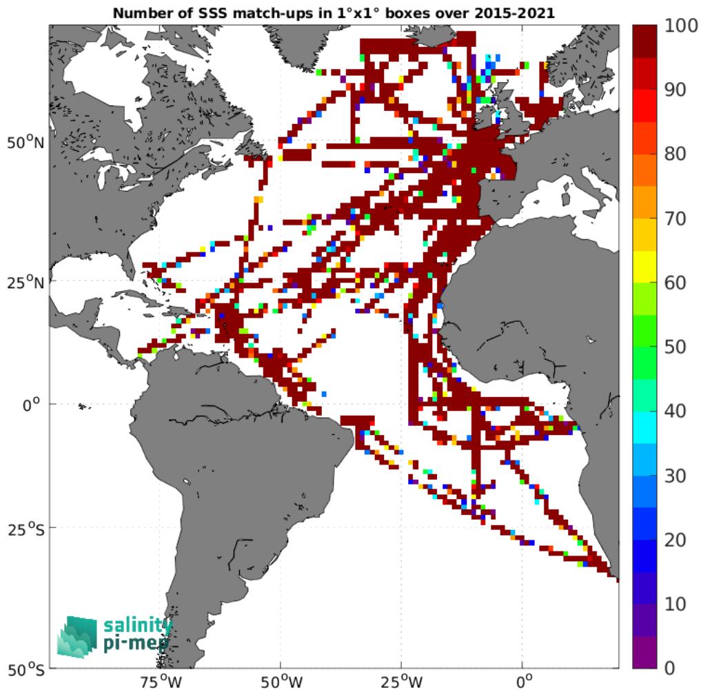
Figure 4: Number of SSS match-ups between TSG (GOSUD-Research-vessel) SSS and the SMAP SSS L2 v5 - 40 km (RSS) SSS product for the Atlantic Ocean Pi-MEP region over 1^\circ \times 1^\circ boxes and for the full satellite product period.
