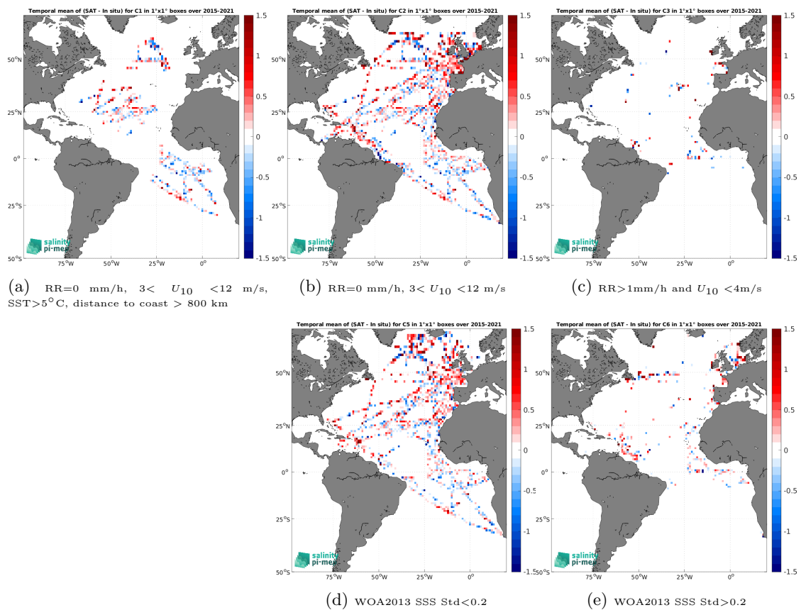
Figure 12: Temporal mean gridded over spatial boxes of size 1^\circ \times 1^\circ of \Delta\text{SSS} (SMAP SSS L2 v5 - 40 km (RSS) - TSG (GOSUD-Research-vessel)) for 5 different subdatasets corresponding to:RR=0 mm/h, 3 < U_{10} < 12 m/s, SST>5°C, distance to coast > 800 km (a), RR=0 mm/h, 3 < U_{10} < 12 m/s (b), RR>1mm/h and U_{10} < 4 m/s (c), WOA2013 SSS Std<0.2 (d), WOA2013 SSS Std>0.2 (e).
