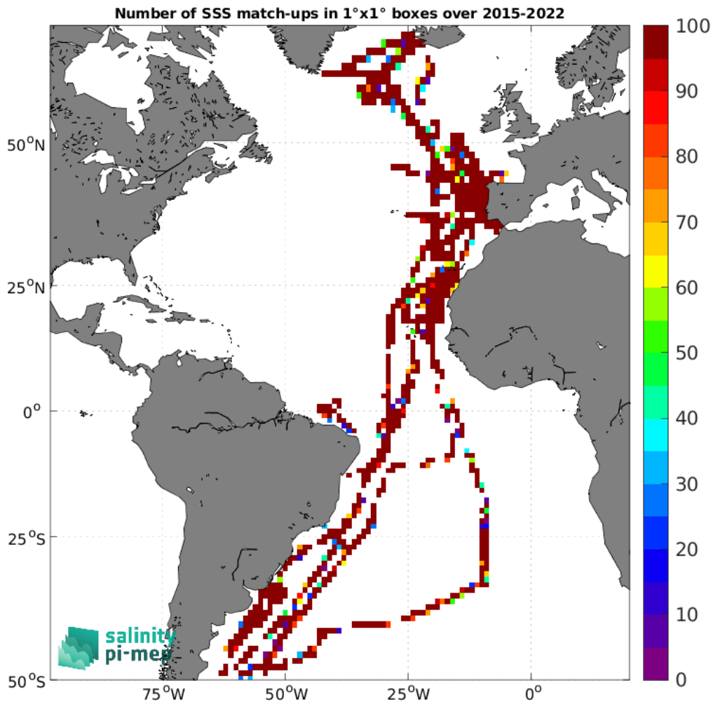
Figure 4: Number of SSS match-ups between TSG (CSIC-UTM) SSS and the SMAP SSS L2 v5 - 40 km (RSS) SSS product for the Atlantic Ocean Pi-MEP region over 1^{\circ} \times 1^{\circ} boxes and for the full satellite product period.
