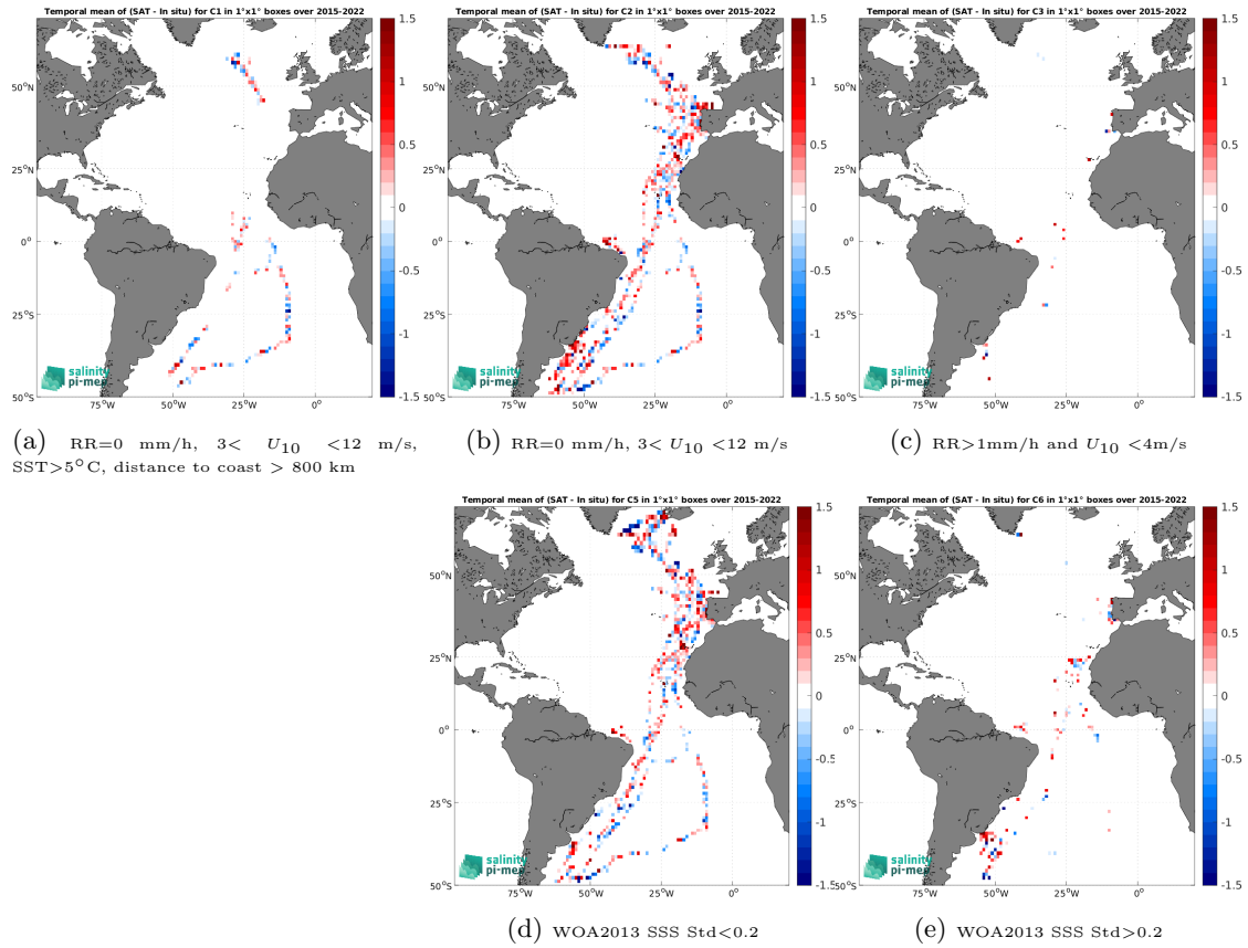
Figure 12: Temporal mean gridded over spatial boxes of size 1^\circ \times 1^\circ of \Delta SSS (SMAP SSS L2 v5 - 40 km (RSS) - TSG (CSIC-UTM)) for 5 different subdatasets corresponding to:RR=0 mm/h, 3 < U_{10} < 12 m/s, SST >5^\circ\text{C} , distance to coast > 800 km (a), RR=0 mm/h, 3 < U_{10} < 12 m/s (b), RR >1 mm/h and U_{10} < 4 m/s (c), WOA2013 SSS Std <0.2 (d), WOA2013 SSS Std >0.2 (e).
