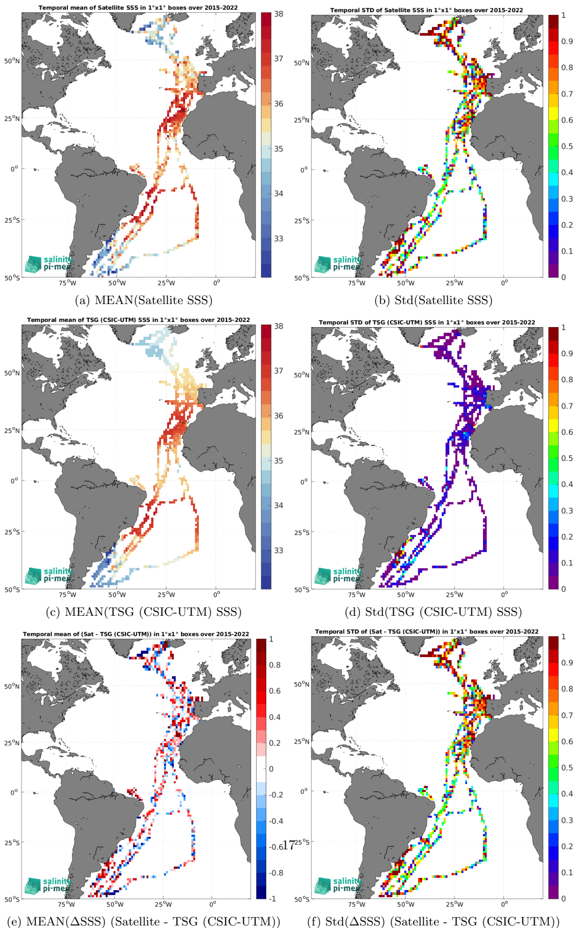
Figure 6: Temporal mean (left) and Std (right) of SSS from SMAP SSS L2 v5 - 40 km (RSS) (top), TSG (CSIC-UTM) (middle), and of \Delta SSS (Satellite - TSG (CSIC-UTM)). Only match-up pairs are used to generate these maps.
