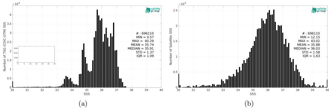
Figure 2: Histograms of SSS from TSG (CSIC-UTM) (a) and SMAP SSS L2 v5 - 40 km (RSS) (b) considering all match-up pairs per bins of 0.1 over the Atlantic Ocean Pi-MEP region and for the full satellite product period.
