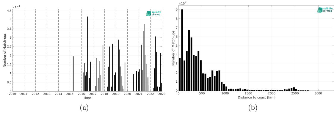
Figure 1: Number of match-ups between TSG (CSIC-UTM) and SMAP SSS L2 v5 - 40 km (RSS) SSS as a function of time (a) and as function of the distance to coast (b) over the Atlantic Ocean Pi-MEP region and for the full satellite product period.
