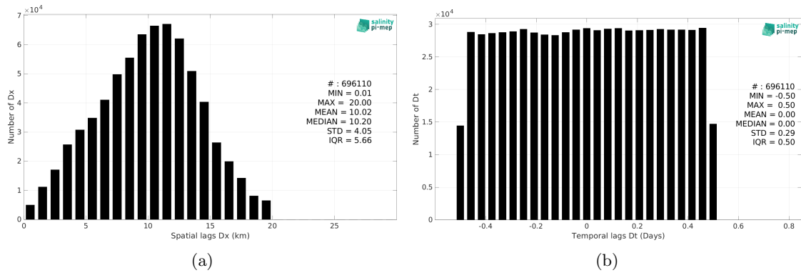
Figure 5: Histograms of the spatial (a) and temporal (b) lags between the location/time of the TSG (CSIC-UTM) measurement and the date of the corresponding SMAP SSS L2 v5 - 40 km (RSS) SSS pixel.
