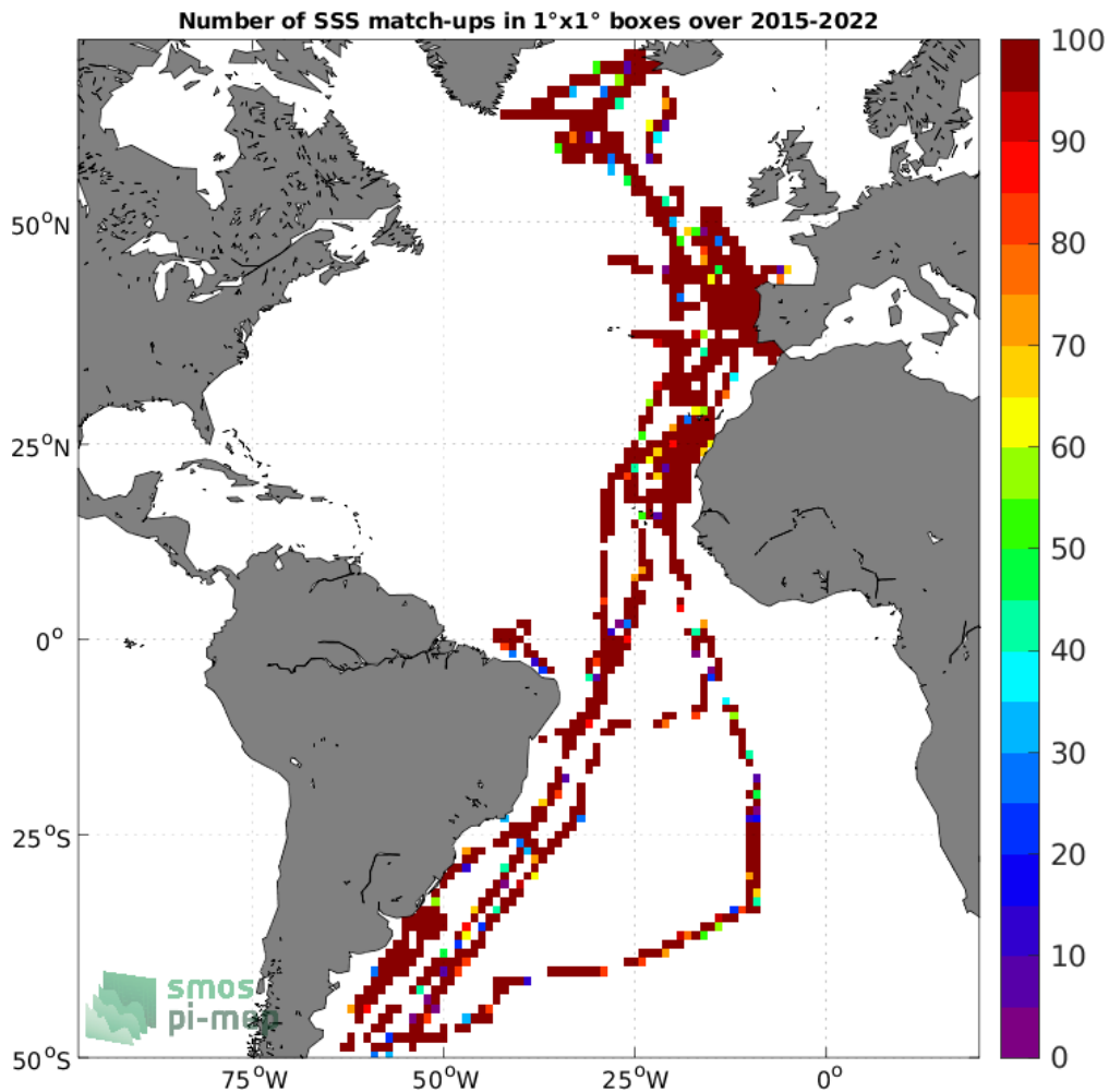
Figure 4: Number of SSS match-ups between TSG (CSIC-UTM) SSS and the SMAP SSS L2 v5 - 40 km (RSS) SSS product for the Atlantic Ocean Pi-MEP region over 1°×1° boxes and for the full satellite product period.
