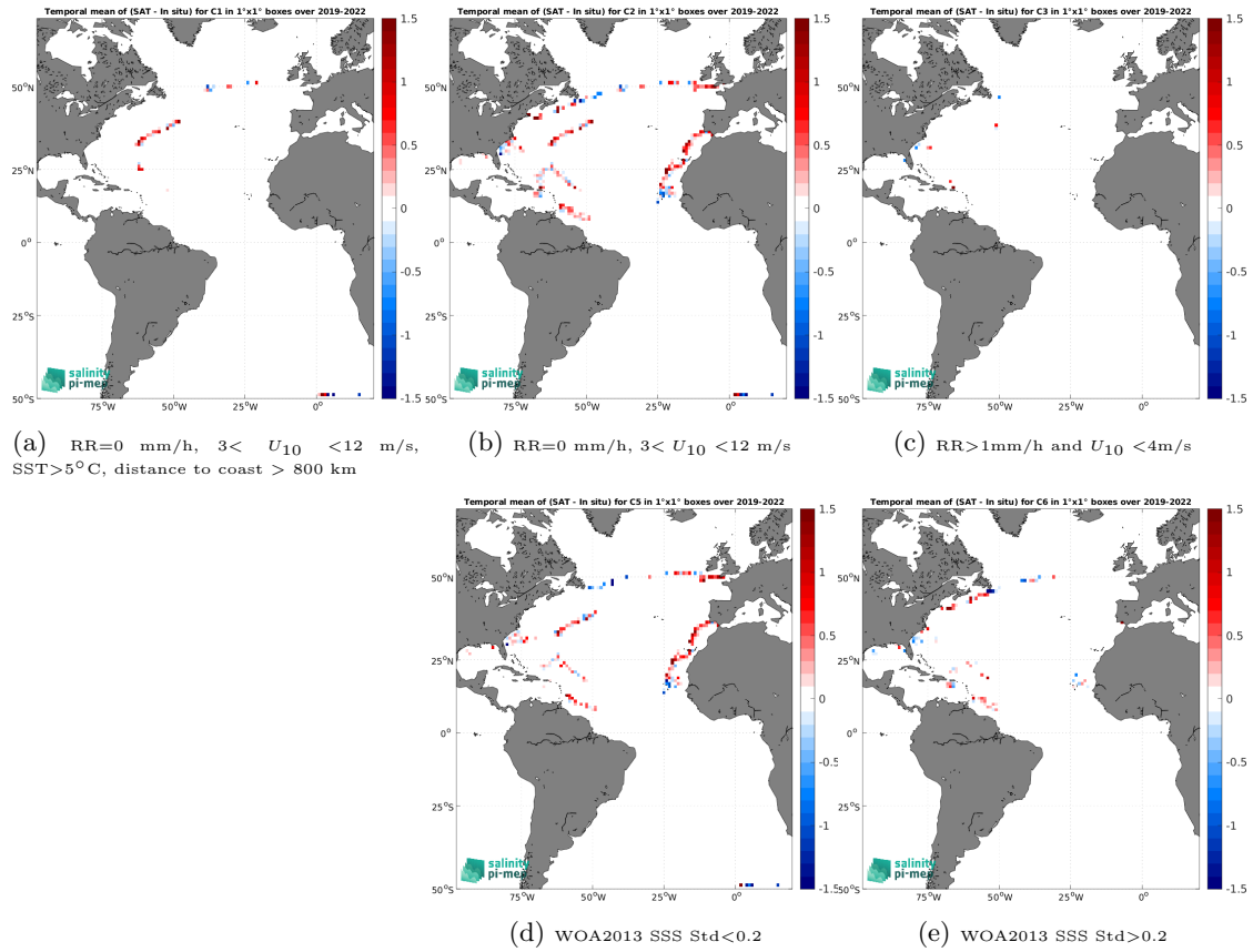
Figure 12: Temporal mean gridded over spatial boxes of size 1^\circ \times 1^\circ of \Delta SSS (SMAP SSS L2 v5 - 40 km (RSS) - Saldron) for 5 different subdatasets corresponding to:RR=0 mm/h, 3 < U_{10} < 12 m/s, SST >5^\circ\text{C} , distance to coast > 800 km (a), RR=0 mm/h, 3 < U_{10} < 12 m/s (b), RR >1 mm/h and U_{10} < 4 m/s (c), WOA2013 SSS Std <0.2 (d), WOA2013 SSS Std >0.2 (e).
