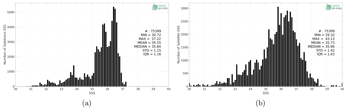
Figure 2: Histograms of SSS from Saildrone (a) and SMAP SSS L2 v5 - 40 km (RSS) (b) considering all match-up pairs per bins of 0.1 over the Atlantic Ocean Pi-MEP region and for the full satellite product period.
