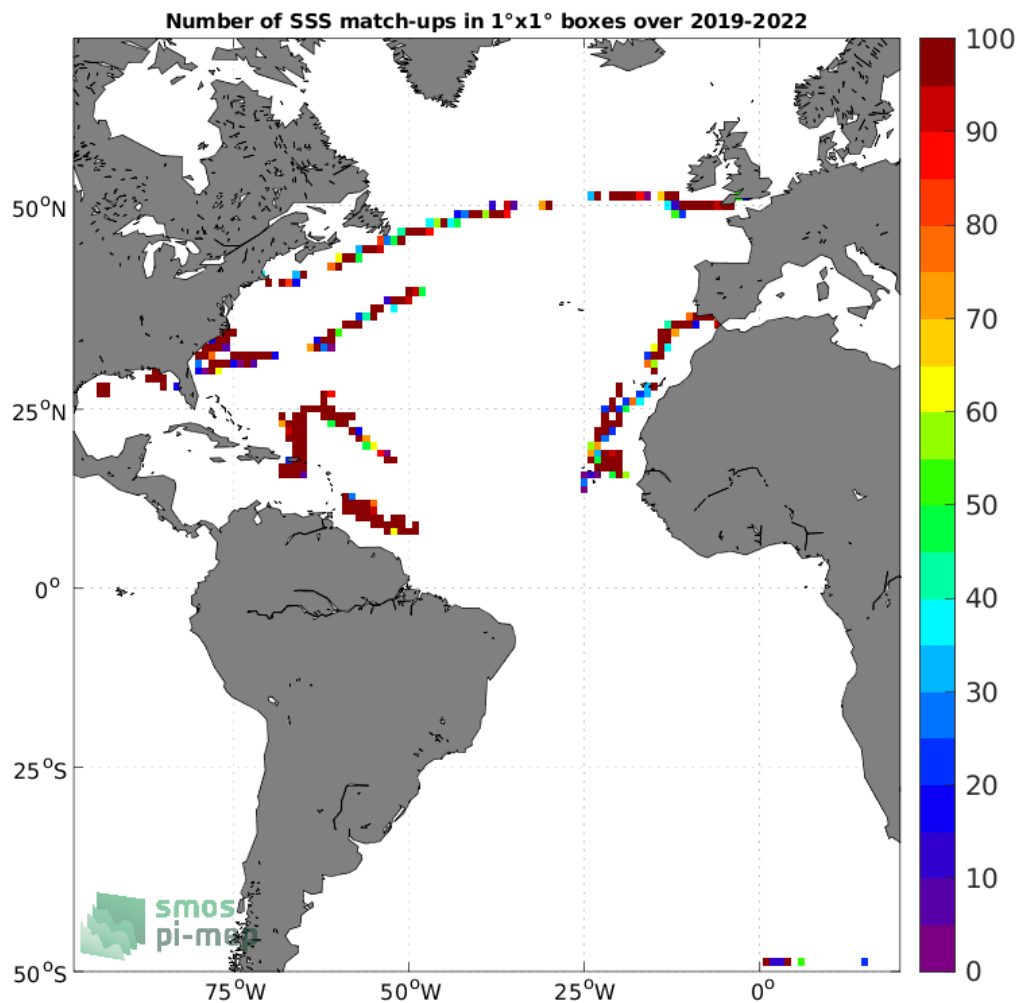
Figure 4: Number of SSS match-ups between Saildrone SSS and the SMAP SSS L2 v5 - 40 km (RSS) SSS product for the Atlantic Ocean Pi-MEP region over 1°x1° boxes and for the full satellite product period.
