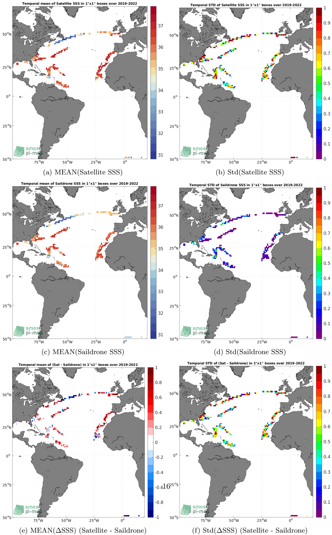
Figure 6: Temporal mean (left) and Std (right) of SSS from SMAP SSS L2 v5 - 40 km (RSS) (top), Saildrone (middle), and of \Delta SSS (Satellite - Saildrone). Only match-up pairs are used to generate these maps.
