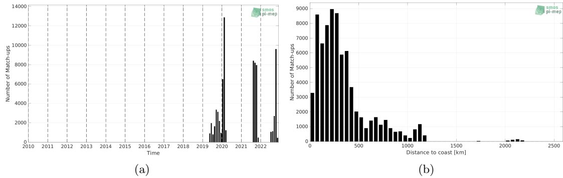
Figure 1: Number of match-ups between Saildrone and SMAP SSS L2 v5 - 40 km (RSS) SSS as a function of time (a) and as function of the distance to coast (b) over the Atlantic Ocean Pi-MEP region and for the full satellite product period.
