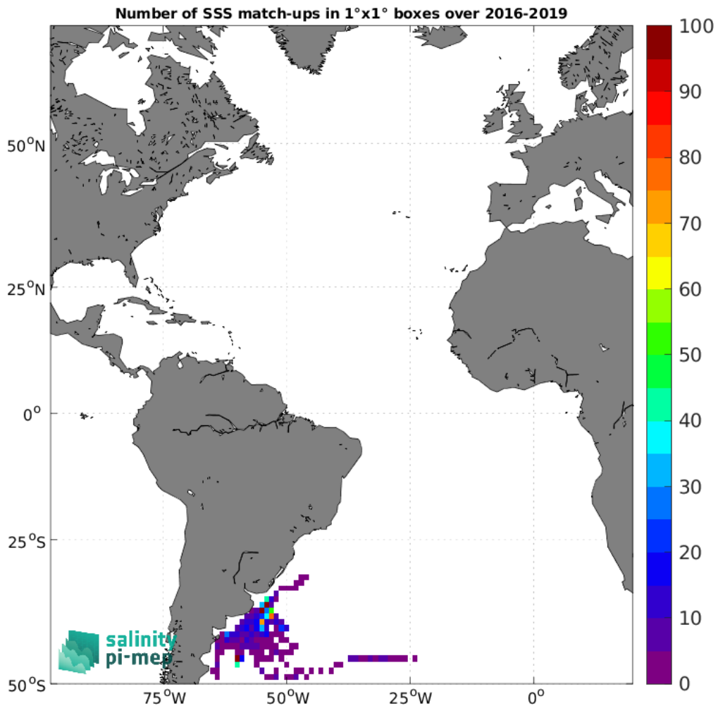
Figure 4: Number of SSS match-ups between Marine mammals SSS and the SMAP SSS L2 v5 - 40 km (RSS) SSS product for the Atlantic Ocean Pi-MEP region over 1°×1° boxes and for the full satellite product period.
