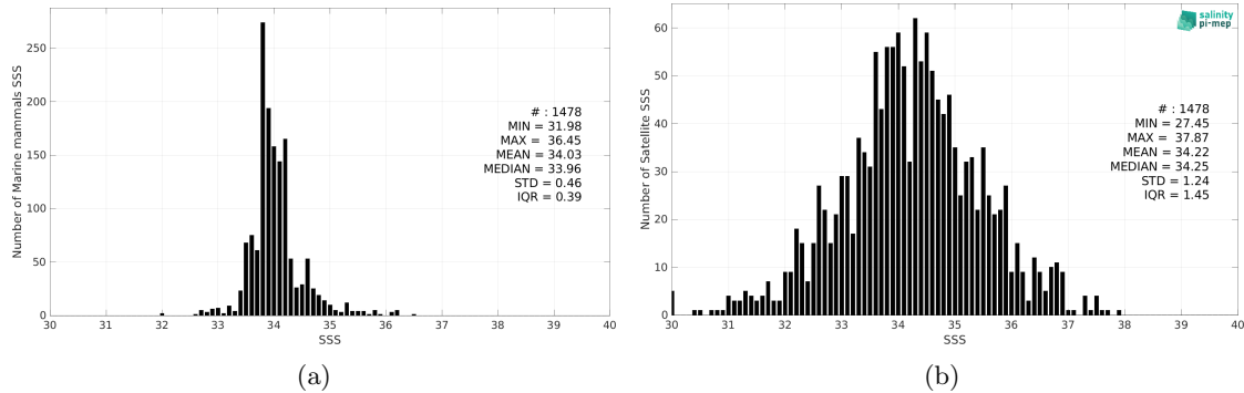
Figure 2: Histograms of SSS from Marine mammals (a) and SMAP SSS L2 v5 - 40 km (RSS) (b) considering all match-up pairs per bins of 0.1 over the Atlantic Ocean Pi-MEP region and for the full satellite product period.
