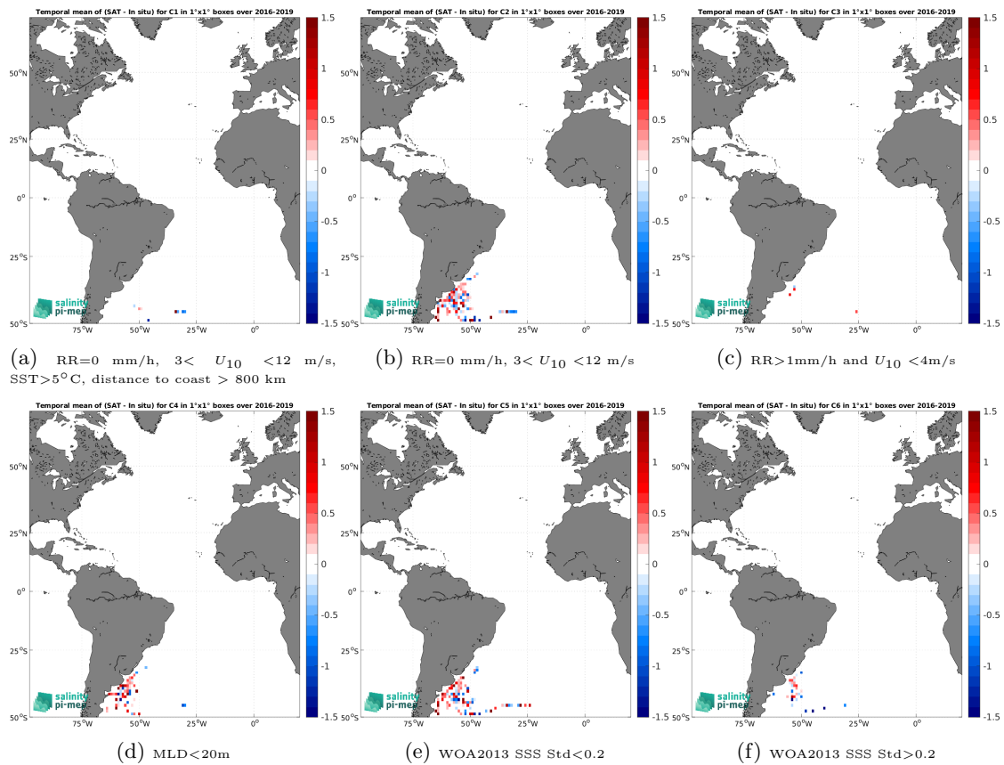
Figure 12: Temporal mean gridded over spatial boxes of size 1^\circ \times 1^\circ of \Delta SSS (SMAP SSS L2 v5 - 40 km (RSS) - Marine mammals) for 6 different subdatasets corresponding to:RR=0 mm/h, 3 < U_{10} < 12 m/s, SST >5^\circ C, distance to coast > 800 km (a), RR=0 mm/h, 3 < U_{10} < 12 m/s (b), RR >1 mm/h and U_{10} < 4 m/s (c),MLD <20 m (d),WOA2013 SSS Std <0.2 (e),WOA2013 SSS Std >0.2 (f).
