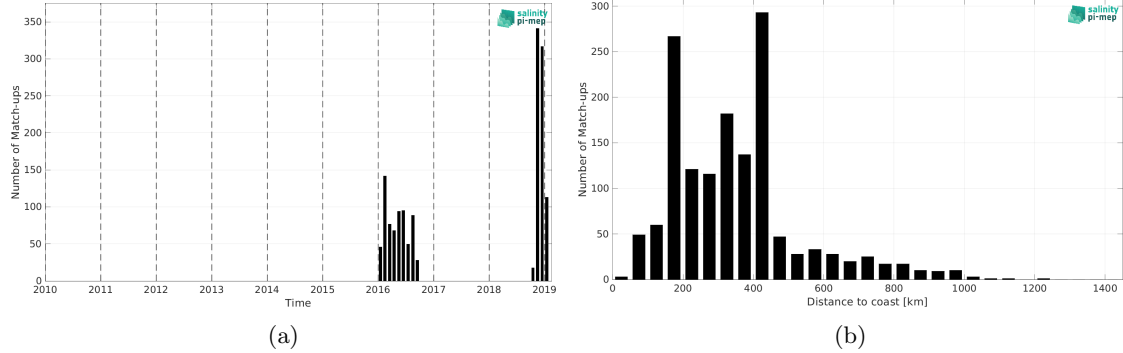
Figure 1: Number of match-ups between Marine mammals and SMAP SSS L2 v5 - 40 km (RSS) SSS as a function of time (a) and as function of the distance to coast (b) over the Atlantic Ocean Pi-MEP region and for the full satellite product period.
