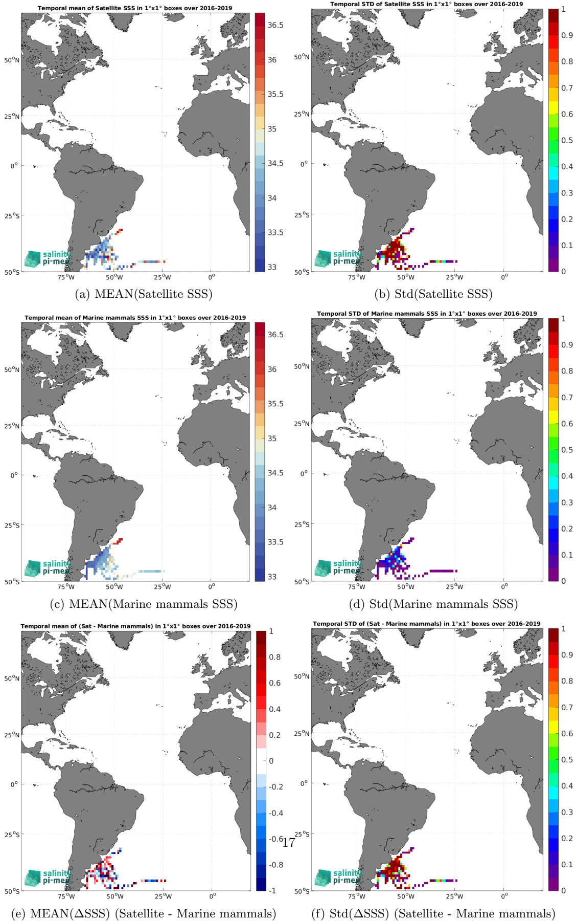
Figure 6: Temporal mean (left) and Std (right) of SSS from SMAP SSS L2 v5 - 40 km (RSS) (top), Marine mammals (middle), and of \Delta SSS (Satellite - Marine mammals). Only match-up pairs are used to generate these maps.
