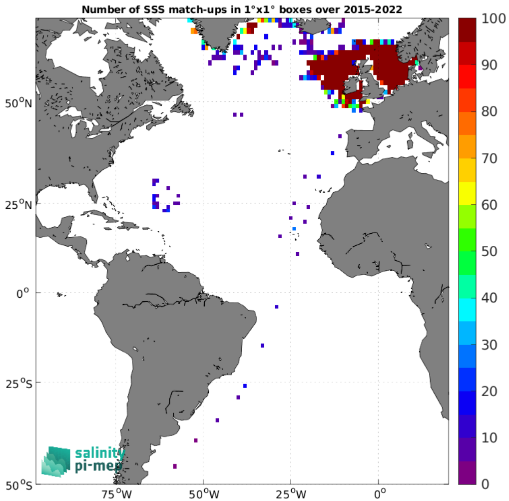
Figure 4: Number of SSS match-ups between ICES SSS and the SMAP SSS L2 v5 - 40 km (RSS) SSS product for the Atlantic Ocean Pi-MEP region over 1^\circ \times 1^\circ boxes and for the full satellite product period.
