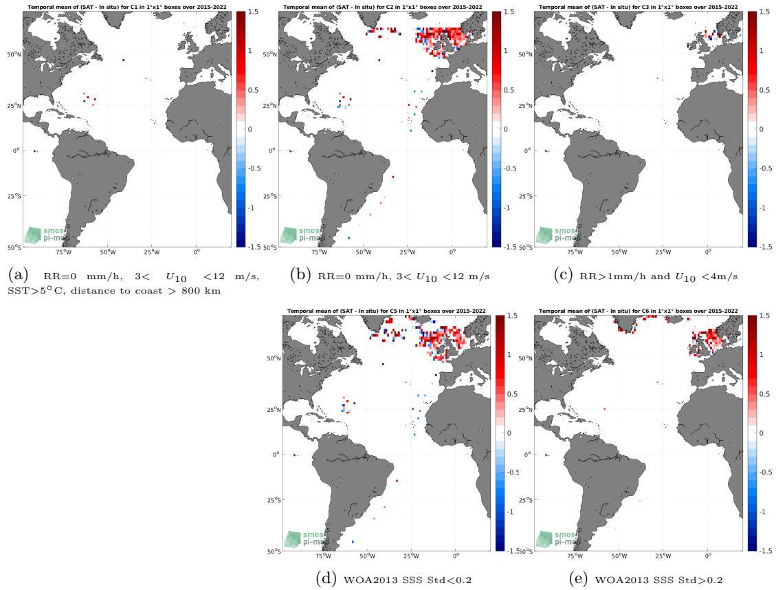
Figure 12: Temporal mean gridded over spatial boxes of size 1^\circ \times 1^\circ of \Delta SSS (SMAP SSS L2 v5 - 40 km (RSS) - ICES) for 5 different subdatasets corresponding to:RR=0 mm/h, 3 < U_{10} < 12 m/s, SST >5^\circ\text{C} , distance to coast > 800 km (a), RR=0 mm/h, 3 < U_{10} < 12 m/s (b), RR >1 mm/h and U_{10} < 4 m/s (c), WOA2013 SSS Std <0.2 (d), WOA2013 SSS Std >0.2 (e).
