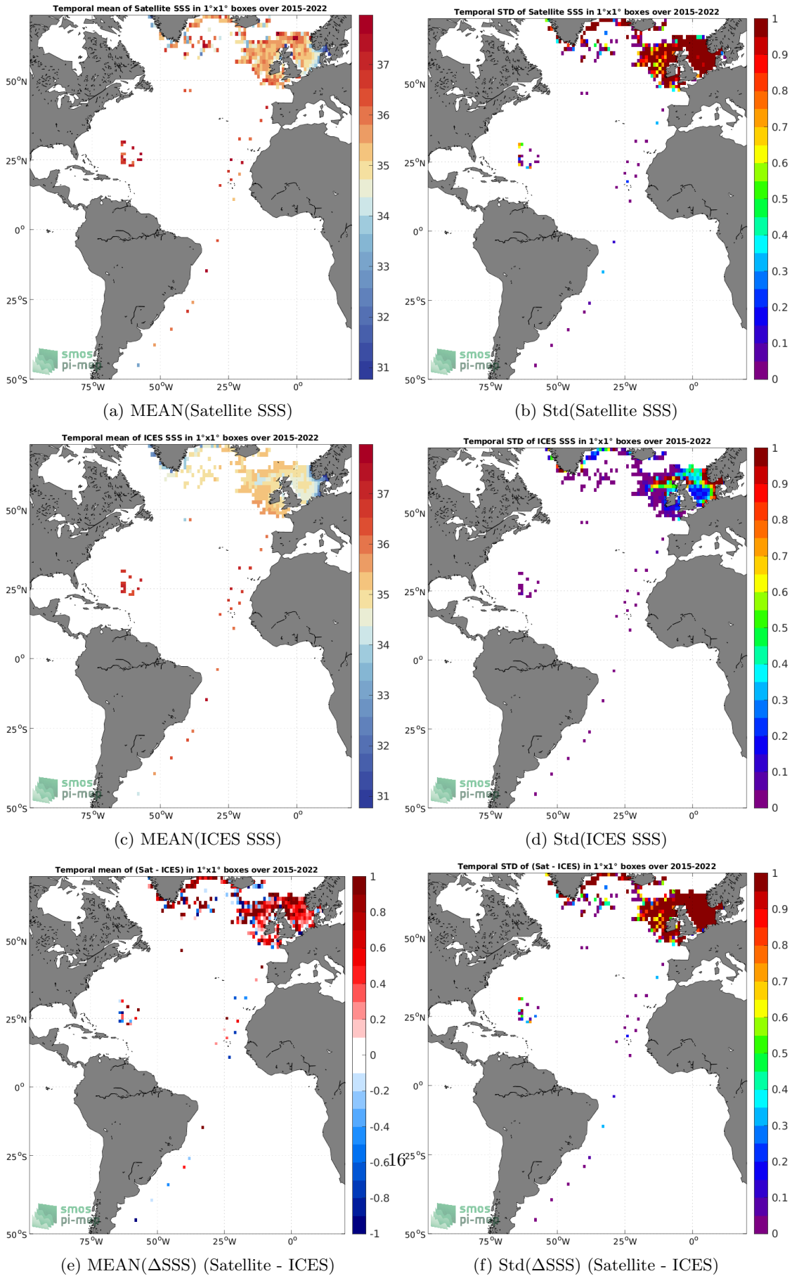
Figure 6: Temporal mean (left) and Std (right) of SSS from SMAP SSS L2 v5 - 40 km (RSS) (top), ICES (middle), and of \Delta SSS (Satellite - ICES). Only match-up pairs are used to generate these maps.
