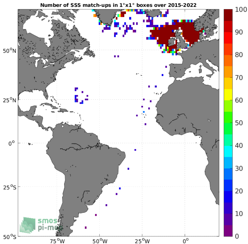
Figure 4: Number of SSS match-ups between ICES SSS and the SMAP SSS L2 v5 - 40 km (RSS) SSS product for the Atlantic Ocean Pi-MEP region over 1°×1° boxes and for the full satellite product period.
