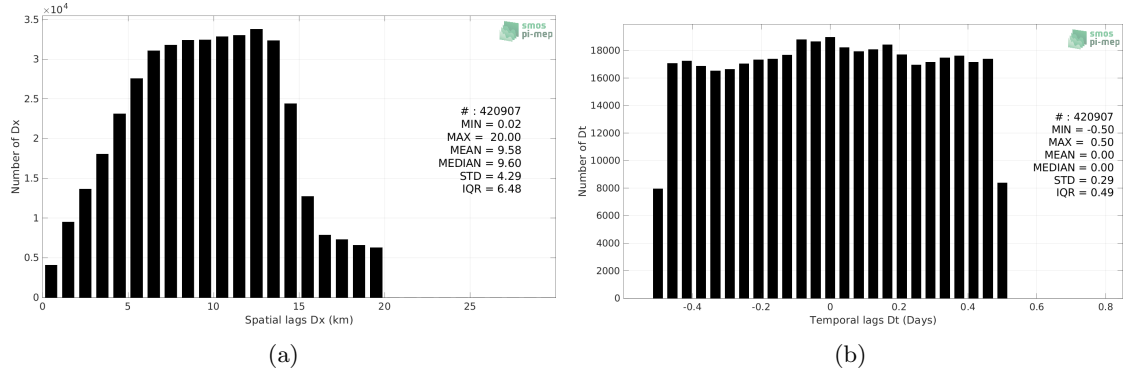
Figure 5: Histograms of the spatial (a) and temporal (b) lags between the location/time of the ICES measurement and the date of the corresponding SMAP SSS L2 v5 - 40 km (RSS) SSS pixel.
