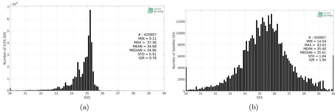
Figure 2: Histograms of SSS from ICES (a) and SMAP SSS L2 v5 - 40 km (RSS) (b) considering all match-up pairs per bins of 0.1 over the Atlantic Ocean Pi-MEP region and for the full satellite product period.
