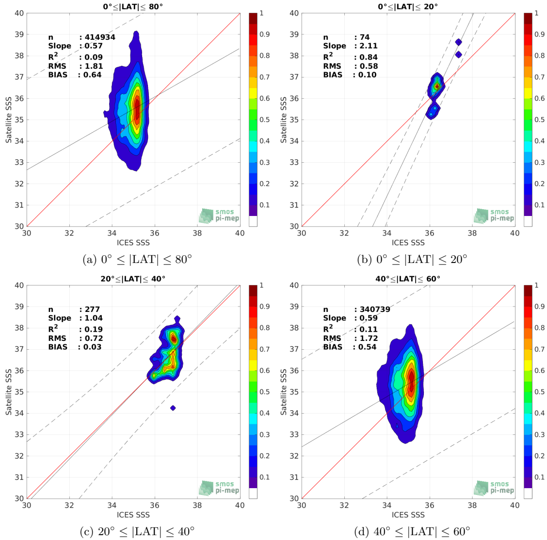
Figure 9: Contour maps of the concentration of SMAP SSS L2 v5 - 40 km (RSS) SSS (y-axis) versus ICES SSS (x-axis) at match-up pairs for different latitude bands. For each plot, the red line shows x=y . The black thin and dashed lines indicate a linear fit through the data cloud and the \pm 95\% confidence levels, respectively. The number match-up pairs n , the slope and R^2 coefficient of the linear fit, the root mean square (RMS) and the mean bias between satellite and in situ data are indicated for each latitude band in each plots.
