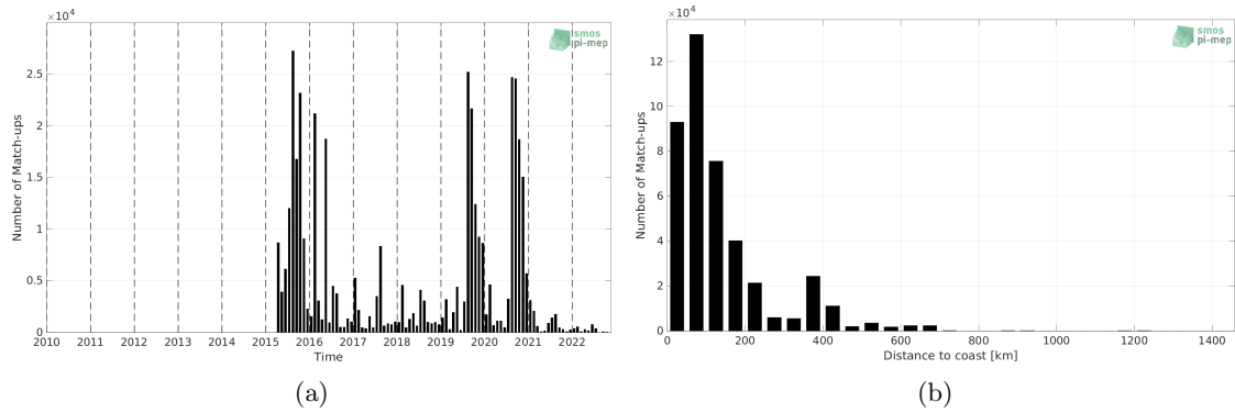
Figure 1: Number of match-ups between ICES and SMAP SSS L2 v5 - 40 km (RSS) SSS as a function of time (a) and as function of the distance to coast (b) over the Atlantic Ocean Pi-MEP region and for the full satellite product period.
