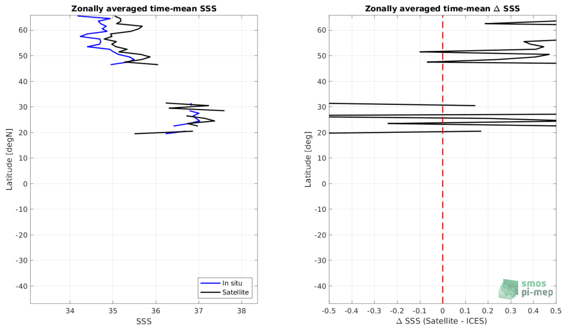
Figure 8: Left panel: Zonal mean SSS from SMAP SSS L2 v5 - 40 km (RSS) satellite product (black) and from ICES (blue). Right panel: Zonal mean of \Delta SSS (Satellite - ICES) for all the collected Pi-MEP match-up pairs estimated over the full satellite product period.
