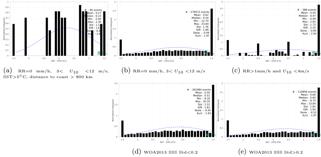
Figure 13: Normalized histogram of \Delta SSS (SMAP SSS L2 v5 - 40 km (RSS) - ICES) for 5 different subdatasets corresponding to: RR=0 mm/h, 3 < U_{10} < 12 m/s, SST > 5°C, distance to coast > 800 km (a), RR=0 mm/h, 3 < U_{10} < 12 m/s (b), RR > 1mm/h and U_{10} < 4 m/s (c), WOA2013 SSS Std < 0.2 (d), WOA2013 SSS Std > 0.2 (e).
