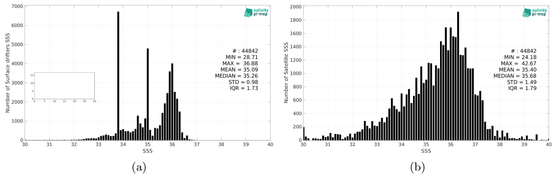
Figure 2: Histograms of SSS from Surface drifters (a) and SMAP SSS L2 v5 - 40 km (RSS) (b) considering all match-up pairs per bins of 0.1 over the Atlantic Ocean Pi-MEP region and for the full satellite product period.
