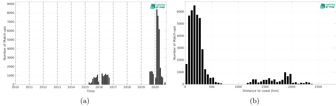
Figure 1: Number of match-ups between Surface drifters and SMAP SSS L2 v5 - 40 km (RSS) SSS as a function of time (a) and as function of the distance to coast (b) over the Atlantic Ocean Pi-MEP region and for the full satellite product period.
