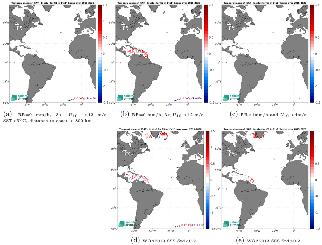
Figure 11: Temporal mean gridded over spatial boxes of size 1^\circ \times 1^\circ of \Delta SSS (SMAP SSS L2 v5 - 40 km (RSS) - Surface drifters) for 5 different subdatasets corresponding to:RR=0 mm/h, 3 < U_{10} < 12 m/s, SST >5^\circ\text{C} , distance to coast > 800 km (a), RR=0 mm/h, 3 < U_{10} < 12 m/s (b), RR >1 mm/h and U_{10} < 4 m/s (c), WOA2013 SSS Std <0.2 (d), WOA2013 SSS Std >0.2 (e).
