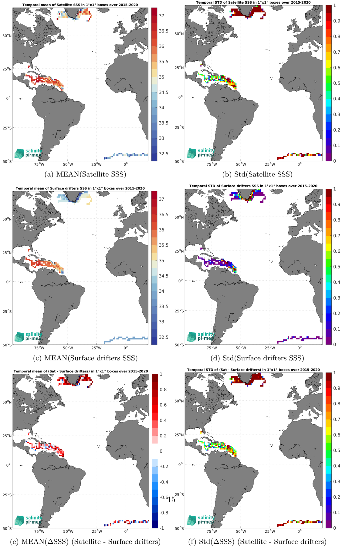
(e) MEAN( \Delta SSS) (Satellite - Surface drifters) (f) Std( \Delta SSS) (Satellite - Surface drifters) Figure 5: Temporal mean (left) and Std (right) of SSS from SMAP SSS L2 v5 - 40 km (RSS) (top), Surface drifters (middle), and of \Delta SSS (Satellite - Surface drifters). Only match-up pairs are used to generate these maps.
