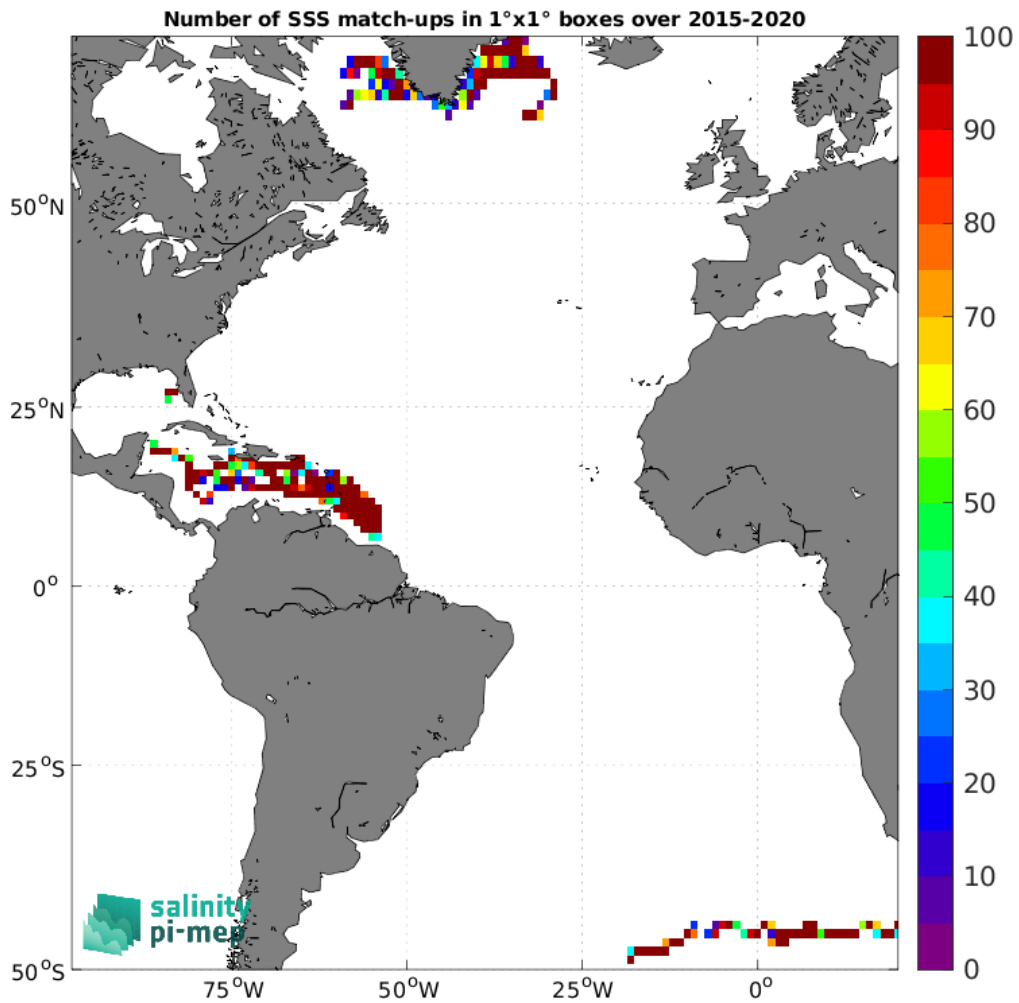
Figure 3: Number of SSS match-ups between Surface drifters SSS and the SMAP SSS L2 v5 - 40 km (RSS) SSS product for the Atlantic Ocean Pi-MEP region over 1°×1° boxes and for the full satellite product period.
