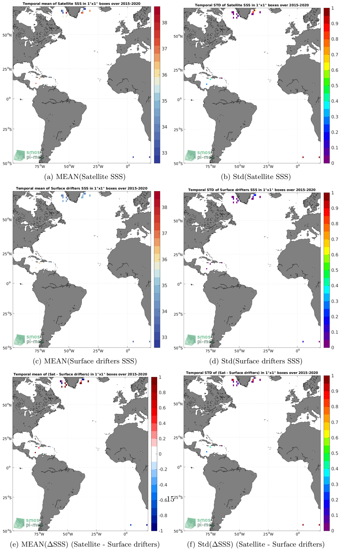
Figure 5: Temporal mean (left) and Std (right) of SSS from SMAP SSS L2 v5 - 40 km (RSS) (top), Surface drifters (middle), and of \Delta SSS (Satellite - Surface drifters). Only match-up pairs are used to generate these maps.
