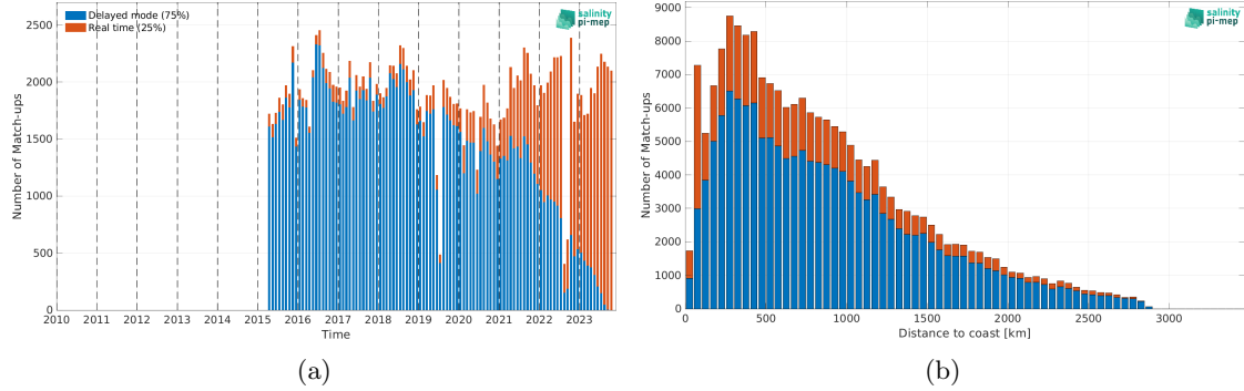
Figure 1: Number of match-ups between Argo and SMAP SSS L2 v5 - 40 km (RSS) SSS as a function of time (a) and as function of the distance to coast (b) over the Atlantic Ocean Pi-MEP region and for the full satellite product period.
