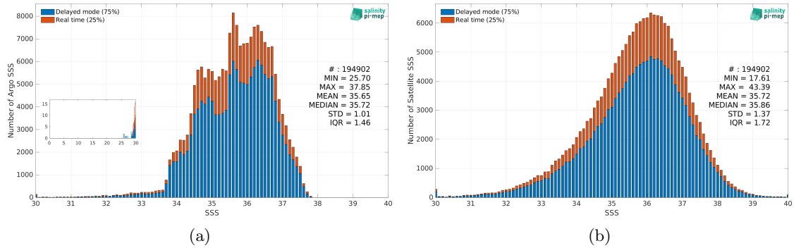
Figure 2: Histograms of SSS from Argo (a) and SMAP SSS L2 v5 - 40 km (RSS) (b) considering all match-up pairs per bins of 0.1 over the Atlantic Ocean Pi-MEP region and for the full satellite product period.
