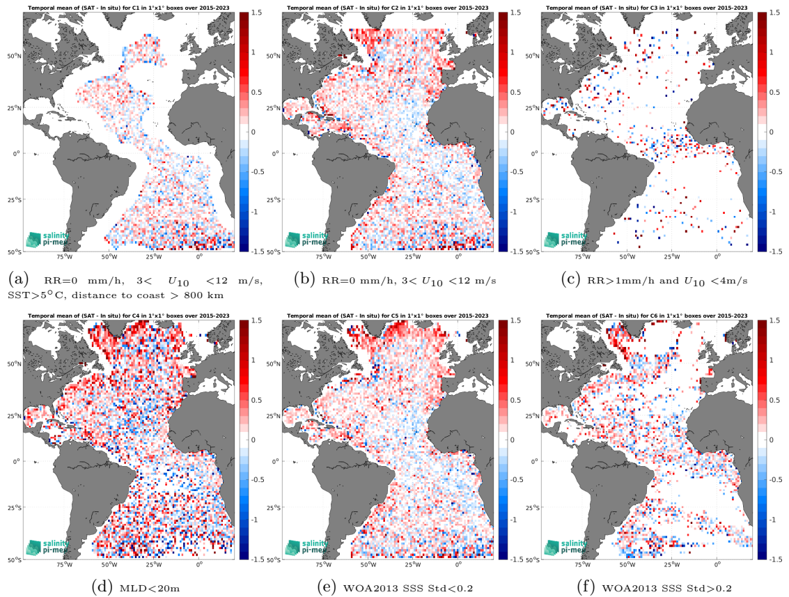
Figure 12: Temporal mean gridded over spatial boxes of size 1^\circ \times 1^\circ of \Delta SSS (SMAP SSS L2 v5 - 40 km (RSS) - Argo) for 6 different subdatasets corresponding to:RR=0 mm/h, 3 < U_{10} < 12 m/s, SST > 5^\circ\text{C} , distance to coast > 800 km (a), RR=0 mm/h, 3 < U_{10} < 12 m/s (b), RR > 1 mm/h and U_{10} < 4 m/s (c),MLD < 20 m (d),WOA2013 SSS Std < 0.2 (e),WOA2013 SSS Std > 0.2 (f).
