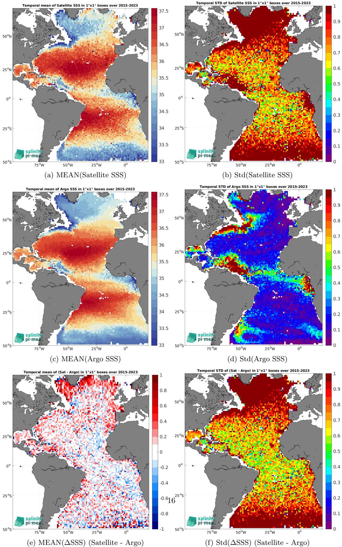
Figure 6: Temporal mean (left) and Std (right) of SSS from SMAP SSS L2 v5 - 40 km (RSS) (top), Argo (middle), and of \Delta SSS (Satellite - Argo). Only match-up pairs are used to generate these maps.
