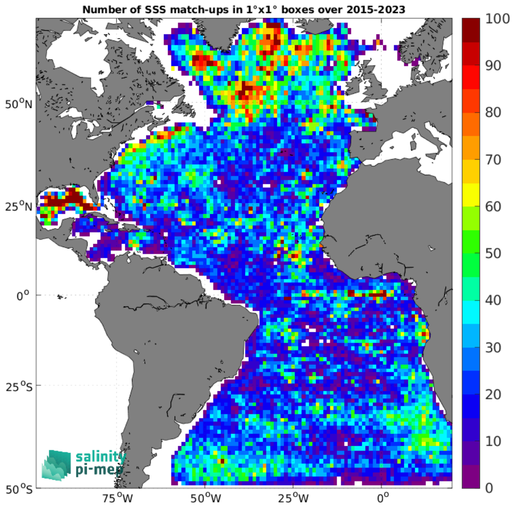
Figure 4: Number of SSS match-ups between Argo SSS and the SMAP SSS L2 v5 - 40 km (RSS) SSS product for the Atlantic Ocean Pi-MEP region over 1^\circ \times 1^\circ boxes and for the full satellite product period.
