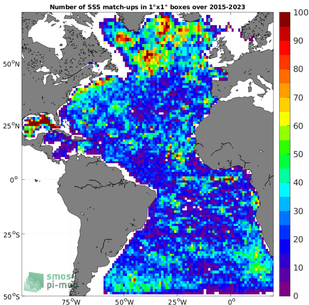
Figure 4: Number of SSS match-ups between Argo SSS and the SMAP SSS L2 v5 - 40 km (RSS) SSS product for the Atlantic Ocean Pi-MEP region over 1°×1° boxes and for the full satellite product period.
