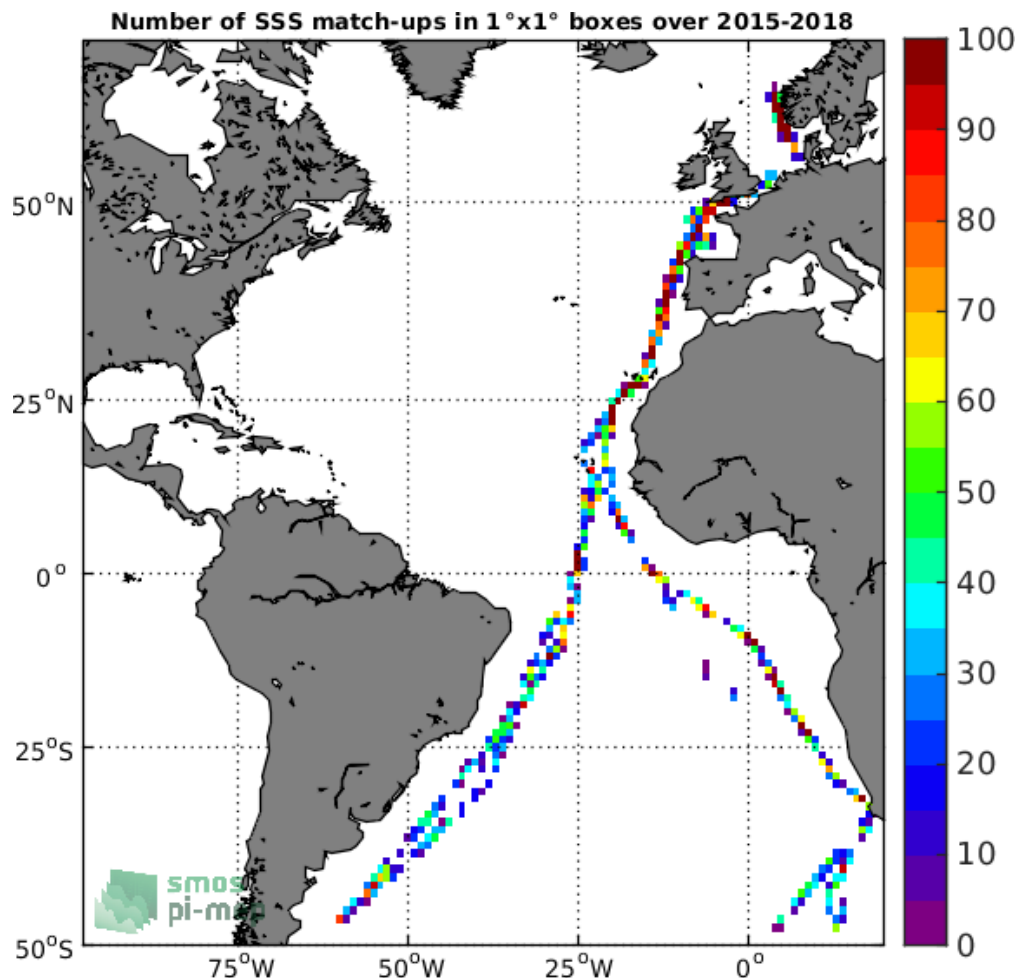
Figure 4: Number of SSS match-ups between TSG-POLARSTERN SSS and the SMAP-L2-RSS-V4 SSS product for the Atlantic Ocean Pi-MEP region over 1^\circ \times 1^\circ boxes and for the full satellite product period.
