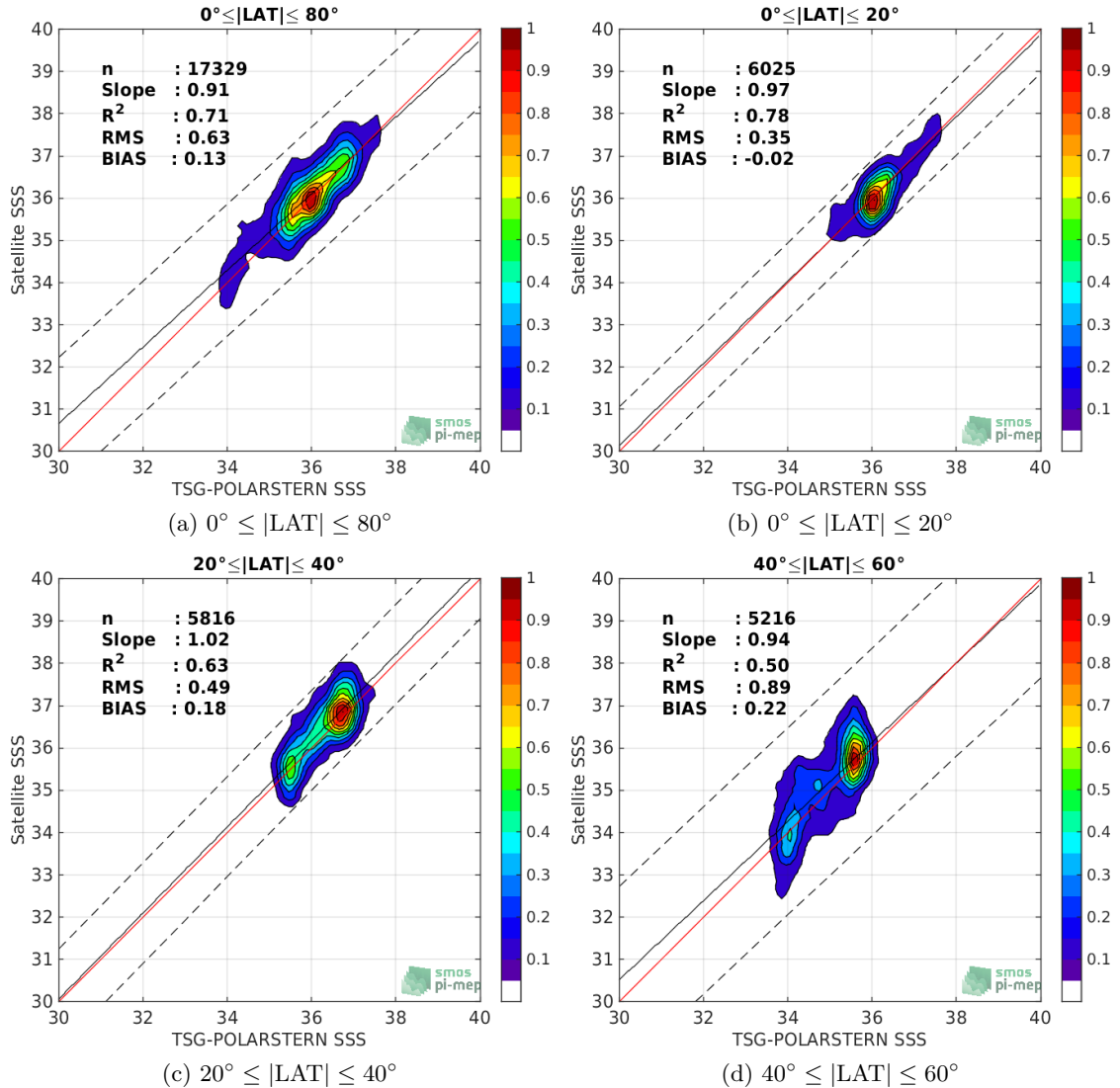
Figure 9: Contour maps of the concentration of SMAP-L2-RSS-V4 SSS (y-axis) versus TSG-POLARSTERN SSS (x-axis) at match-up pairs for different latitude bands. For each plot, the red line shows x=y . The black thin and dashed lines indicate a linear fit through the data cloud and the \pm 95\% confidence levels, respectively. The number match-up pairs n , the slope and R^2 coefficient of the linear fit, the root mean square (RMS) and the mean bias between satellite and in situ data are indicated for each latitude band in each plots.
