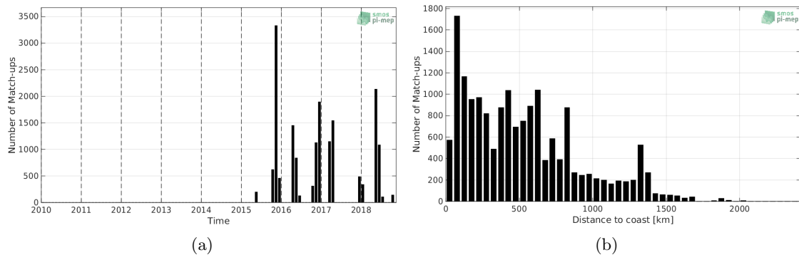
Figure 1: Number of match-ups between TSG-POLARSTERN and SMAP-L2-RSS-V4 SSS as a function of time (a) and as function of the distance to coast (b) over the Atlantic Ocean Pi-MEP region and for the full satellite product period.
