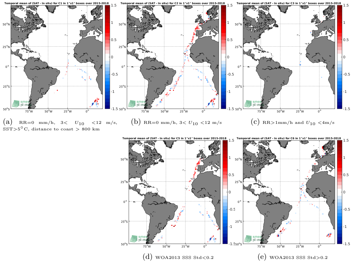
Figure 12: Temporal mean gridded over spatial boxes of size 1^\circ \times 1^\circ of \Delta SSS (SMAP-L2-RSS-V4 - TSG-POLARSTERN) for 5 different subdatasets corresponding to: RR=0 mm/h, 3 < U_{10} < 12 m/s, SST > 5^\circ C , distance to coast > 800 km (a), RR=0 mm/h, 3 < U_{10} < 12 m/s (b), RR > 1 mm/h and U_{10} < 4 m/s (c), WOA2013 SSS Std < 0.2 (d), WOA2013 SSS Std > 0.2 (e).
