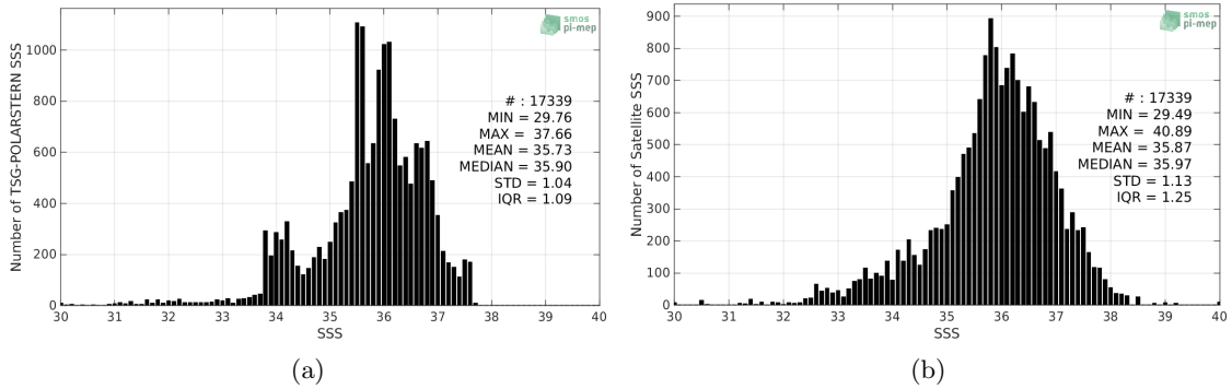
Figure 2: Histograms of SSS from TSG-POLARSTERN (a) and SMAP-L2-RSS-V4 (b) considering all match-up pairs per bins of 0.1 over the Atlantic Ocean Pi-MEP region and for the full satellite product period.
