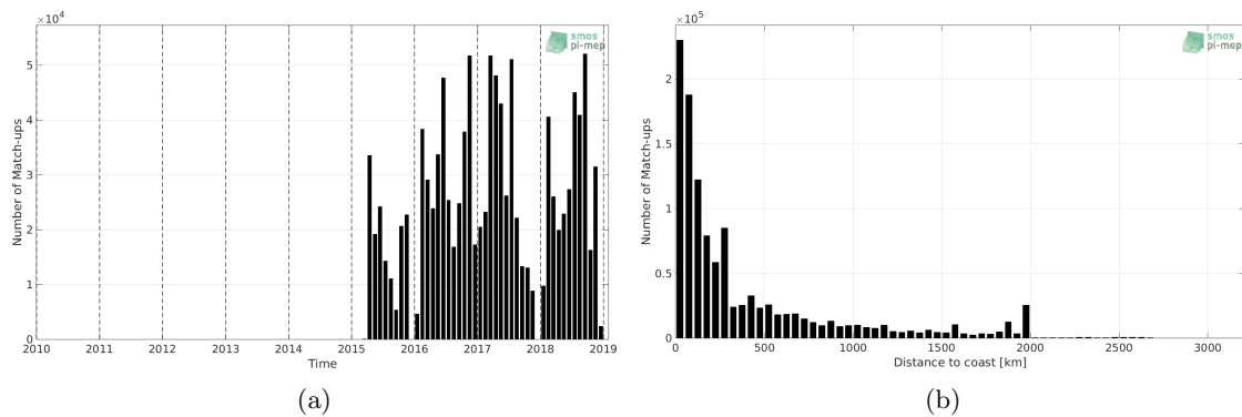
Figure 1: Number of match-ups between TSG-GOSUD-Research-vessel and SMAP-L2-RSS-V4 SSS as a function of time (a) and as function of the distance to coast (b) over the Atlantic Ocean Pi-MEP region and for the full satellite product period.
