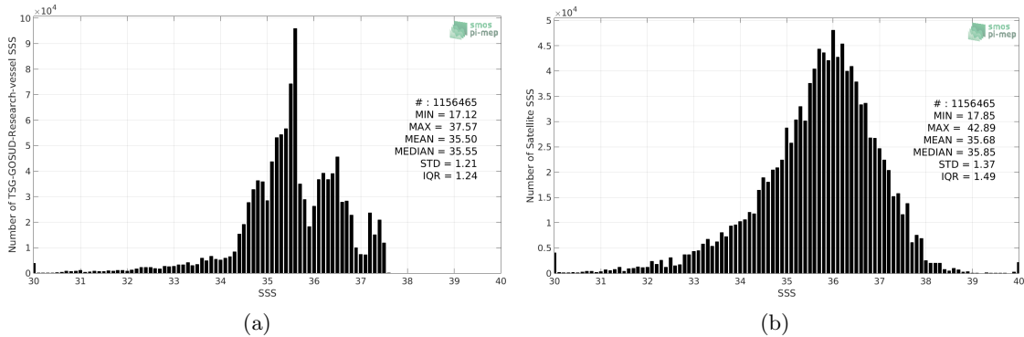
Figure 2: Histograms of SSS from TSG-GOSUD-Research-vessel (a) and SMAP-L2-RSS-V4 (b) considering all match-up pairs per bins of 0.1 over the Atlantic Ocean Pi-MEP region and for the full satellite product period.
