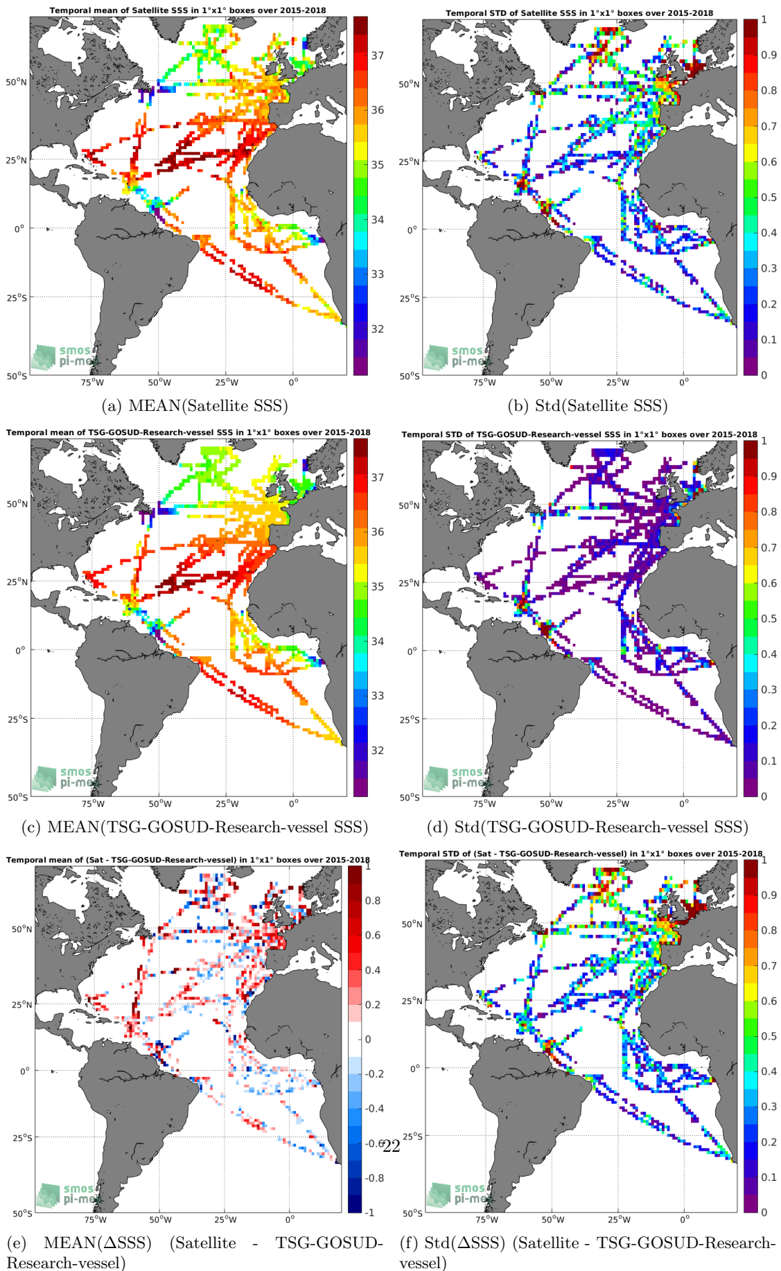
Figure 6: Temporal mean (left) and Std (right) of SSS from SMAP-L2-RSS-V4 (top), TSG-GOSUD-Research-vessel (middle), and of \Delta SSS (Satellite - TSG-GOSUD-Research-vessel). Only match-up pairs are used to generate these maps.
