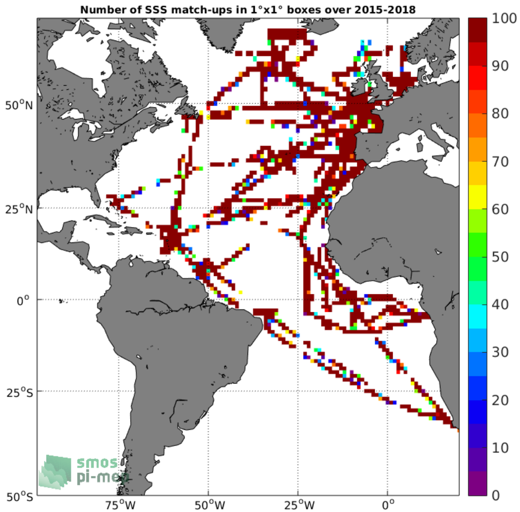
Figure 4: Number of SSS match-ups between TSG-GOSUD-Research-vessel SSS and the SMAP-L2-RSS-V4 SSS product for the Atlantic Ocean Pi-MEP region over 1°x1° boxes and for the full satellite product period.
