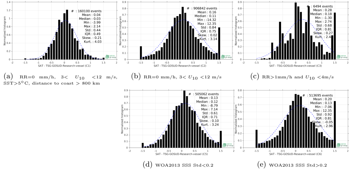
Figure 13: Normalized histogram of \Delta SSS (SMAP-L2-RSS-V4 - TSG-GOSUD-Research-vessel) for 5 different subdatasets corresponding to: RR=0 mm/h, 3 < U_{10} < 12 m/s, SST > 5°C, distance to coast > 800 km (a), RR=0 mm/h, 3 < U_{10} < 12 m/s (b), RR > 1mm/h and U_{10} < 4 m/s (c), WOA2013 SSS Std < 0.2 (d), WOA2013 SSS Std > 0.2 (e).
