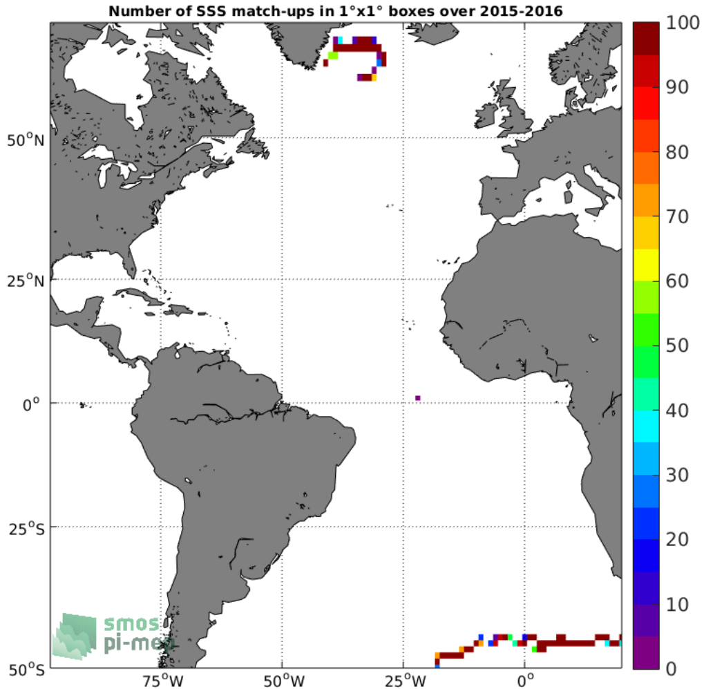
Figure 3: Number of SSS match-ups between Surface drifters SSS and the SMAP SSS L2 v4 (RSS) SSS product for the Atlantic Ocean Pi-MEP region over 1°x1° boxes and for the full satellite product period.
