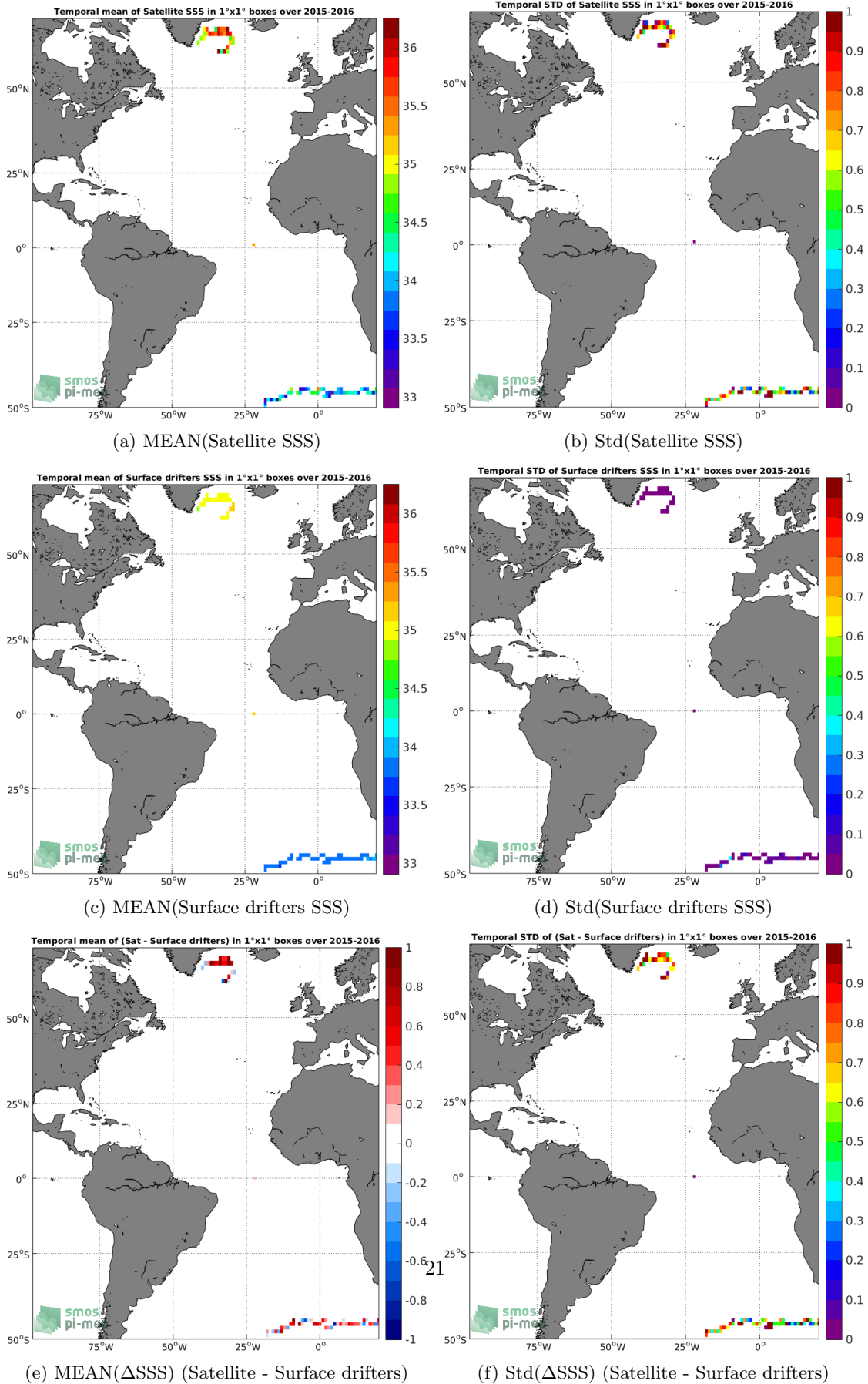
Figure 5: Temporal mean (left) and Std (right) of SSS from SMAP SSS L2 v4 (RSS) (top), Surface drifters (middle), and of \Delta SSS (Satellite - Surface drifters). Only match-up pairs are used to generate these maps.
