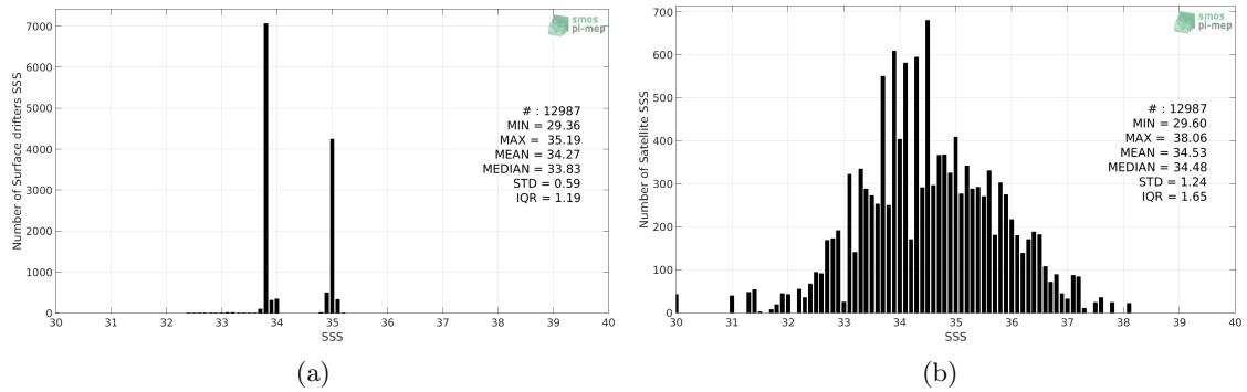
Figure 2: Histograms of SSS from Surface drifters (a) and SMAP SSS L2 v4 (RSS) (b) considering all match-up pairs per bins of 0.1 over the Atlantic Ocean Pi-MEP region and for the full satellite product period.
