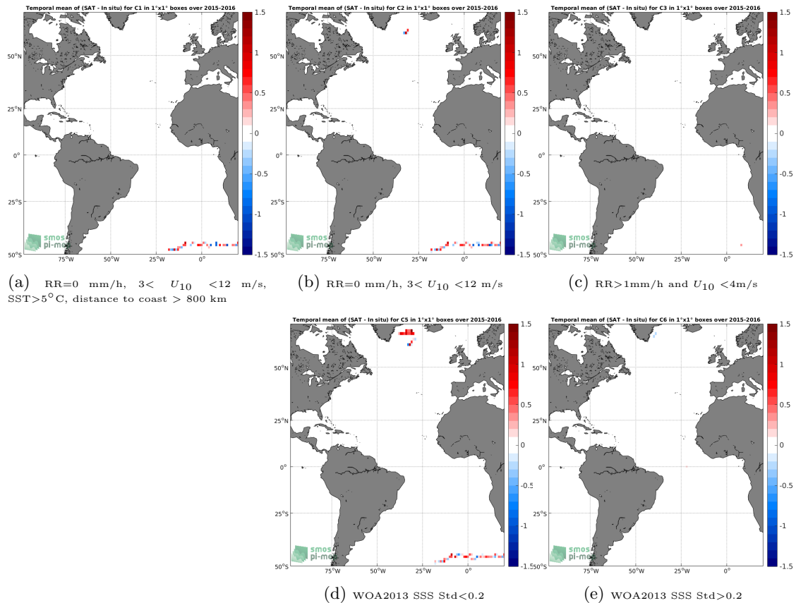
Figure 11: Temporal mean gridded over spatial boxes of size 1^{\circ}\times 1^{\circ} of \Delta\text{SSS} (SMAP SSS L2 v4 (RSS) - Surface drifters) for 5 different subdatasets corresponding to:RR=0 mm/h, 3 < U_{10} < 12 m/s, SST >5^{\circ}\text{C} , distance to coast > 800 km (a), RR=0 mm/h, 3 < U_{10} < 12 m/s (b), RR >1 mm/h and U_{10} < 4 m/s (c), WOA2013 SSS Std <0.2 (d), WOA2013 SSS Std >0.2 (e).
