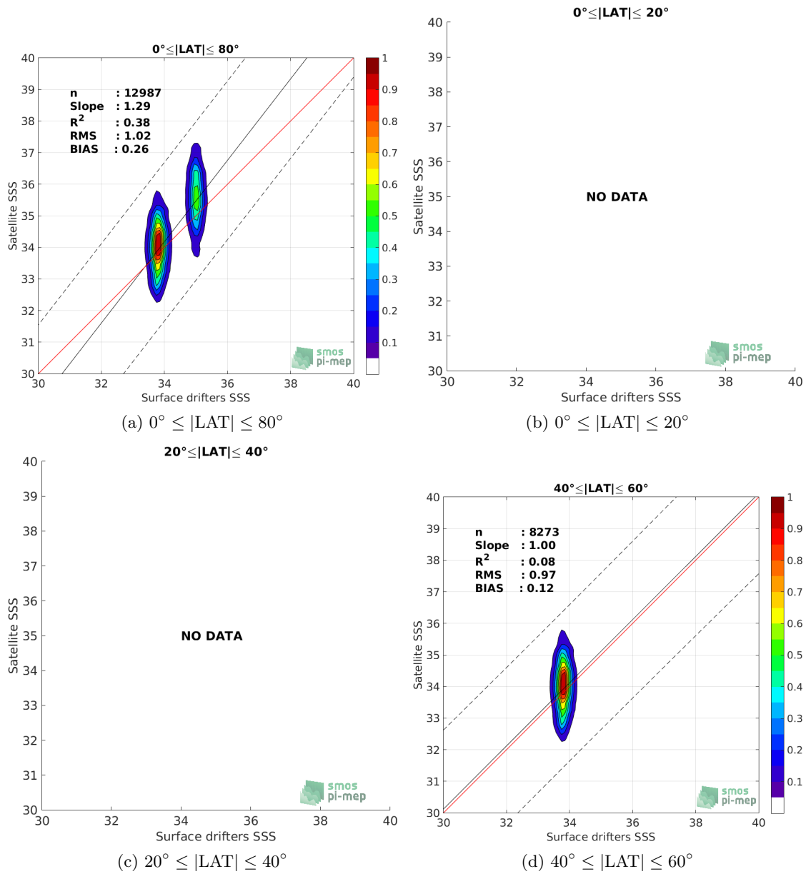
Figure 8: Contour maps of the concentration of SMAP SSS L2 v4 (RSS) SSS (y-axis) versus Surface drifters SSS (x-axis) at match-up pairs for different latitude bands. For each plot, the red line shows x=y . The black thin and dashed lines indicate a linear fit through the data cloud and the \pm 95\% confidence levels, respectively. The number match-up pairs n , the slope and R^2 coefficient of the linear fit, the root mean square (RMS) and the mean bias between satellite and in situ data are indicated for each latitude band in each plots.
