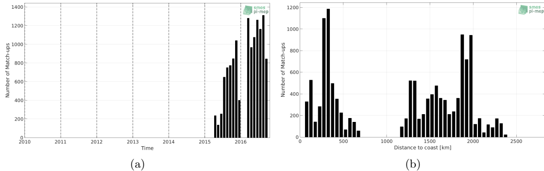
Figure 1: Number of match-ups between Surface drifters and SMAP SSS L2 v4 (RSS) SSS as a function of time (a) and as function of the distance to coast (b) over the Atlantic Ocean Pi-MEP region and for the full satellite product period.
