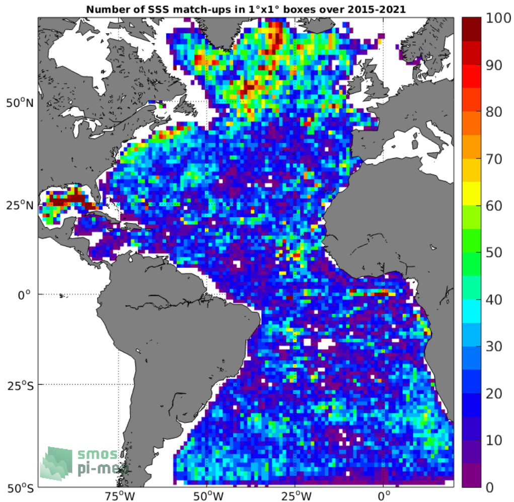
Figure 4: Number of SSS match-ups between Argo SSS and the SMAP SSS L2 v4 (RSS) SSS product for the Atlantic Ocean Pi-MEP region over 1°×1° boxes and for the full satellite product period.
