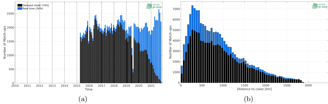
Figure 1: Number of match-ups between Argo and SMAP SSS L2 v4 (RSS) SSS as a function of time (a) and as function of the distance to coast (b) over the Atlantic Ocean Pi-MEP region and for the full satellite product period.
