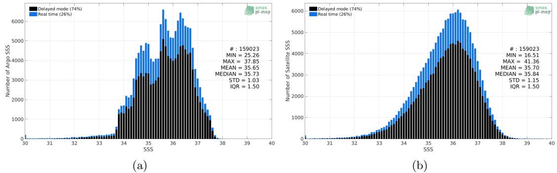
Figure 2: Histograms of SSS from Argo (a) and SMAP SSS L2 v4 (RSS) (b) considering all match-up pairs per bins of 0.1 over the Atlantic Ocean Pi-MEP region and for the full satellite product period.
