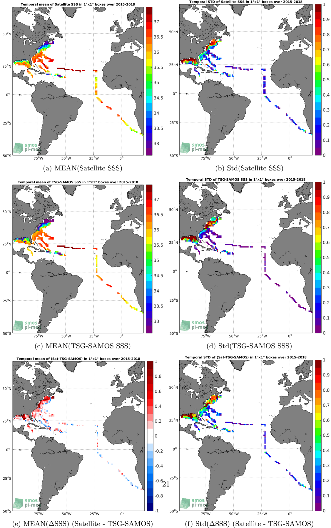
Figure 6: Temporal mean (left) and Std (right) of SSS from SMAP-L2-RSS-V3-70KM (top), TSG-SAMOS (middle), and of \Delta SSS (Satellite - TSG-SAMOS). Only match-up pairs are used to generate these maps.
