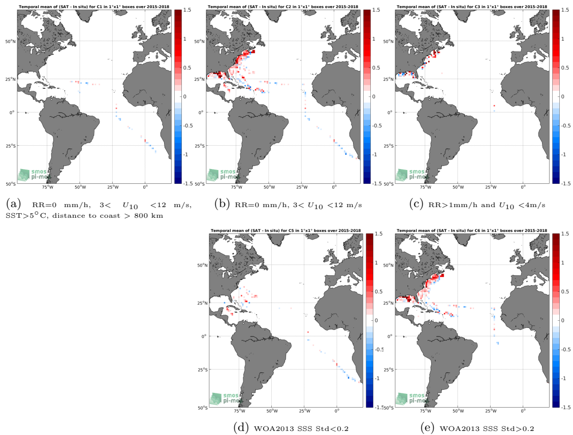
Figure 12: Temporal mean gridded over spatial boxes of size 1^\circ \times 1^\circ of \Delta SSS (SMAP-L2-RSS-V3-70KM - TSG-SAMOS) for 5 different subdatasets corresponding to: RR=0 mm/h, 3 < U_{10} < 12 m/s, SST > 5^\circ C , distance to coast > 800 km (a), RR=0 mm/h, 3 < U_{10} < 12 m/s (b), RR > 1 mm/h and U_{10} < 4 m/s (c), WOA2013 SSS Std < 0.2 (d), WOA2013 SSS Std > 0.2 (e).
