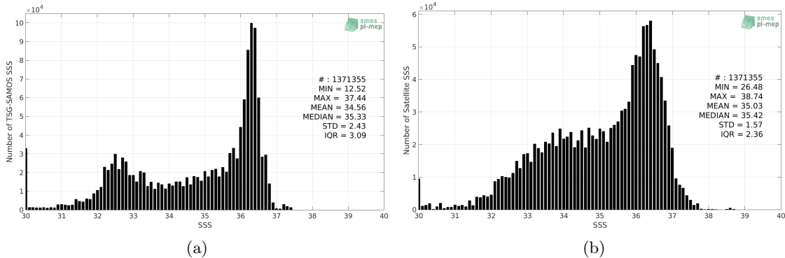
Figure 2: Histograms of SSS from TSG-SAMOS (a) and SMAP-L2-RSS-V3-70KM (b) considering all match-up pairs per bins of 0.1 over the Atlantic Ocean Pi-MEP region and for the full satellite product period.
