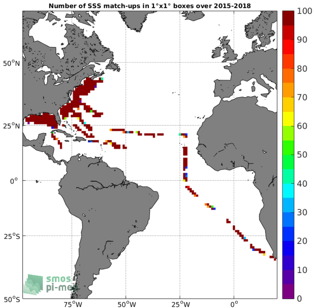
Figure 4: Number of SSS match-ups between TSG-SAMOS SSS and the SMAP-L2-RSS-V3-70KM SSS product for the Atlantic Ocean Pi-MEP region over 1°x1° boxes and for the full satellite product period.
