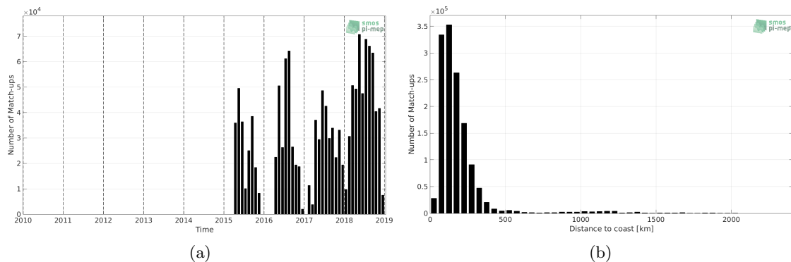
Figure 1: Number of match-ups between TSG-SAMOS and SMAP-L2-RSS-V3-70KM SSS as a function of time (a) and as function of the distance to coast (b) over the Atlantic Ocean Pi-MEP region and for the full satellite product period.
