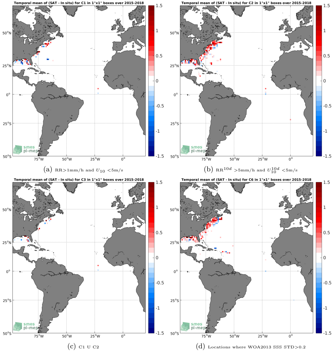
Figure 12: Temporal mean gridded over spatial boxes of size 1^\circ \times 1^\circ of \Delta SSS (SMAP-L2-RSS-V3-70KM - TSG-SAMOS) for 4 different subdatasets corresponding to: RR > 1\text{mm/h} and U_{10} < 5\text{m/s} (a), RR^{10d} > 5\text{mm/h} and U_{10}^{10d} < 5\text{m/s} (b), C1 U C2 (c), Locations where WOA2013 SSS STD > 0.2 (d).
