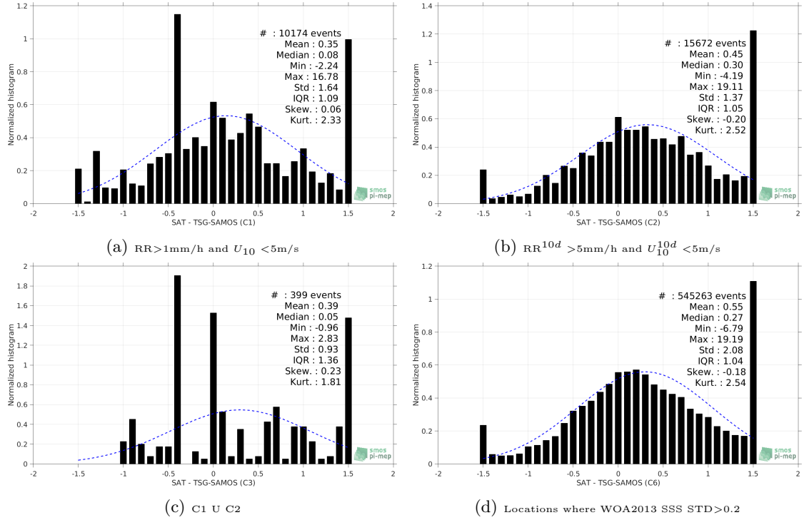
Figure 13: Normalized histogram of \Delta\text{SSS} (SMAP-L2-RSS-V3-70KM - TSG-SAMOS) for 6 different subdatasets corresponding to: RR > 1mm/h and U_{10} < 5\text{m/s} (a), RR^{10d} > 5\text{mm/h} and U_{10}^{10d} < 5\text{m/s} (b), C1 U C2 (c), Locations where WOA2013 SSS STD > 0.2 (d).
