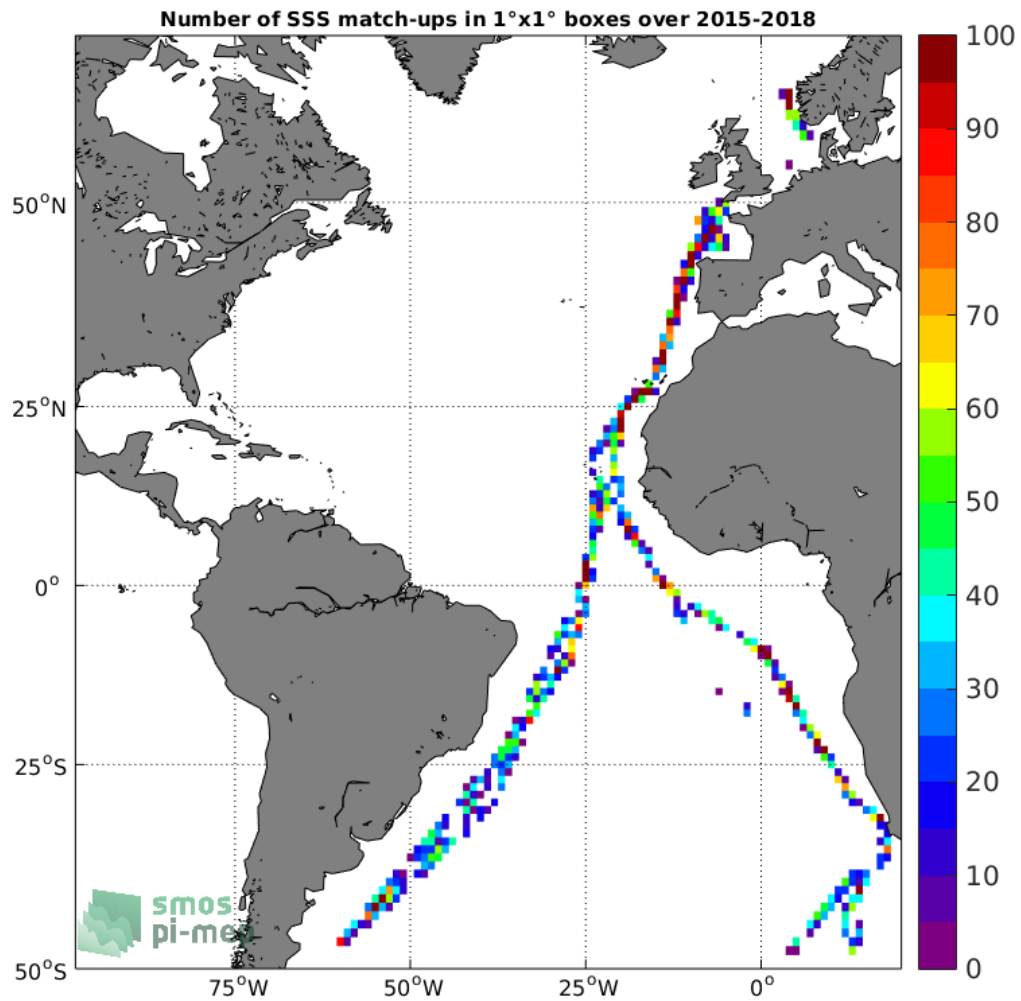
Figure 4: Number of SSS match-ups between TSG-POLARSTERN SSS and the SMAP-L2-RSS-V3-70KM SSS product for the Atlantic Ocean Pi-MEP region over 1°x1° boxes and for the full satellite product period.
