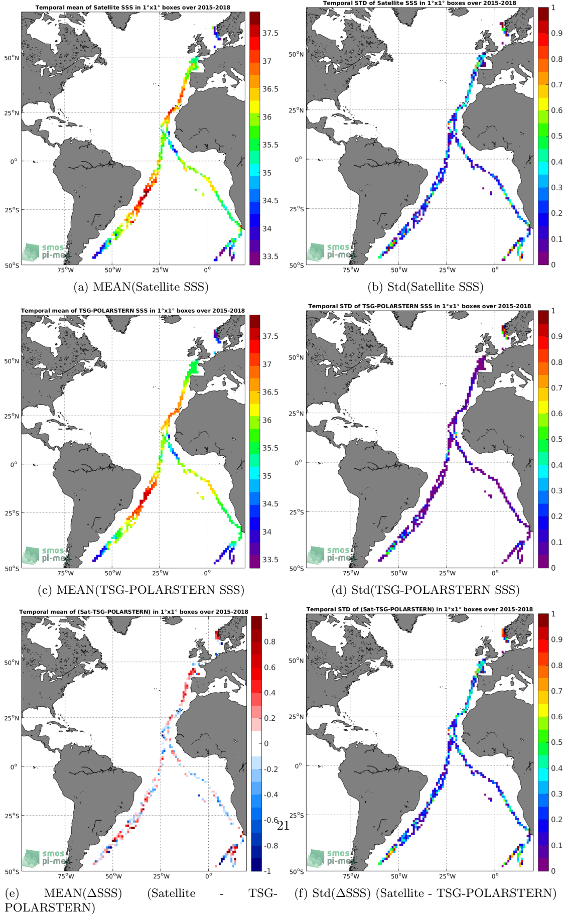
Figure 6: Temporal mean (left) and Std (right) of SSS from SMAP-L2-RSS-V3-70KM (top), TSG-POLARSTERN (middle), and of \Delta SSS (Satellite - TSG-POLARSTERN). Only match-up pairs are used to generate these maps.
