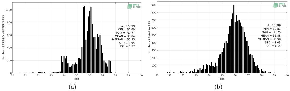
Figure 2: Histograms of SSS from TSG-POLARSTERN (a) and SMAP-L2-RSS-V3-70KM (b) considering all match-up pairs per bins of 0.1 over the Atlantic Ocean Pi-MEP region and for the full satellite product period.
