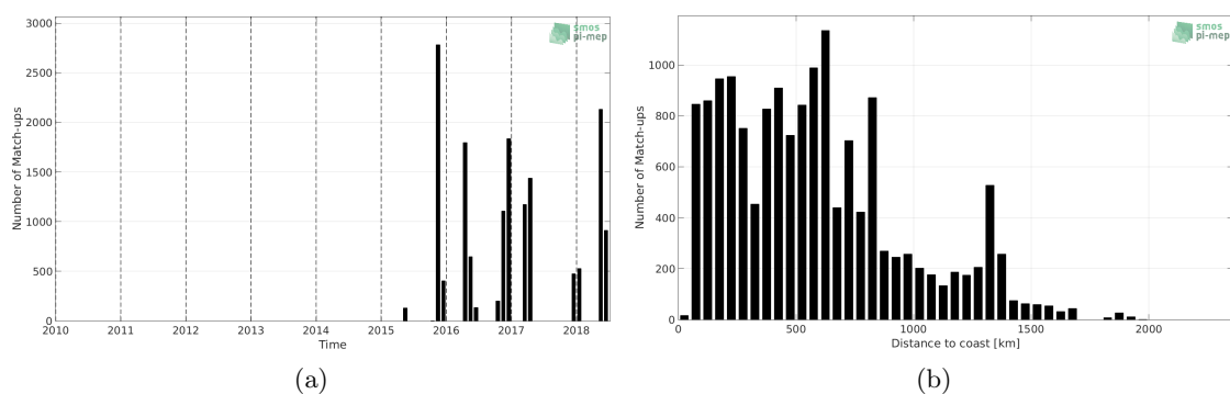
Figure 1: Number of match-ups between TSG-POLARSTERN and SMAP-L2-RSS-V3-70KM SSS as a function of time (a) and as function of the distance to coast (b) over the Atlantic Ocean Pi-MEP region and for the full satellite product period.
