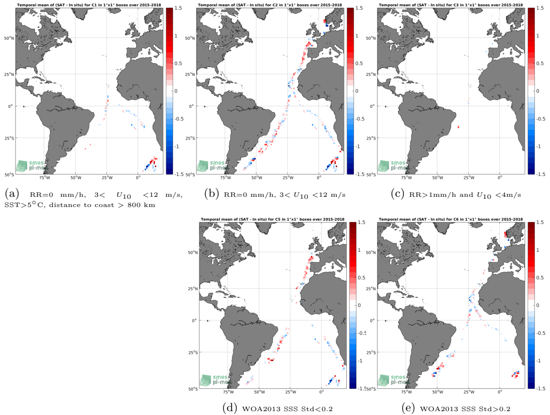
Figure 12: Temporal mean gridded over spatial boxes of size 1^\circ \times 1^\circ of \Delta SSS (SMAP-L2-RSS-V3-70KM - TSG-POLARSTERN) for 5 different subdatasets corresponding to: RR=0 mm/h, 3 < U_{10} < 12 m/s, SST > 5^\circ C , distance to coast > 800 km (a), RR=0 mm/h, 3 < U_{10} < 12 m/s (b), RR > 1 mm/h and U_{10} < 4 m/s (c), WOA2013 SSS Std < 0.2 (d), WOA2013 SSS Std > 0.2 (e).
