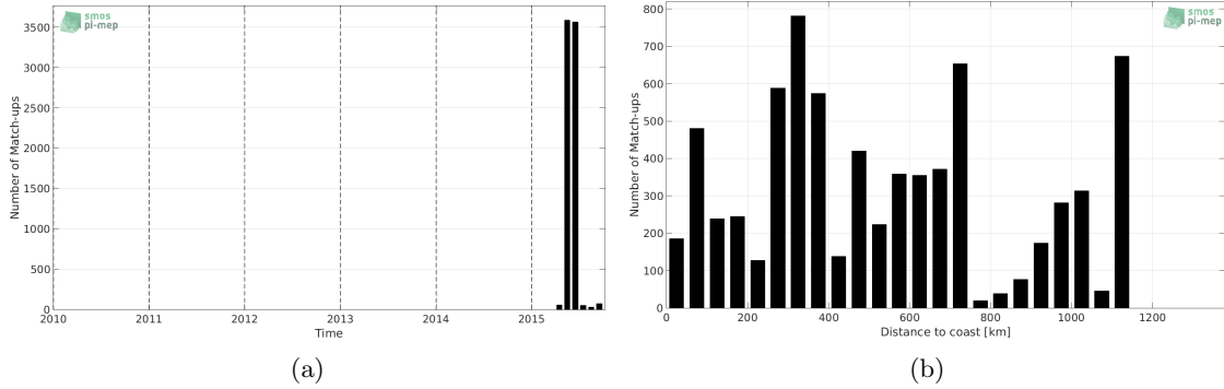
Figure 1: Number of match-ups between TSG-GOSUD-Sailing-ship and SMAP-L2-RSS-V3-70KM SSS as a function of time (a) and as function of the distance to coast (b) over the Atlantic Ocean Pi-MEP region and for the full satellite product period.
