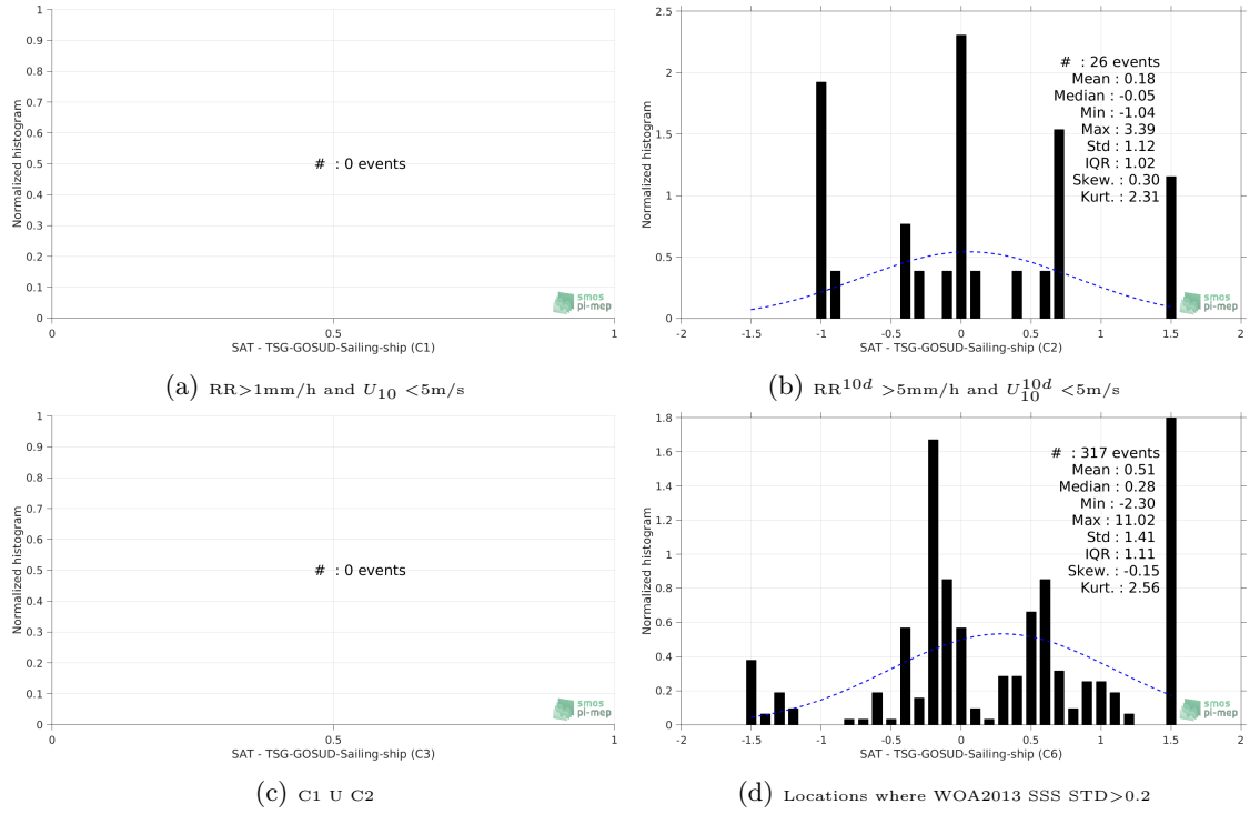
Figure 13: Normalized histogram of \Delta\text{SSS} (SMAP-L2-RSS-V3-70KM - TSG-GOSUD-Sailing-ship) for 6 different subdatasets corresponding to: RR > 1\text{mm/h} and U_{10} < 5\text{m/s} (a), RR^{10d} > 5\text{mm/h} and U_{10}^{10d} < 5\text{m/s} (b), C1 \cup C2 (c), Locations where WOA2013 SSS STD > 0.2 (d).
