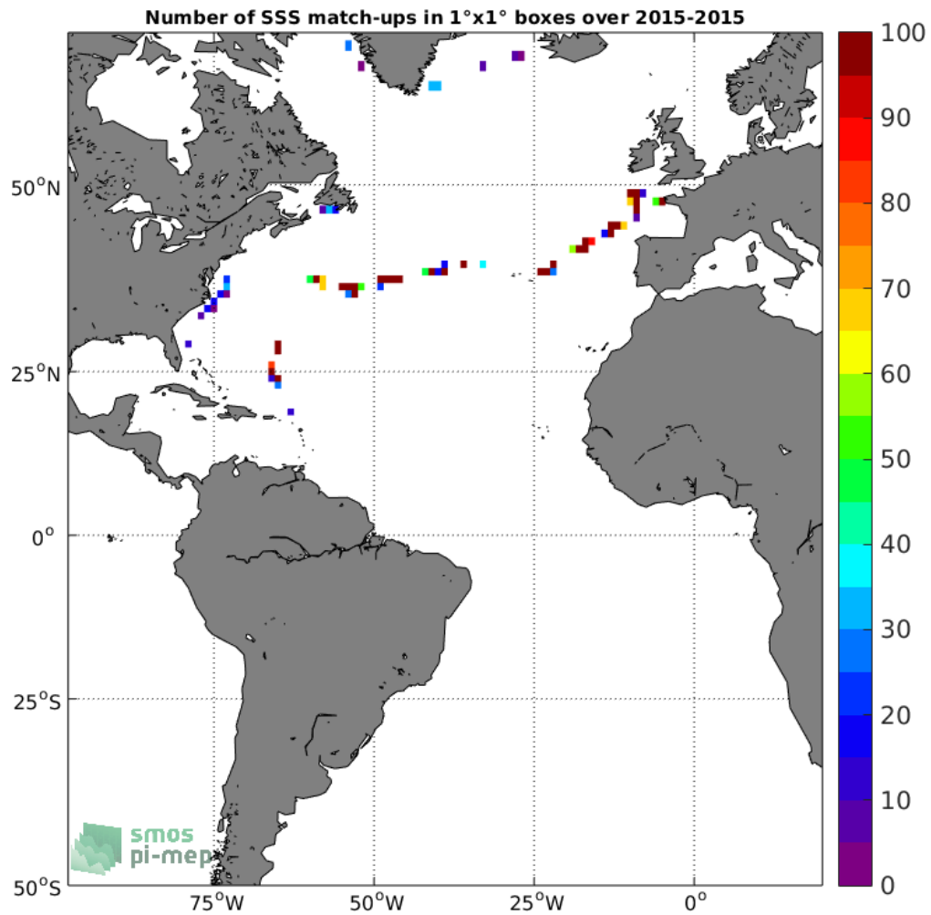
Figure 4: Number of SSS match-ups between TSG-GOSUD-Sailing-ship SSS and the SMAP-L2-RSS-V3-70KM SSS product for the Atlantic Ocean Pi-MEP region over 1°x1° boxes and for the full satellite product period.
