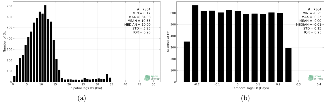
Figure 5: Histograms of the spatial (a) and temporal (b) lags between the time of the TSG-GOSUD-Sailing-ship measurements and the date of the corresponding SMAP-L2-RSS-V3-70KM SSS product.
