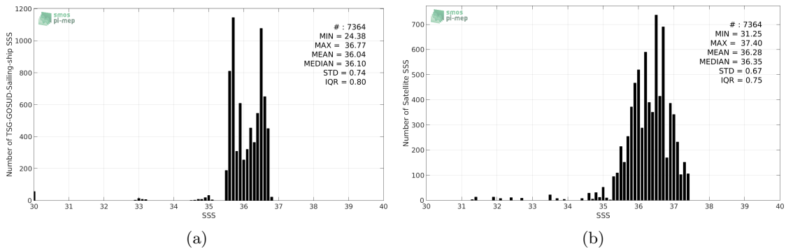
Figure 2: Histograms of SSS from TSG-GOSUD-Sailing-ship (a) and SMAP-L2-RSS-V3-70KM (b) considering all match-up pairs per bins of 0.1 over the Atlantic Ocean Pi-MEP region and for the full satellite product period.
