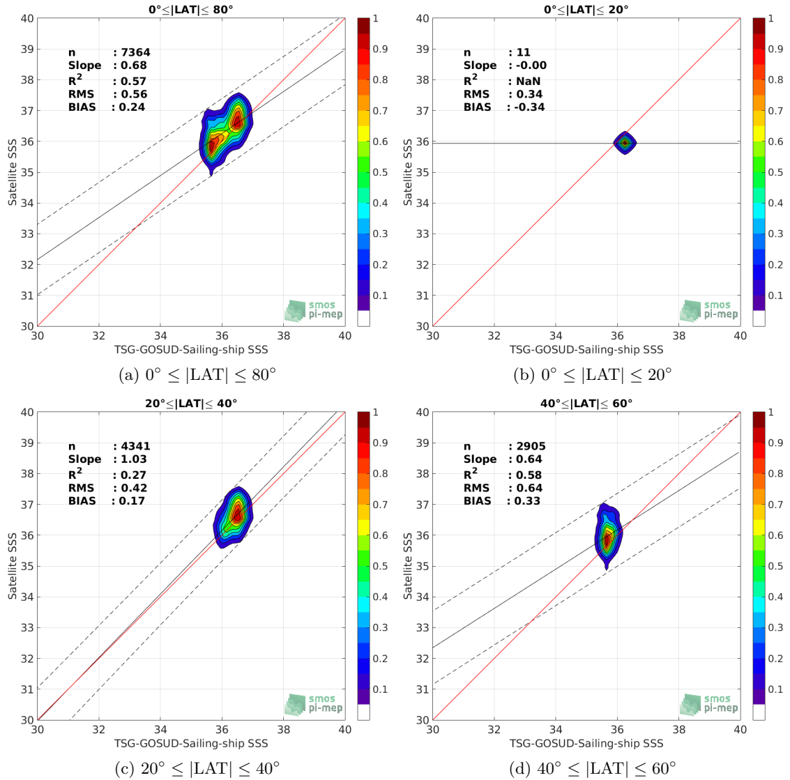
Figure 9: Contour maps of the concentration of SMAP-L2-RSS-V3-70KM SSS (y-axis) versus TSG-GOSUD-Sailing-ship SSS (x-axis) at match-up pairs for different latitude bands. For each plot, the red line shows x=y . The black thin and dashed lines indicate a linear fit through the data cloud and the \pm 95\% confidence levels, respectively. The number match-up pairs n , the slope and R^2 coefficient of the linear fit, the root mean square (RMS) and the mean bias between satellite and in situ data are indicated for each latitude band in each plots.
