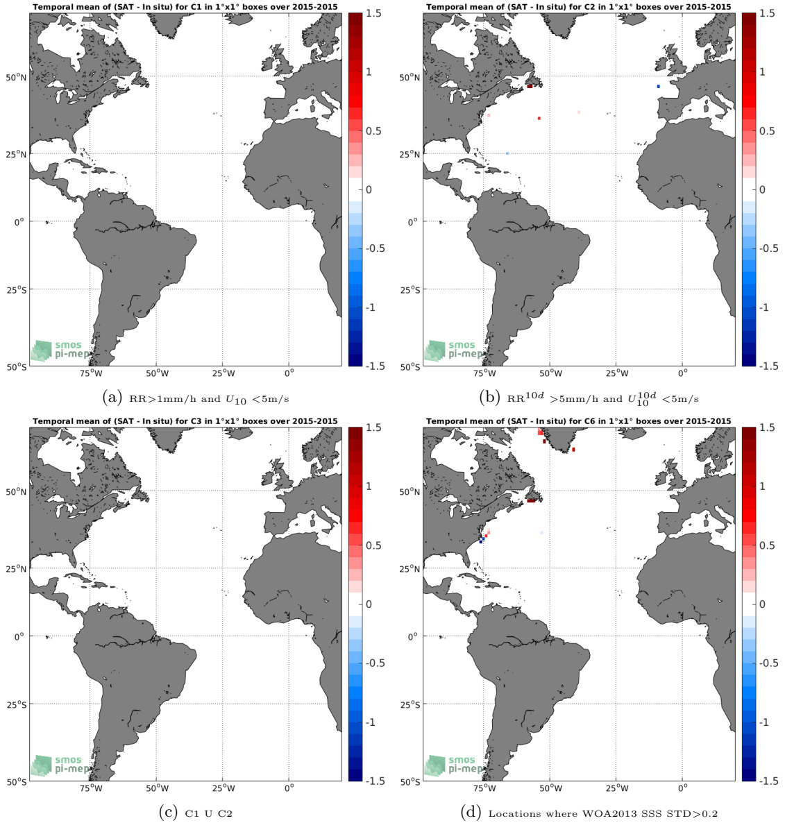
Figure 12: Temporal mean gridded over spatial boxes of size 1^\circ \times 1^\circ of \Delta SSS (SMAP-L2-RSS-V3-70KM - TSG-GOSUD-Sailing-ship) for 4 different subdatasets corresponding to: RR > 1mm/h and U_{10} < 5m/s (a), RR 10d > 5mm/h and U_{10}^{10d} < 5m/s (b), C1 U C2 (c), Locations where WOA2013 SSS STD > 0.2 (d).
