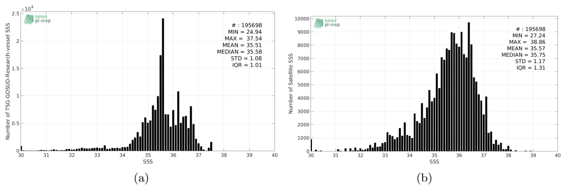
Figure 2: Histograms of SSS from TSG-GOSUD-Research-vessel (a) and SMAP-L2-RSS-V3-70KM (b) considering all match-up pairs per bins of 0.1 over the Atlantic Ocean Pi-MEP region and for the full satellite product period.
