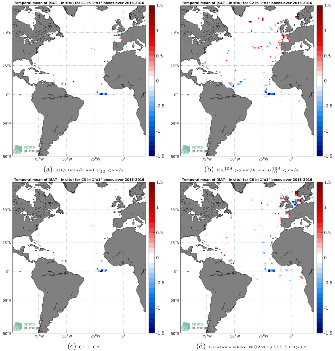
Figure 12: Temporal mean gridded over spatial boxes of size 1^\circ \times 1^\circ of \Delta SSS (SMAP-L2-RSS-V3-70KM - TSG-GOSUD-Research-vessel) for 4 different subdatasets corresponding to:RR>1mm/h and U_{10} < 5m/s (a), RR^{10d} > 5mm/h and U_{10}^{10d} < 5m/s (b), C1 U C2 (c),Locations where WOA2013 SSS STD>0.2 (d).
