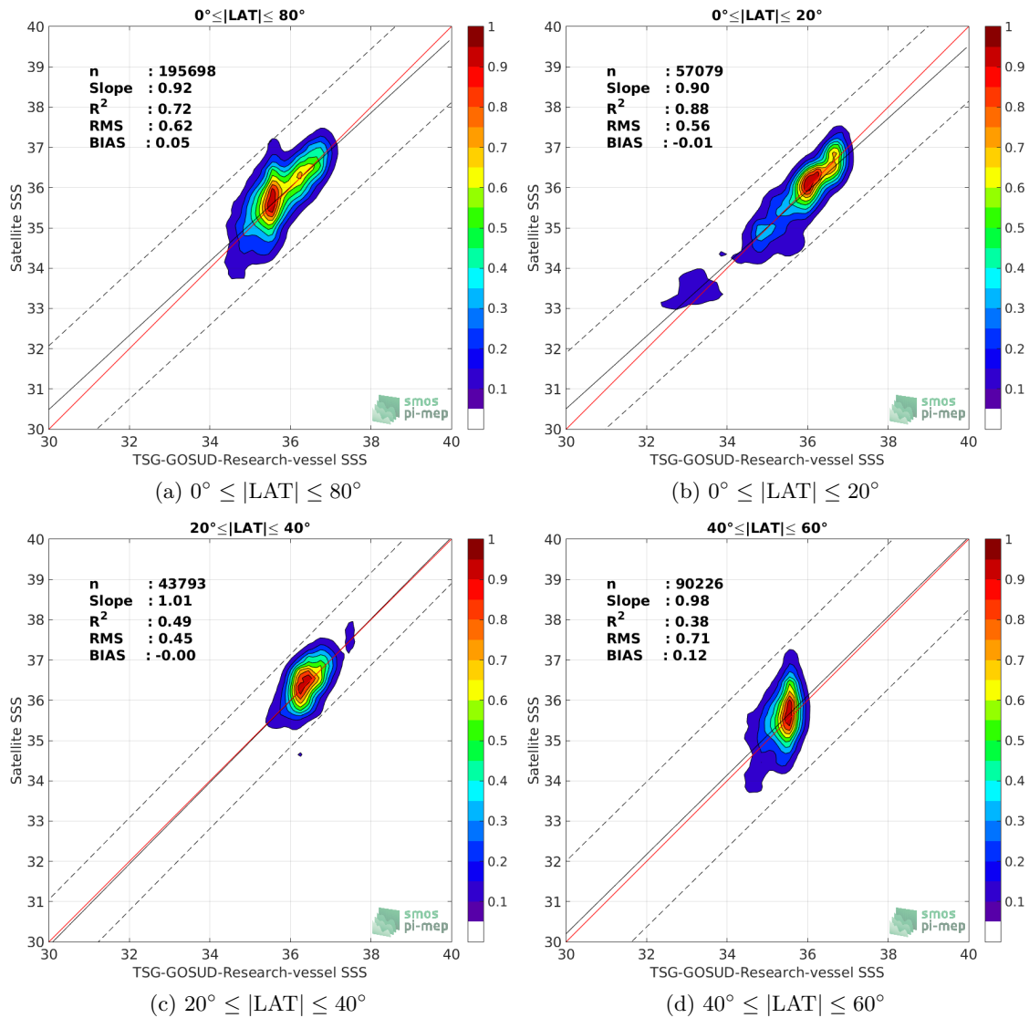
Figure 9: Contour maps of the concentration of SMAP-L2-RSS-V3-70KM SSS (y-axis) versus TSG-GOSUD-Research-vessel SSS (x-axis) at match-up pairs for different latitudinal bands. For each plot, the red line shows x=y . The black thin and dashed lines indicate a linear fit through the data cloud and the \pm 95\% confidence levels, respectively. The number match-up pairs n , the slope and R^2 coefficient of the linear fit, the root mean square (RMS) and the mean bias between satellite and in situ data are indicated for each latitude band in each plots.
