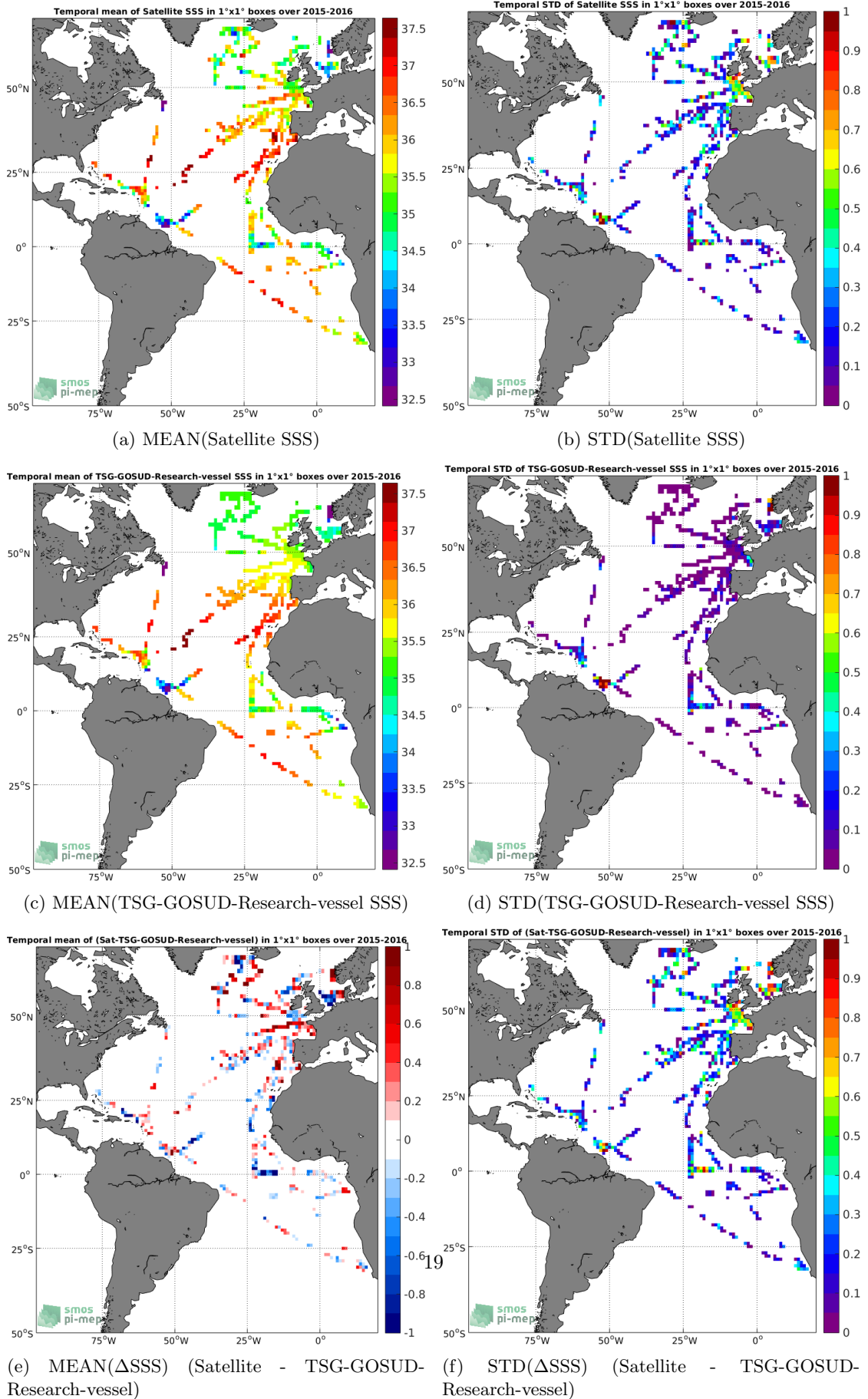
Figure 6: Temporal mean (left) and STD (right) of SSS from SMAP-L2-RSS-V3-70KM (top), TSG-GOSUD-Research-vessel (middle), and of \Delta SSS (Satellite - TSG-GOSUD-Research-vessel). Only match-up pairs are used to generate these maps.
