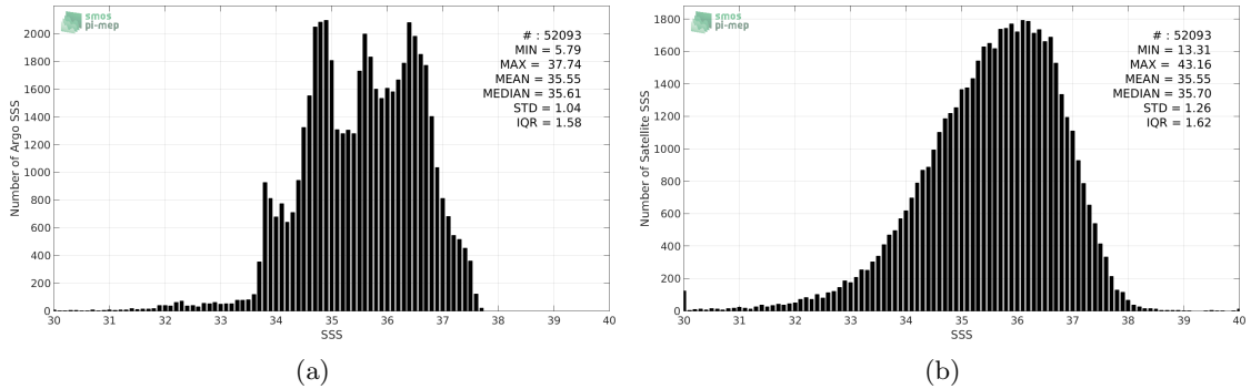
Figure 2: Histograms of SSS from Argo (a) and SMAP-L2-RSS-V3-70KM (b) considering all match-up pairs per bins of 0.1 over the Atlantic Ocean Pi-MEP region and for the full satellite product period.
