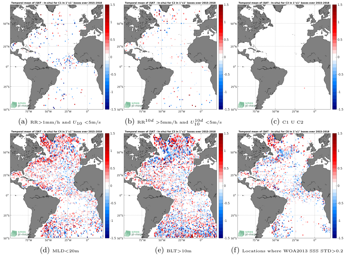
Figure 12: Temporal mean gridded over spatial boxes of size 1^\circ \times 1^\circ of \Delta\text{SSS} (SMAP-L2-RSS-V3-70KM - Argo) for 6 different subdatasets corresponding to: \text{RR} > 1\text{mm/h} and U_{10} < 5\text{m/s} (a), \text{RR}^{10d} > 5\text{mm/h} and U_{10}^{10d} < 5\text{m/s} (b), C1 U C2 (c), \text{MLD} < 20\text{m} (d), \text{BLT} > 10\text{m} (e), Locations where WOA2013 SSS STD > 0.2 (f).
