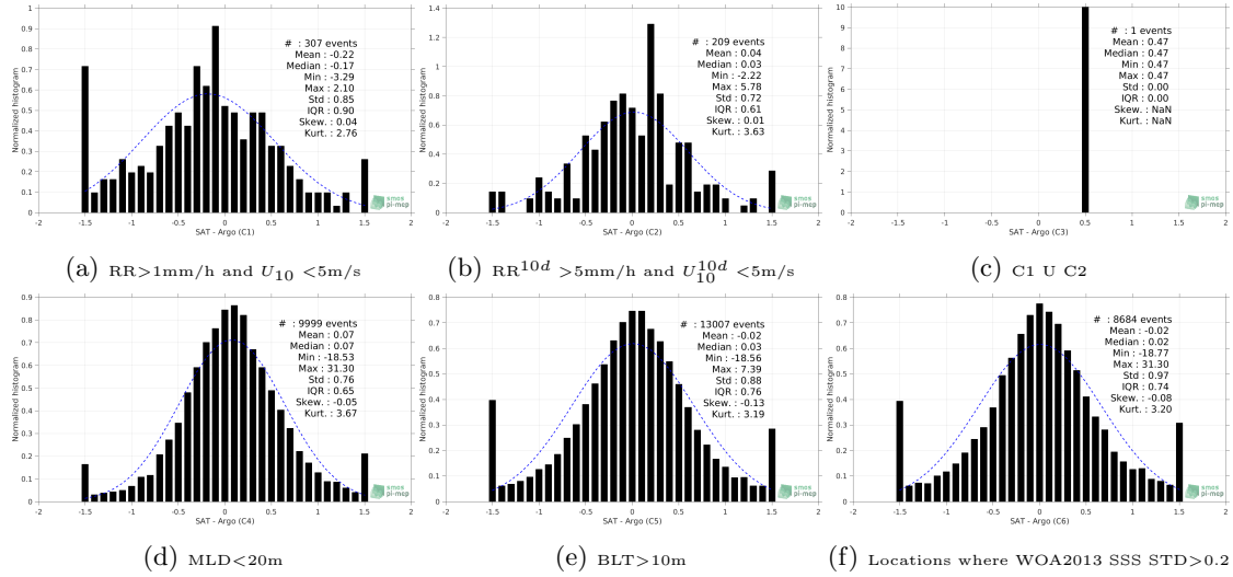
Figure 13: Normalized histogram of \Delta\text{SSS} (SMAP-L2-RSS-V3-70KM - Argo) for 6 different sub-datasets corresponding to: \text{RR} > 1\text{mm/h} and U_{10} < 5\text{m/s} (a), \text{RR}^{10d} > 5\text{mm/h} and U_{10}^{10d} < 5\text{m/s} (b), C1 \cup C2 (c), \text{MLD} < 20\text{m} (d), \text{BLT} > 10\text{m} (e), Locations where \text{WOA2013 SSS STD} > 0.2 (f).
