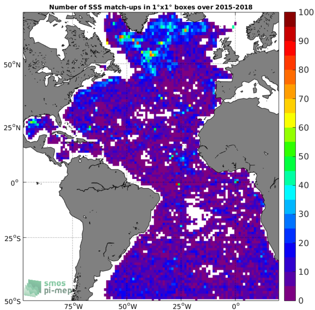
Figure 4: Number of SSS match-ups between Argo SSS and the SMAP-L2-RSS-V3-70KM SSS product for the Atlantic Ocean Pi-MEP region over 1°x1° boxes and for the full satellite product period.
