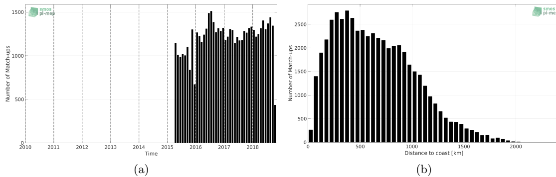
Figure 1: Number of match-ups between Argo and SMAP-L2-RSS-V3-70KM SSS as a function of time (a) and as function of the distance to coast (b) over the Atlantic Ocean Pi-MEP region and for the full satellite product period.
