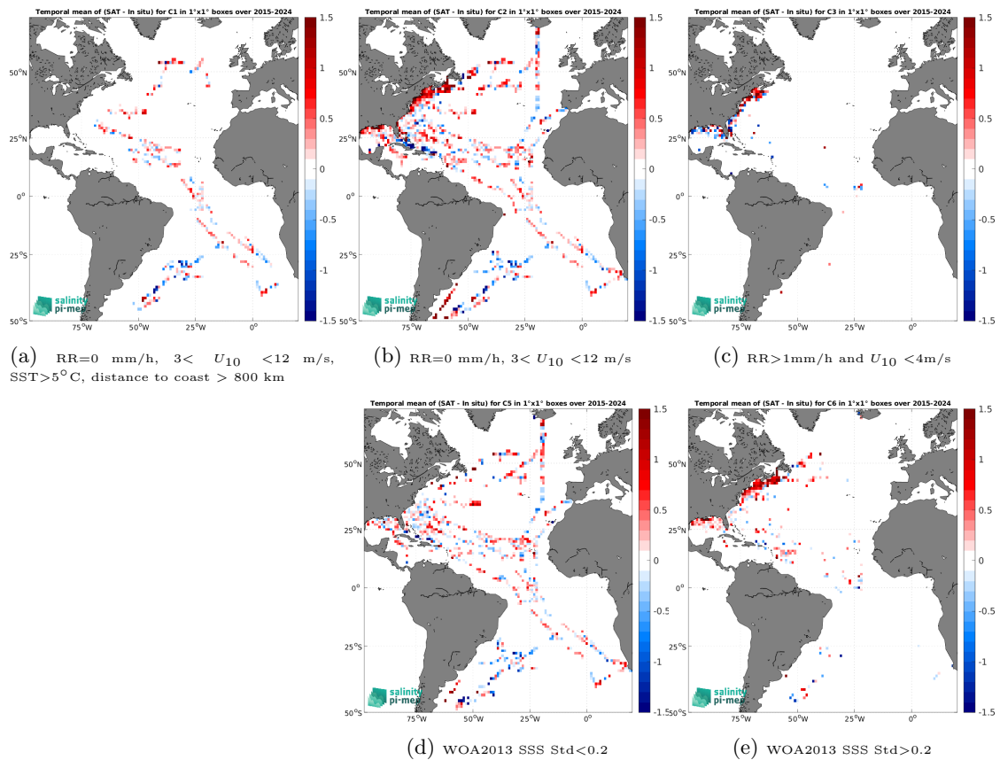
Figure 14: Temporal mean gridded over spatial boxes of size 1^\circ \times 1^\circ of \Delta\text{SSS} (SMAP SSS L2 v5.0 (JPL) - TSG (SAMOS)) for 5 different subdatasets corresponding to:RR=0 mm/h, 3 < U_{10} < 12 m/s, SST >5^\circ\text{C} , distance to coast > 800 km (a), RR=0 mm/h, 3 < U_{10} < 12 m/s (b), RR >1 mm/h and U_{10} < 4 m/s (c), WOA2013 SSS Std <0.2 (d), WOA2013 SSS Std >0.2 (e).
