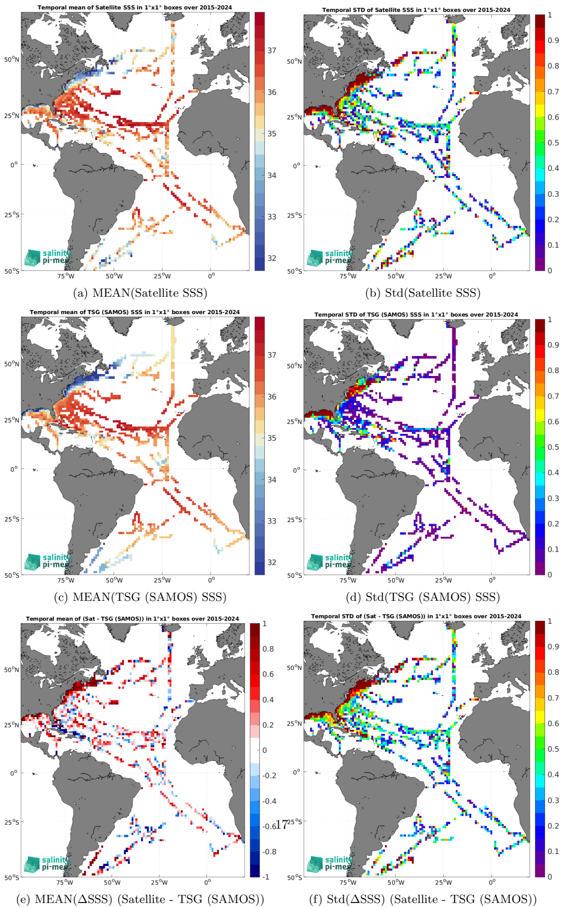
(e) MEAN( \Delta SSS) (Satellite - TSG (SAMOS)) (f) Std( \Delta SSS) (Satellite - TSG (SAMOS)) Figure 7: Temporal mean (left) and Std (right) of SSS from SMAP SSS L2 v5.0 (JPL) (top), TSG (SAMOS) (middle), and of \Delta SSS (Satellite - TSG (SAMOS)). Only match-up pairs are used to generate these maps.
