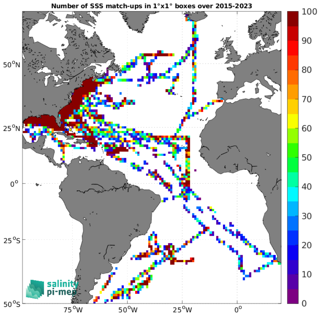
Figure 4: Number of SSS match-ups between TSG (SAMOS) SSS and the SMAP SSS L2 v5.0 (JPL) SSS product for the Atlantic Ocean Pi-MEP region over 1^{\circ} \times 1^{\circ} boxes and for the full satellite product period.
