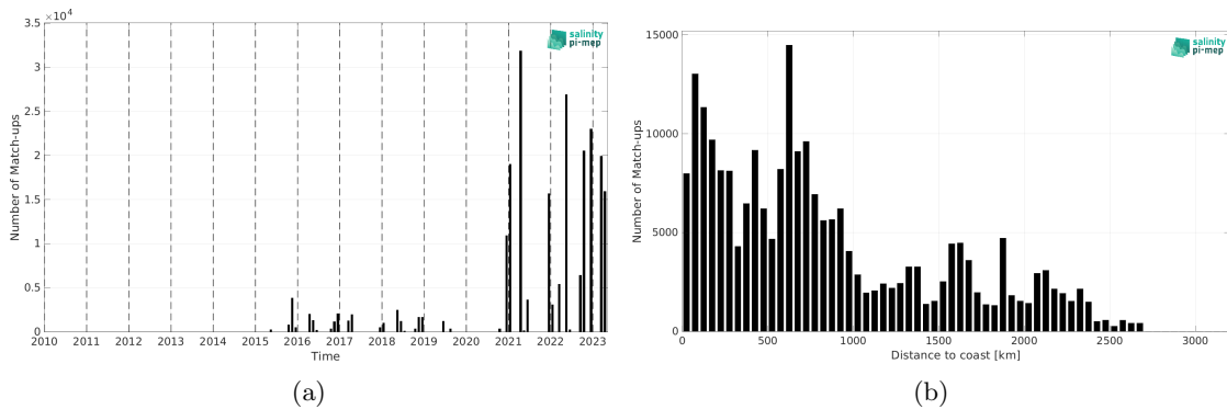
Figure 2: Number of match-ups between TSG (Polarstern) and SMAP SSS L2 v5.0 (JPL) SSS as a function of time (a) and as function of the distance to coast (b) over the Atlantic Ocean Pi-MEP region and for the full satellite product period.
