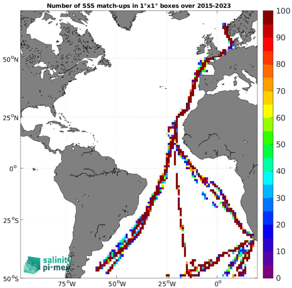
Figure 5: Number of SSS match-ups between TSG (Polarstern) SSS and the SMAP SSS L2 v5.0 (JPL) SSS product for the Atlantic Ocean Pi-MEP region over 1^\circ \times 1^\circ boxes and for the full satellite product period.
