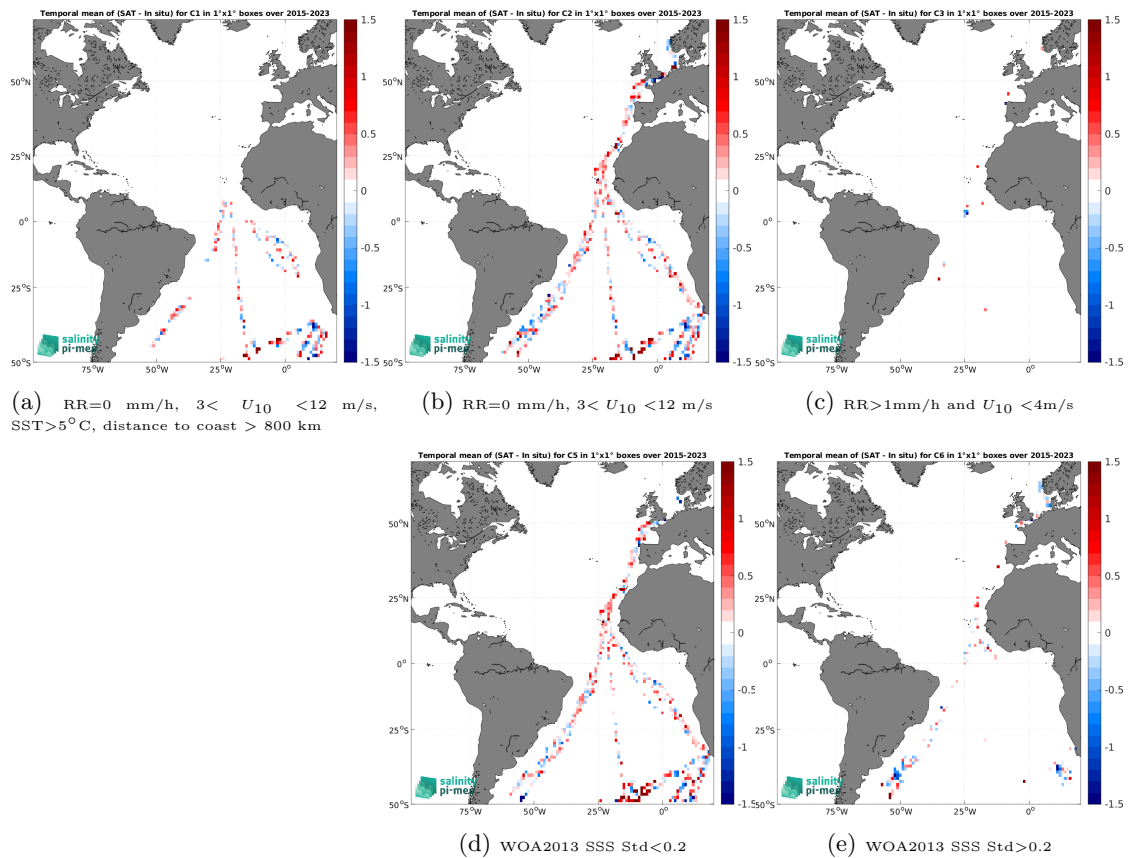
Figure 14: Temporal mean gridded over spatial boxes of size 1^\circ \times 1^\circ of \Delta\text{SSS} (SMAP SSS L2 v5.0 (JPL) - TSG (Polarstern)) for 5 different subdatasets corresponding to:RR=0 mm/h, 3 < U_{10} < 12 m/s, SST>5°C, distance to coast > 800 km (a), RR=0 mm/h, 3 < U_{10} < 12 m/s (b), RR>1mm/h and U_{10} < 4 m/s (c), WOA2013 SSS Std<0.2 (d), WOA2013 SSS Std>0.2 (e).
