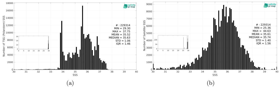
Figure 3: Histograms of SSS from TSG (Polarstern) (a) and SMAP SSS L2 v5.0 (JPL) (b) considering all match-up pairs per bins of 0.1 over the Atlantic Ocean Pi-MEP region and for the full satellite product period.
