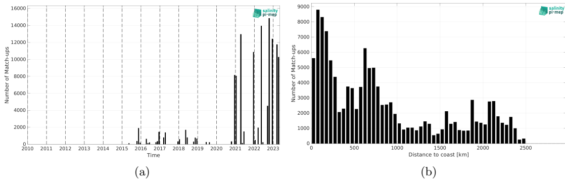
Figure 2: Number of match-ups between TSG (Polarstern) and SMAP SSS L2 v5.0 (JPL) SSS as a function of time (a) and as function of the distance to coast (b) over the Atlantic Ocean Pi-MEP region and for the full satellite product period.
