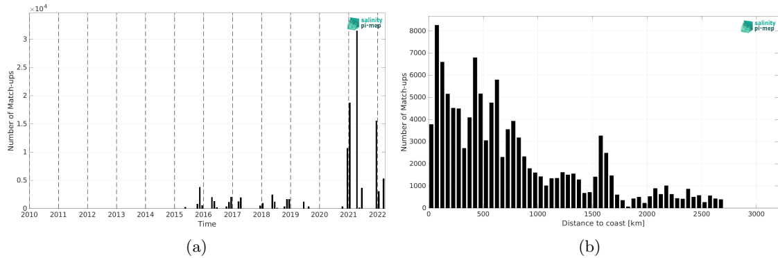
Figure 1: Number of match-ups between TSG (Polarstern) and SMAP SSS L2 v5.0 (JPL) SSS as a function of time (a) and as function of the distance to coast (b) over the Atlantic Ocean Pi-MEP region and for the full satellite product period.
