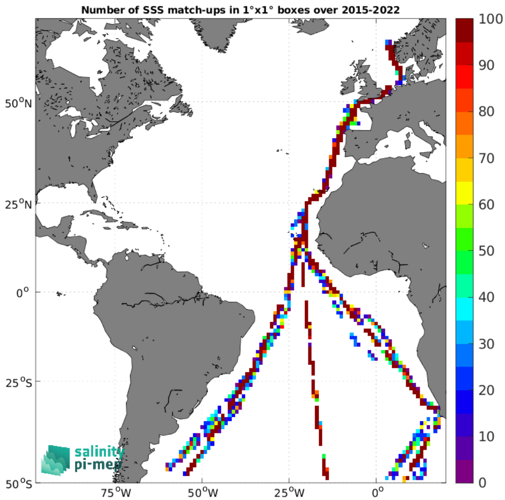
Figure 4: Number of SSS match-ups between TSG (Polarstern) SSS and the SMAP SSS L2 v5.0 (JPL) SSS product for the Atlantic Ocean Pi-MEP region over 1^\circ \times 1^\circ boxes and for the full satellite product period.
