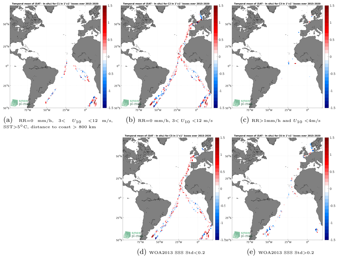
Figure 12: Temporal mean gridded over spatial boxes of size 1^\circ \times 1^\circ of \Delta SSS (SMAP SSS L2 v5.0 (JPL) - TSG (Polarstern)) for 5 different subdatasets corresponding to:RR=0 mm/h, 3 < U_{10} < 12 m/s, SST >5^\circ\text{C} , distance to coast > 800 km (a), RR=0 mm/h, 3 < U_{10} < 12 m/s (b), RR >1 mm/h and U_{10} < 4 m/s (c), WOA2013 SSS Std <0.2 (d), WOA2013 SSS Std >0.2 (e).
