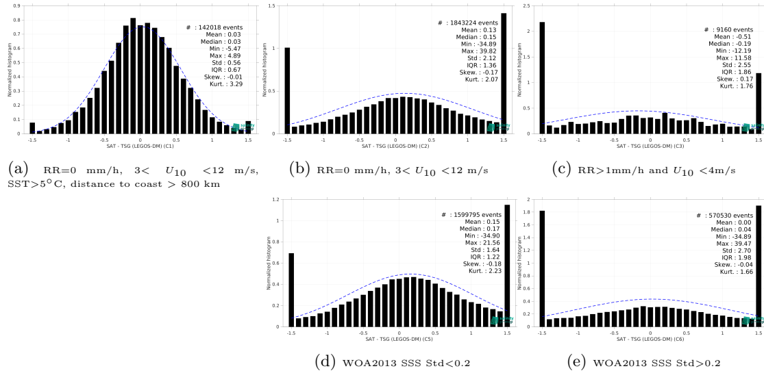
Figure 15: Normalized histogram of \Delta SSS (SMAP SSS L2 v5.0 (JPL) - TSG (LEGOS-DM)) for 5 different subdatasets corresponding to: RR=0 mm/h, 3 < U_{10} < 12 m/s, SST>5°C, distance to coast > 800 km (a), RR=0 mm/h, 3 < U_{10} < 12 m/s (b), RR>1mm/h and U_{10} < 4 m/s (c), WOA2013 SSS Std<0.2 (d), WOA2013 SSS Std>0.2 (e).
