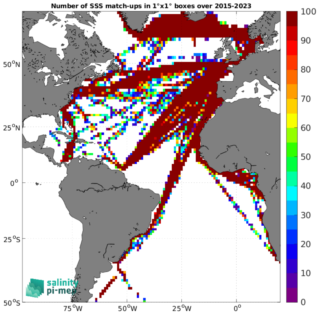
Figure 5: Number of SSS match-ups between TSG (LEGOS-DM) SSS and the SMAP SSS L2 v5.0 (JPL) SSS product for the Atlantic Ocean Pi-MEP region over 1°x1° boxes and for the full satellite product period.
