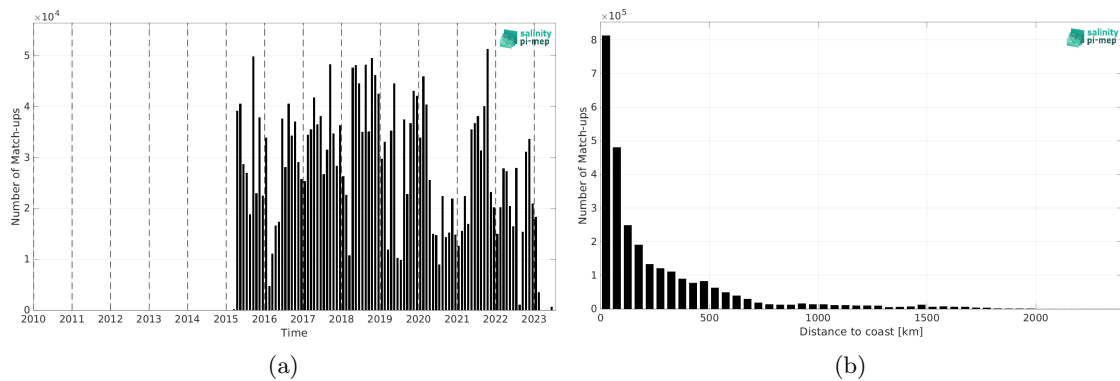
Figure 2: Number of match-ups between TSG (LEGOS-DM) and SMAP SSS L2 v5.0 (JPL) SSS as a function of time (a) and as function of the distance to coast (b) over the Atlantic Ocean Pi-MEP region and for the full satellite product period.
