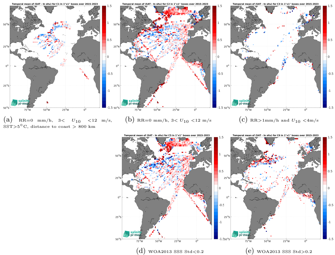
Figure 14: Temporal mean gridded over spatial boxes of size 1^\circ \times 1^\circ of \Delta\text{SSS} (SMAP SSS L2 v5.0 (JPL) - TSG (LEGOS-DM)) for 5 different subdatasets corresponding to:RR=0 mm/h, 3 < U_{10} < 12 m/s, SST >5^\circ\text{C} , distance to coast > 800 km (a), RR=0 mm/h, 3 < U_{10} < 12 m/s (b), RR >1 mm/h and U_{10} < 4 m/s (c), WOA2013 SSS Std <0.2 (d), WOA2013 SSS Std >0.2 (e).
