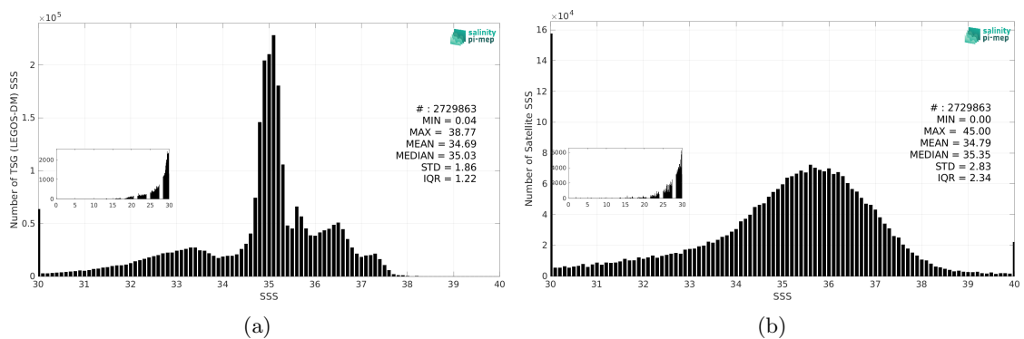
Figure 3: Histograms of SSS from TSG (LEGOS-DM) (a) and SMAP SSS L2 v5.0 (JPL) (b) considering all match-up pairs per bins of 0.1 over the Atlantic Ocean Pi-MEP region and for the full satellite product period.
