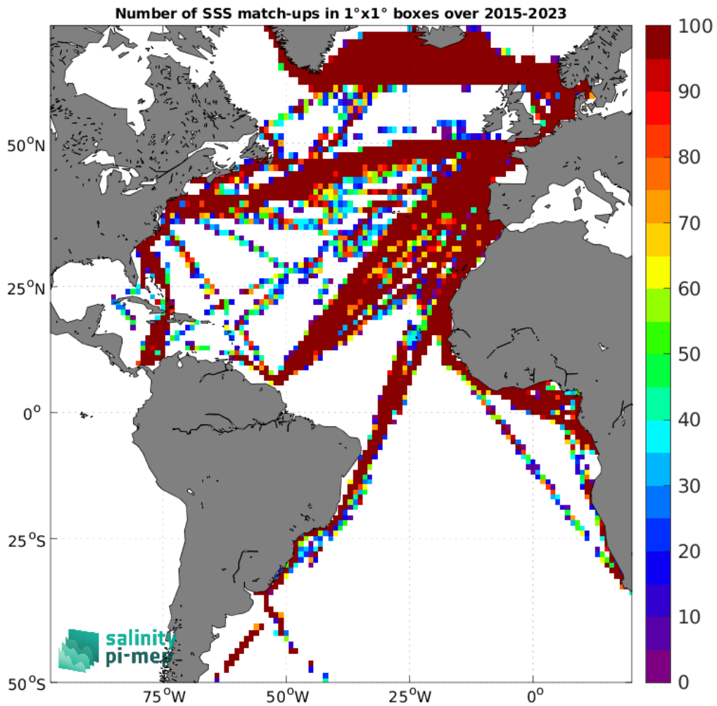
Figure 4: Number of SSS match-ups between TSG (LEGOS-DM) SSS and the SMAP SSS L2 v5.0 (JPL) SSS product for the Atlantic Ocean Pi-MEP region over 1^\circ \times 1^\circ boxes and for the full satellite product period.
