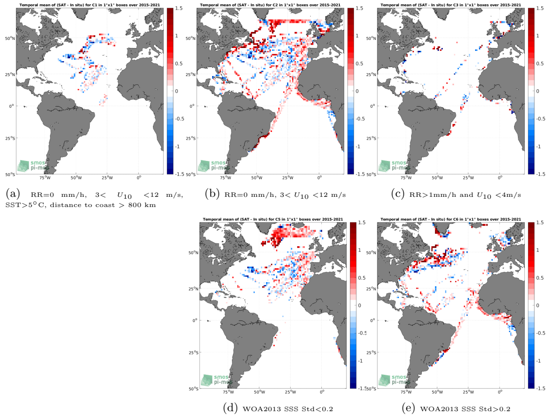
Figure 12: Temporal mean gridded over spatial boxes of size 1^\circ \times 1^\circ of \Delta\text{SSS} (SMAP SSS L2 v5.0 (JPL) - TSG (LEGOS-DM)) for 5 different subdatasets corresponding to:RR=0 mm/h, 3 < U_{10} < 12 m/s, SST >5^\circ\text{C} , distance to coast > 800 km (a), RR=0 mm/h, 3 < U_{10} < 12 m/s (b), RR >1 mm/h and U_{10} < 4 m/s (c), WOA2013 SSS Std <0.2 (d), WOA2013 SSS Std >0.2 (e).
