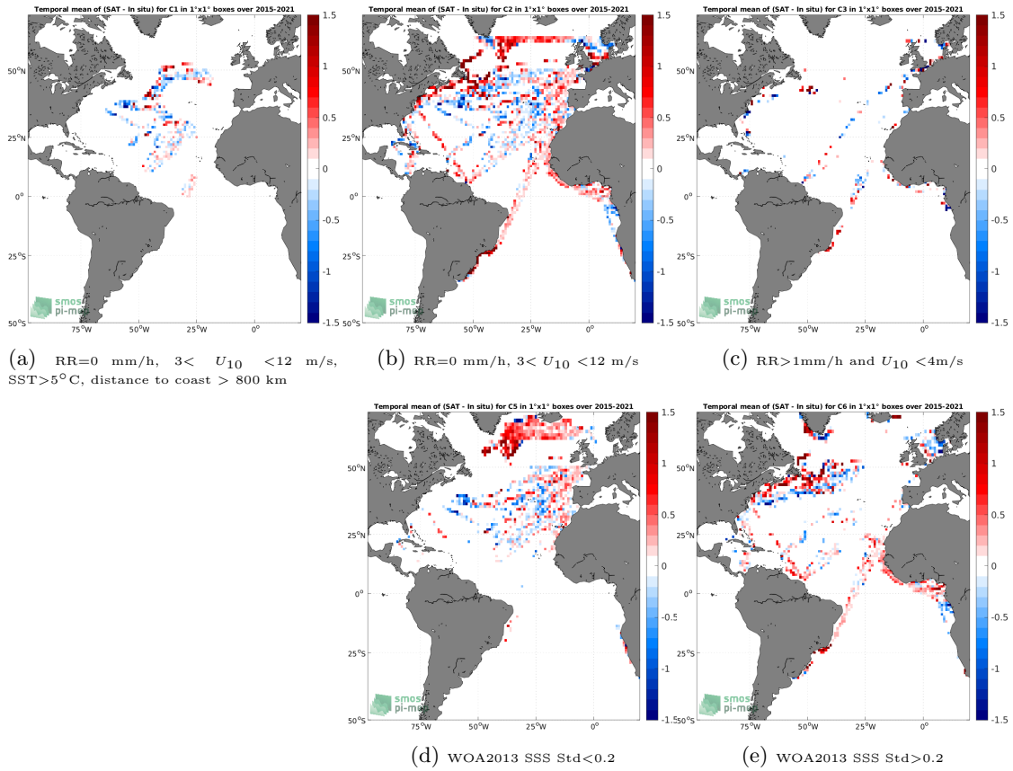
Figure 12: Temporal mean gridded over spatial boxes of size 1^\circ \times 1^\circ of \Delta SSS (SMAP SSS L2 v5.0 (JPL) - TSG (LEGOS-DM)) for 5 different subdatasets corresponding to:RR=0 mm/h, 3 < U_{10} < 12 m/s, SST >5^\circ\text{C} , distance to coast > 800 km (a), RR=0 mm/h, 3 < U_{10} < 12 m/s (b), RR >1 mm/h and U_{10} < 4 m/s (c), WOA2013 SSS Std <0.2 (d), WOA2013 SSS Std >0.2 (e).
