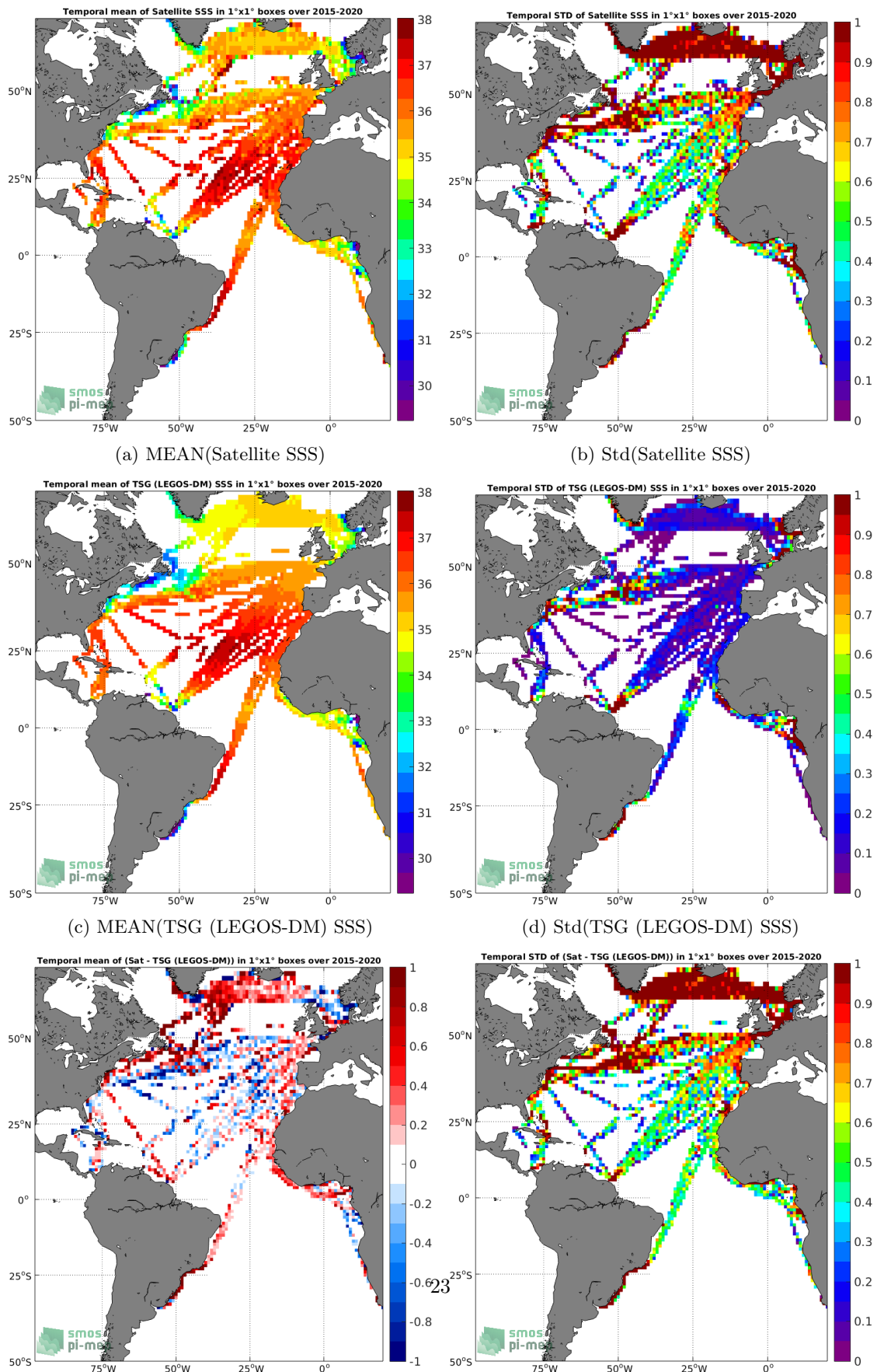
(e) MEAN( \Delta SSS) (Satellite - TSG (LEGOS-DM)) (f) Std( \Delta SSS) (Satellite - TSG (LEGOS-DM)) Figure 6: Temporal mean (left) and Std (right) of SSS from SMAP SSS L2 v5.0 (JPL) (top), TSG (LEGOS-DM) (middle), and of \Delta SSS (Satellite - TSG (LEGOS-DM)). Only match-up pairs are used to generate these maps.
