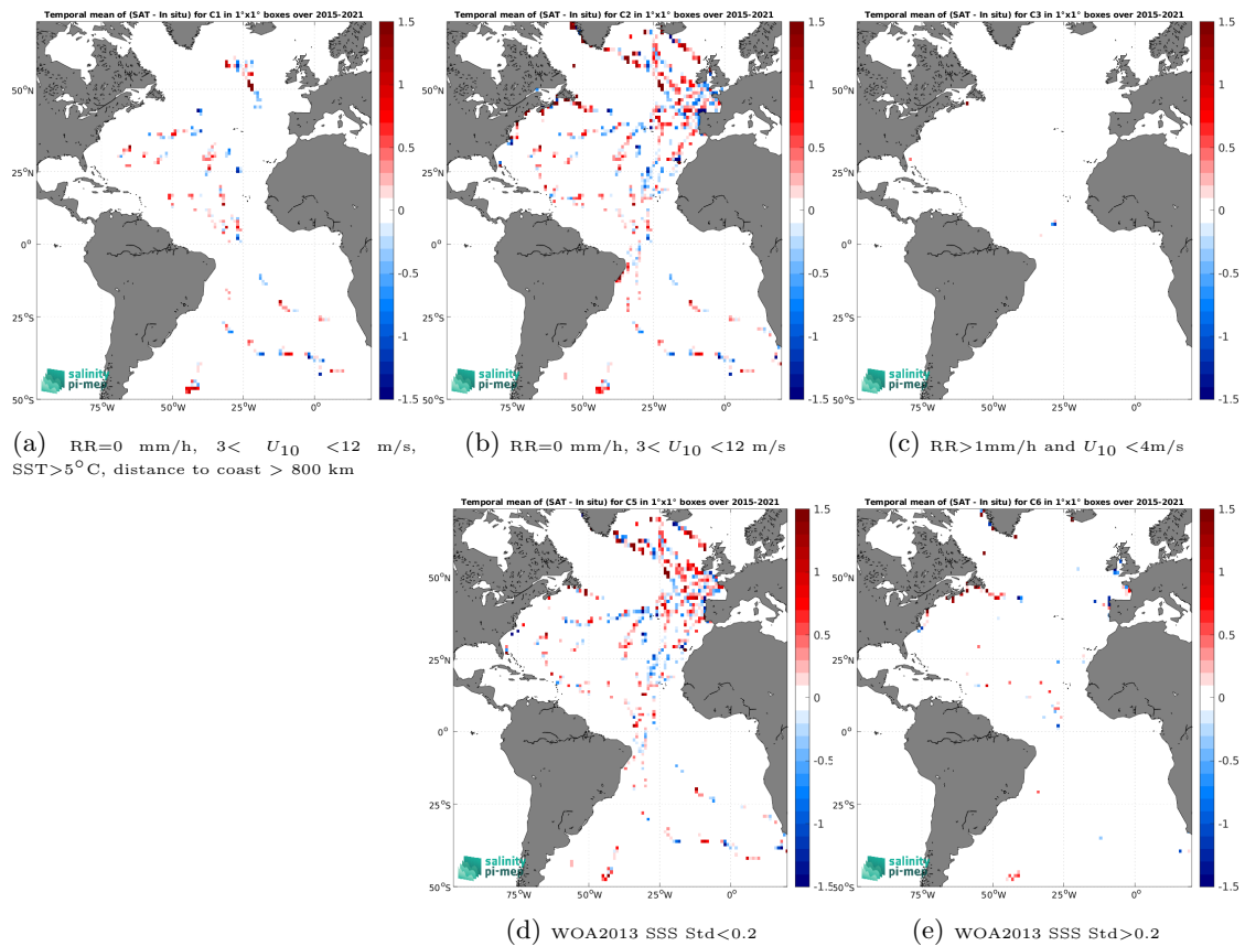
Figure 14: Temporal mean gridded over spatial boxes of size 1^\circ \times 1^\circ of \Delta\text{SSS} (SMAP SSS L2 v5.0 (JPL) - TSG (GOSUD-Sailing-ship)) for 5 different subdatasets corresponding to:RR=0 mm/h, 3 < U_{10} < 12 m/s, SST >5^\circ\text{C} , distance to coast > 800 km (a), RR=0 mm/h, 3 < U_{10} < 12 m/s (b), RR >1 mm/h and U_{10} < 4 m/s (c), WOA2013 SSS Std <0.2 (d), WOA2013 SSS Std >0.2 (e).
