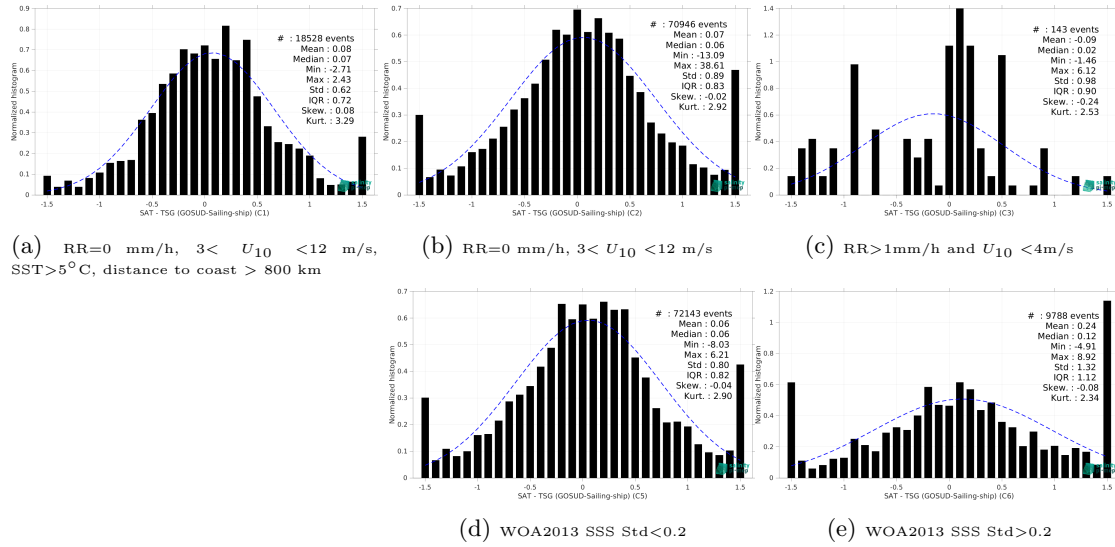
Figure 15: Normalized histogram of \Delta\text{SSS} (SMAP SSS L2 v5.0 (JPL) - TSG (GOSUD-Sailing-ship)) for 5 different subdatasets corresponding to: RR=0 mm/h, 3 < U_{10} < 12 m/s, SST >5^{\circ}\text{C} , distance to coast > 800 km (a), RR=0 mm/h, 3 < U_{10} < 12 m/s (b), RR >1 mm/h and U_{10} < 4 m/s (c), WOA2013 SSS Std <0.2 (d), WOA2013 SSS Std >0.2 (e).
