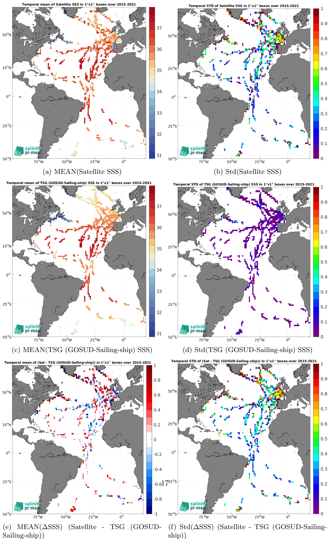
Figure 7: Temporal mean (left) and Std (right) of SSS from SMAP SSS L2 v5.0 (JPL) (top), TSG (GOSUD-Sailing-ship) (middle), and of \Delta SSS (Satellite - TSG (GOSUD-Sailing-ship)). Only match-up pairs are used to generate these maps.
