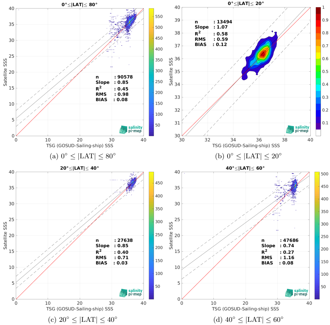
Figure 10: Contour maps of the concentration of SMAP SSS L2 v5.0 (JPL) SSS (y-axis) versus TSG (GOSUD-Sailing-ship) SSS (x-axis) at match-up pairs for different latitude bands. For each plot, the red line shows x=y . The black thin and dashed lines indicate a linear fit through the data cloud and the \pm 95\% confidence levels, respectively. The number match-up pairs n , the slope and R^2 coefficient of the linear fit, the root mean square (RMS) and the mean bias between satellite and in situ data are indicated for each latitude band in each plots.
