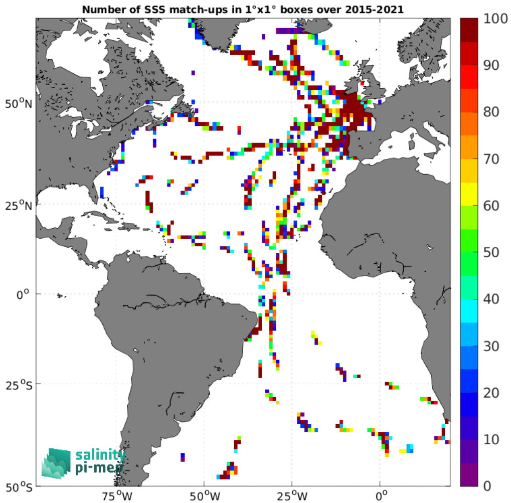
Figure 5: Number of SSS match-ups between TSG (GOSUD-Sailing-ship) SSS and the SMAP SSS L2 v5.0 (JPL) SSS product for the Atlantic Ocean Pi-MEP region over 1^\circ \times 1^\circ boxes and for the full satellite product period.
