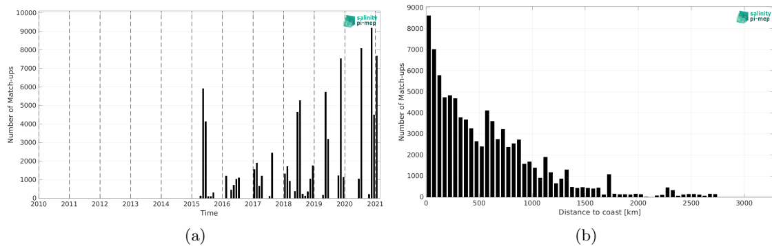
Figure 2: Number of match-ups between TSG (GOSUD-Sailing-ship) and SMAP SSS L2 v5.0 (JPL) SSS as a function of time (a) and as function of the distance to coast (b) over the Atlantic Ocean Pi-MEP region and for the full satellite product period.
