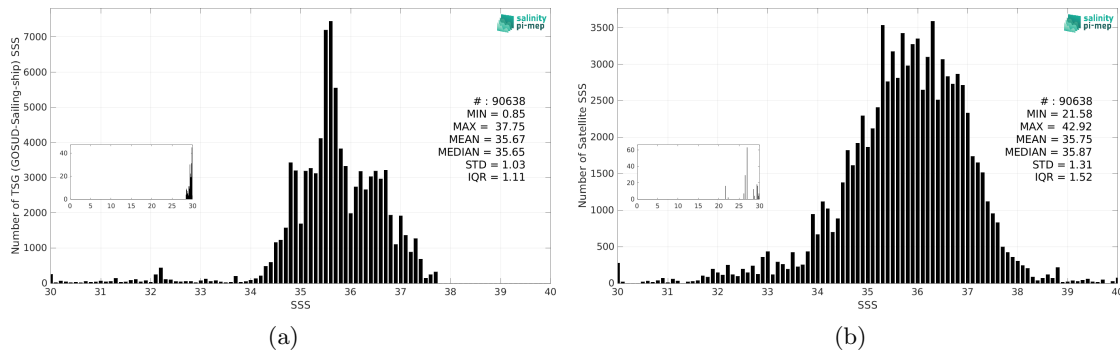
Figure 3: Histograms of SSS from TSG (GOSUD-Sailing-ship) (a) and SMAP SSS L2 v5.0 (JPL) (b) considering all match-up pairs per bins of 0.1 over the Atlantic Ocean Pi-MEP region and for the full satellite product period.
