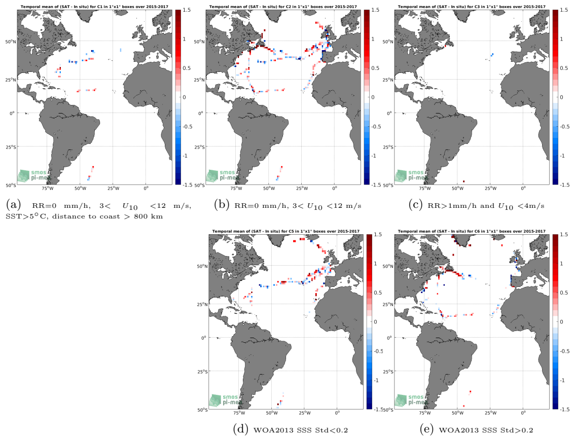
Figure 12: Temporal mean gridded over spatial boxes of size 1^\circ \times 1^\circ of \Delta SSS (SMAP SSS L2 v5.0 (JPL) - TSG (GOSUD-Sailing-ship)) for 5 different subdatasets corresponding to: RR=0 mm/h, 3 < U_{10} < 12 m/s, SST > 5°C, distance to coast > 800 km (a), RR=0 mm/h, 3 < U_{10} < 12 m/s (b), RR > 1mm/h and U_{10} < 4 m/s (c), WOA2013 SSS Std < 0.2 (d), WOA2013 SSS Std > 0.2 (e).
