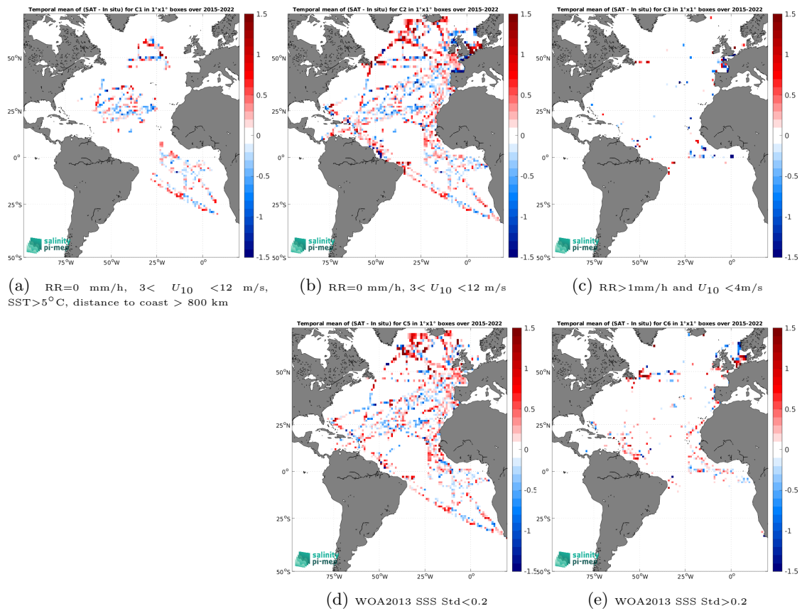
Figure 14: Temporal mean gridded over spatial boxes of size 1^\circ \times 1^\circ of \Delta SSS (SMAP SSS L2 v5.0 (JPL) - TSG (GOSUD-Research-vessel)) for 5 different subdatasets corresponding to:RR=0 mm/h, 3 < U_{10} < 12 m/s, SST>5°C, distance to coast > 800 km (a), RR=0 mm/h, 3 < U_{10} < 12 m/s (b), RR>1mm/h and U_{10} < 4 m/s (c), WOA2013 SSS Std<0.2 (d), WOA2013 SSS Std>0.2 (e).
