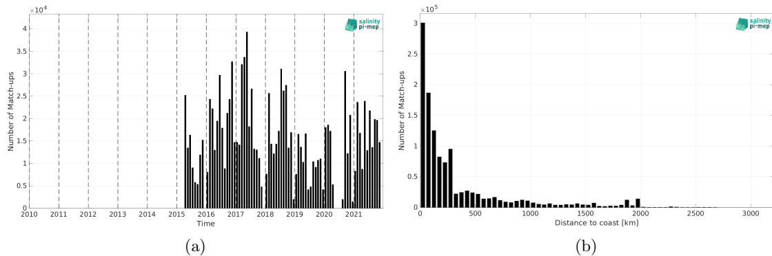
Figure 2: Number of match-ups between TSG (GOSUD-Research-vessel) and SMAP SSS L2 v5.0 (JPL) SSS as a function of time (a) and as function of the distance to coast (b) over the Atlantic Ocean Pi-MEP region and for the full satellite product period.
