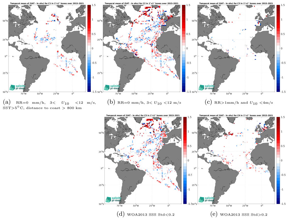
Figure 14: Temporal mean gridded over spatial boxes of size 1^\circ \times 1^\circ of \Delta\text{SSS} (SMAP SSS L2 v5.0 (JPL) - TSG (GOSUD-Research-vessel)) for 5 different subdatasets corresponding to:RR=0 mm/h, 3 < U_{10} < 12 m/s, SST >5^\circ\text{C} , distance to coast > 800 km (a), RR=0 mm/h, 3 < U_{10} < 12 m/s (b), RR >1 mm/h and U_{10} < 4 m/s (c), WOA2013 SSS Std <0.2 (d), WOA2013 SSS Std >0.2 (e).
