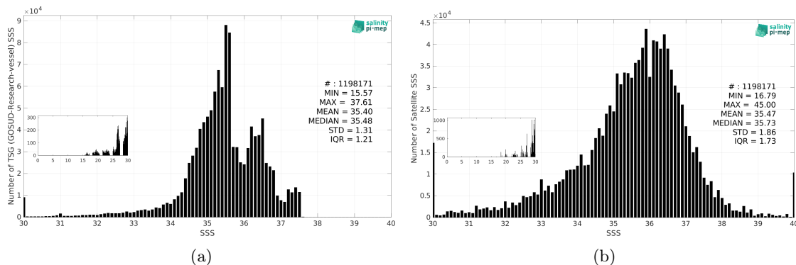
Figure 3: Histograms of SSS from TSG (GOSUD-Research-vessel) (a) and SMAP SSS L2 v5.0 (JPL) (b) considering all match-up pairs per bins of 0.1 over the Atlantic Ocean Pi-MEP region and for the full satellite product period.
