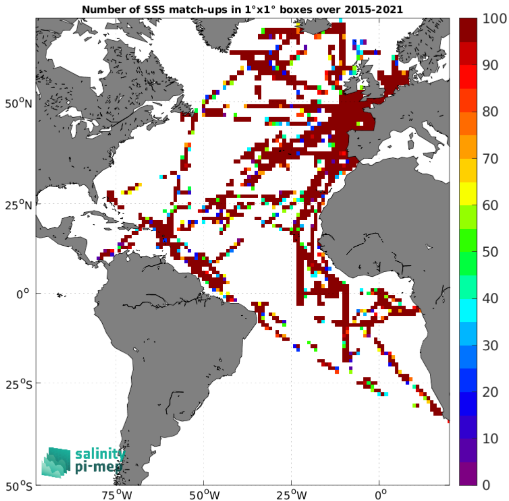
Figure 5: Number of SSS match-ups between TSG (GOSUD-Research-vessel) SSS and the SMAP SSS L2 v5.0 (JPL) SSS product for the Atlantic Ocean Pi-MEP region over 1°x1° boxes and for the full satellite product period.
