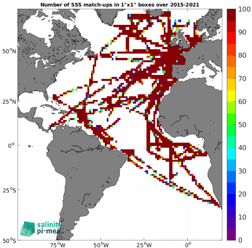
Figure 4: Number of SSS match-ups between TSG (GOSUD-Research-vessel) SSS and the SMAP SSS L2 v5.0 (JPL) SSS product for the Atlantic Ocean Pi-MEP region over 1^\circ \times 1^\circ boxes and for the full satellite product period.
