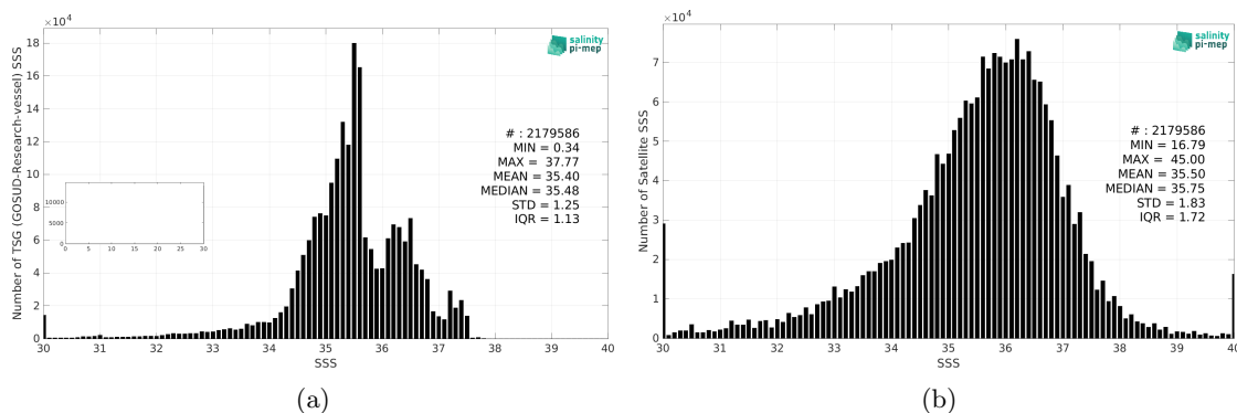
Figure 2: Histograms of SSS from TSG (GOSUD-Research-vessel) (a) and SMAP SSS L2 v5.0 (JPL) (b) considering all match-up pairs per bins of 0.1 over the Atlantic Ocean Pi-MEP region and for the full satellite product period.
