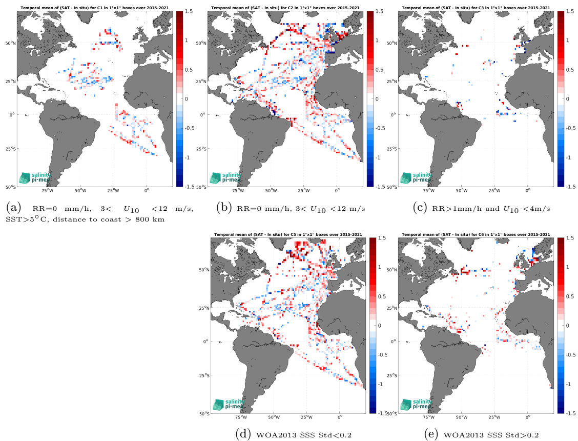
Figure 12: Temporal mean gridded over spatial boxes of size 1^\circ \times 1^\circ of \Delta\text{SSS} (SMAP SSS L2 v5.0 (JPL) - TSG (GOSUD-Research-vessel)) for 5 different subdatasets corresponding to:RR=0 mm/h, 3 < U_{10} < 12 m/s, SST>5°C, distance to coast > 800 km (a), RR=0 mm/h, 3 < U_{10} < 12 m/s (b), RR>1mm/h and U_{10} < 4 m/s (c), WOA2013 SSS Std<0.2 (d), WOA2013 SSS Std>0.2 (e).
