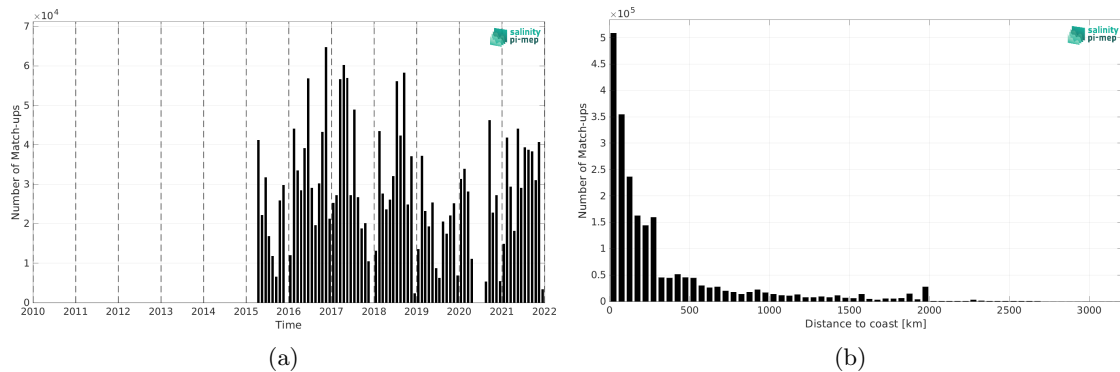
Figure 1: Number of match-ups between TSG (GOSUD-Research-vessel) and SMAP SSS L2 v5.0 (JPL) SSS as a function of time (a) and as function of the distance to coast (b) over the Atlantic Ocean Pi-MEP region and for the full satellite product period.
