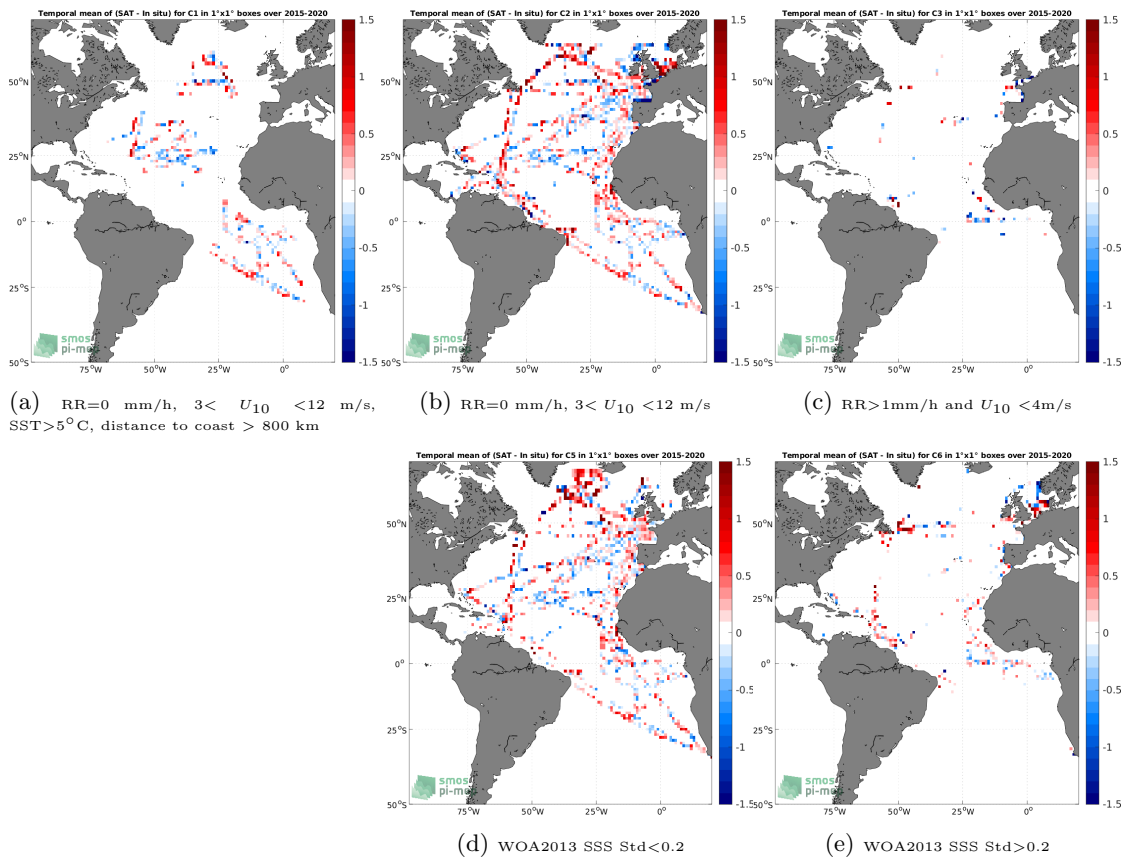
Figure 12: Temporal mean gridded over spatial boxes of size 1^\circ \times 1^\circ of \Delta SSS (SMAP SSS L2 v5.0 (JPL) - TSG (GOSUD-Research-vessel)) for 5 different subdatasets corresponding to:RR=0 mm/h, 3 < U_{10} < 12 m/s, SST>5°C, distance to coast > 800 km (a), RR=0 mm/h, 3 < U_{10} < 12 m/s (b), RR>1mm/h and U_{10} < 4 m/s (c), WOA2013 SSS Std<0.2 (d), WOA2013 SSS Std>0.2 (e).
