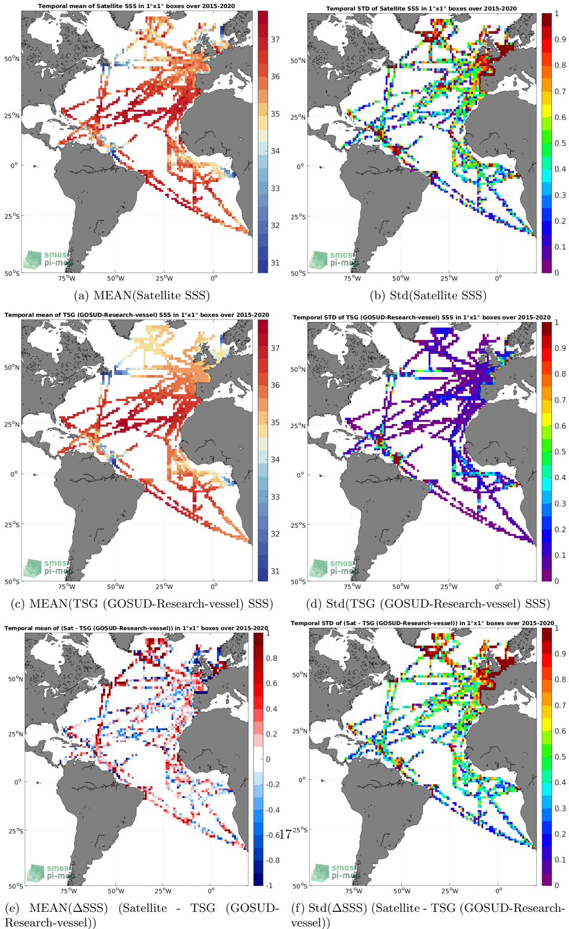
Figure 6: Temporal mean (left) and Std (right) of SSS from SMAP SSS L2 v5.0 (JPL) (top), TSG (GOSUD-Research-vessel) (middle), and of \Delta SSS (Satellite - TSG (GOSUD-Research-vessel)). Only match-up pairs are used to generate these maps.
