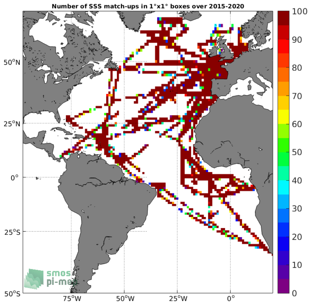
Figure 4: Number of SSS match-ups between TSG (GOSUD-Research-vessel) SSS and the SMAP SSS L2 v5.0 (JPL) SSS product for the Atlantic Ocean Pi-MEP region over 1°x1° boxes and for the full satellite product period.
