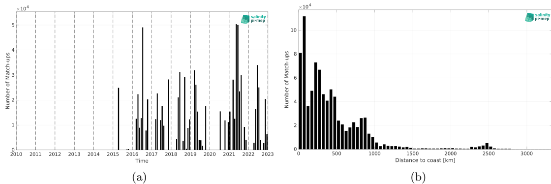
Figure 2: Number of match-ups between TSG (CSIC-UTM) and SMAP SSS L2 v5.0 (JPL) SSS as a function of time (a) and as function of the distance to coast (b) over the Atlantic Ocean Pi-MEP region and for the full satellite product period.
