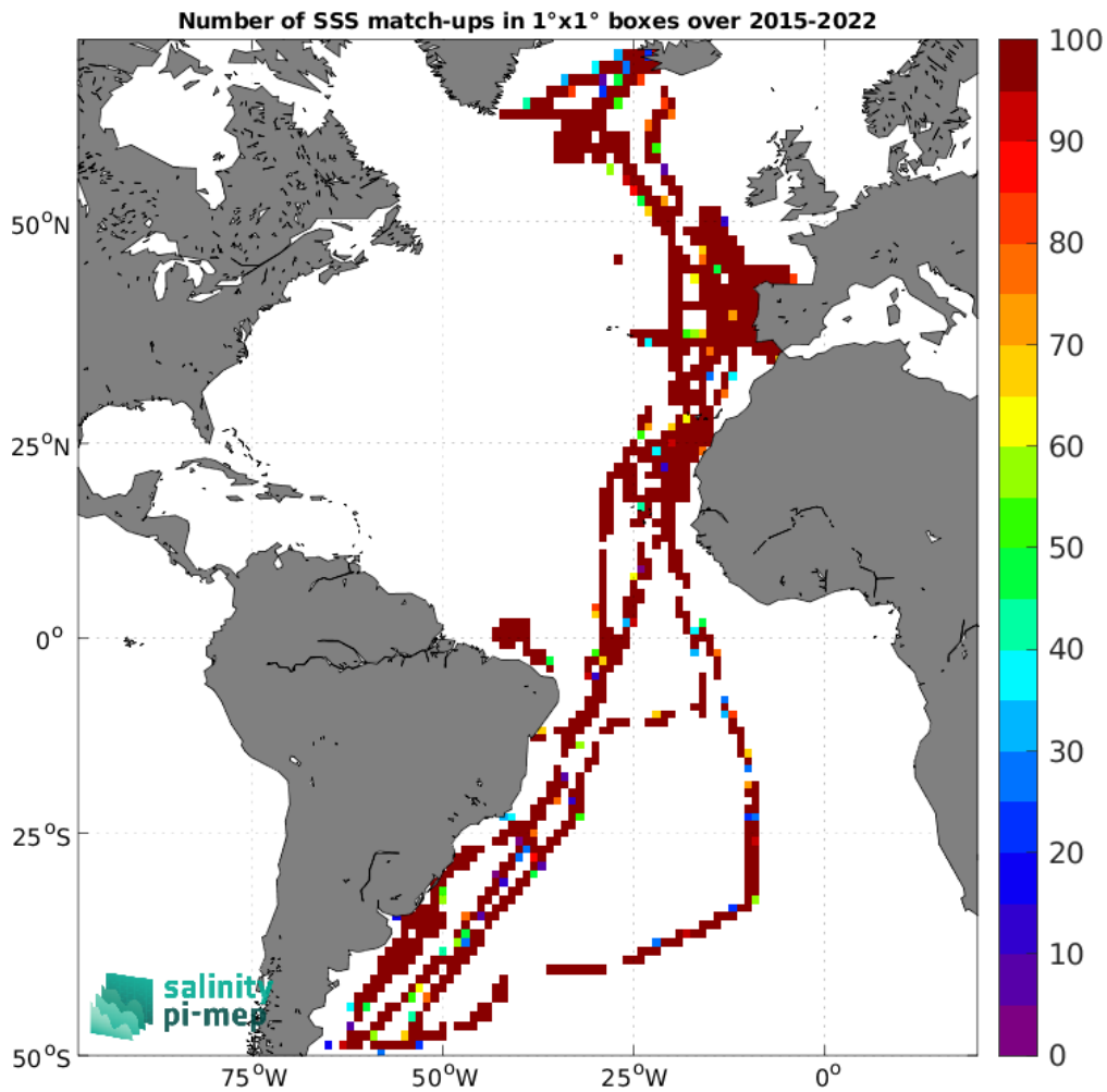
Figure 5: Number of SSS match-ups between TSG (CSIC-UTM) SSS and the SMAP SSS L2 v5.0 (JPL) SSS product for the Atlantic Ocean Pi-MEP region over 1^\circ \times 1^\circ boxes and for the full satellite product period.
