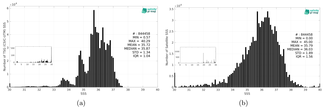
Figure 3: Histograms of SSS from TSG (CSIC-UTM) (a) and SMAP SSS L2 v5.0 (JPL) (b) considering all match-up pairs per bins of 0.1 over the Atlantic Ocean Pi-MEP region and for the full satellite product period.
