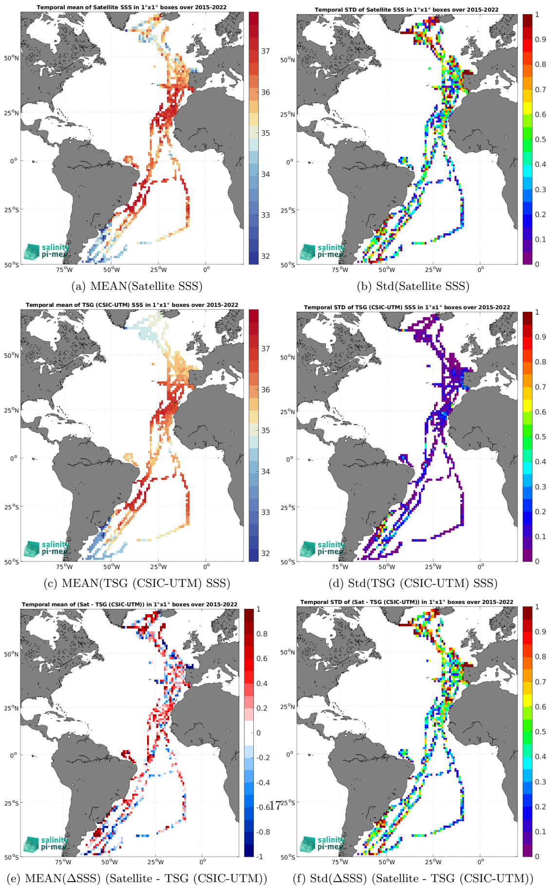
(e) MEAN( \Delta SSS) (Satellite - TSG (CSIC-UTM)) (f) Std( \Delta SSS) (Satellite - TSG (CSIC-UTM)) Figure 7: Temporal mean (left) and Std (right) of SSS from SMAP SSS L2 v5.0 (JPL) (top), TSG (CSIC-UTM) (middle), and of \Delta SSS (Satellite - TSG (CSIC-UTM)). Only match-up pairs are used to generate these maps.
