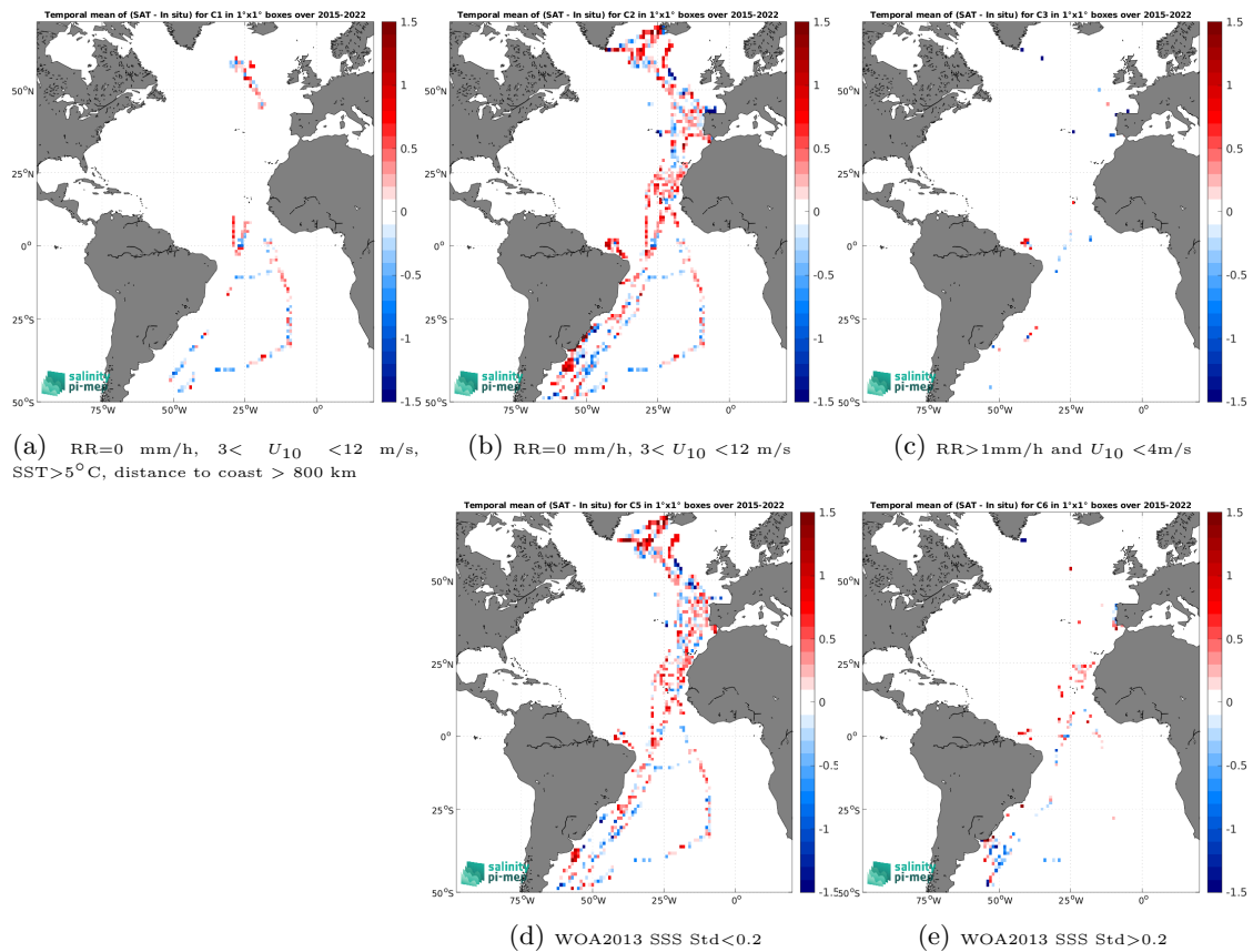
Figure 14: Temporal mean gridded over spatial boxes of size 1^\circ \times 1^\circ of \Delta\text{SSS} (SMAP SSS L2 v5.0 (JPL) - TSG (CSIC-UTM)) for 5 different subdatasets corresponding to:RR=0 mm/h, 3 < U_{10} < 12 m/s, SST >5^\circ\text{C} , distance to coast > 800 km (a), RR=0 mm/h, 3 < U_{10} < 12 m/s (b), RR >1 mm/h and U_{10} < 4 m/s (c), WOA2013 SSS Std <0.2 (d), WOA2013 SSS Std >0.2 (e).
