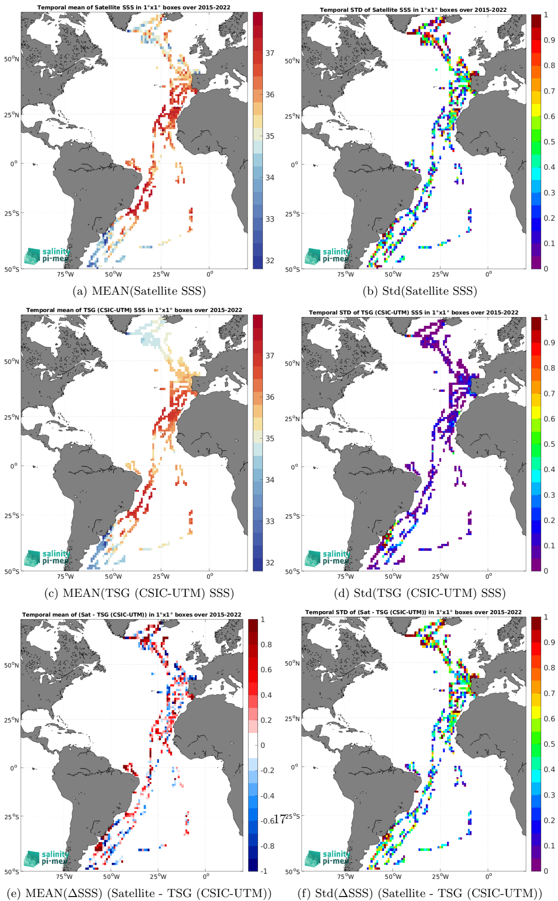
Figure 7: Temporal mean (left) and Std (right) of SSS from SMAP SSS L2 v5.0 (JPL) (top), TSG (CSIC-UTM) (middle), and of \Delta SSS (Satellite - TSG (CSIC-UTM)). Only match-up pairs are used to generate these maps.
