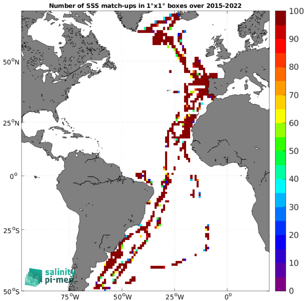
Figure 5: Number of SSS match-ups between TSG (CSIC-UTM) SSS and the SMAP SSS L2 v5.0 (JPL) SSS product for the Atlantic Ocean Pi-MEP region over 1°×1° boxes and for the full satellite product period.
