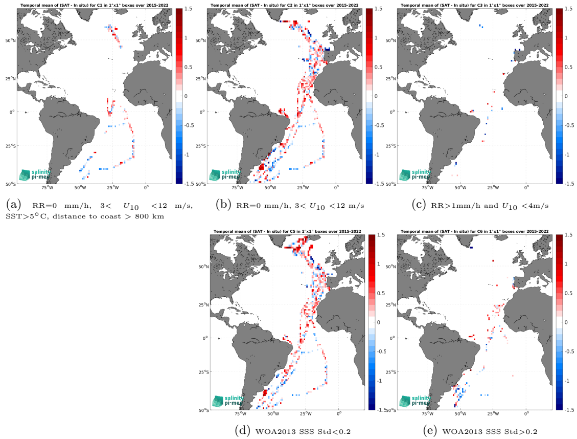
Figure 12: Temporal mean gridded over spatial boxes of size 1^\circ \times 1^\circ of \Delta\text{SSS} (SMAP SSS L2 v5.0 (JPL) - TSG (CSIC-UTM)) for 5 different subdatasets corresponding to:RR=0 mm/h, 3 < U_{10} < 12 m/s, SST >5^\circ\text{C} , distance to coast > 800 km (a), RR=0 mm/h, 3 < U_{10} < 12 m/s (b), RR >1 mm/h and U_{10} < 4 m/s (c), WOA2013 SSS Std <0.2 (d), WOA2013 SSS Std >0.2 (e).
