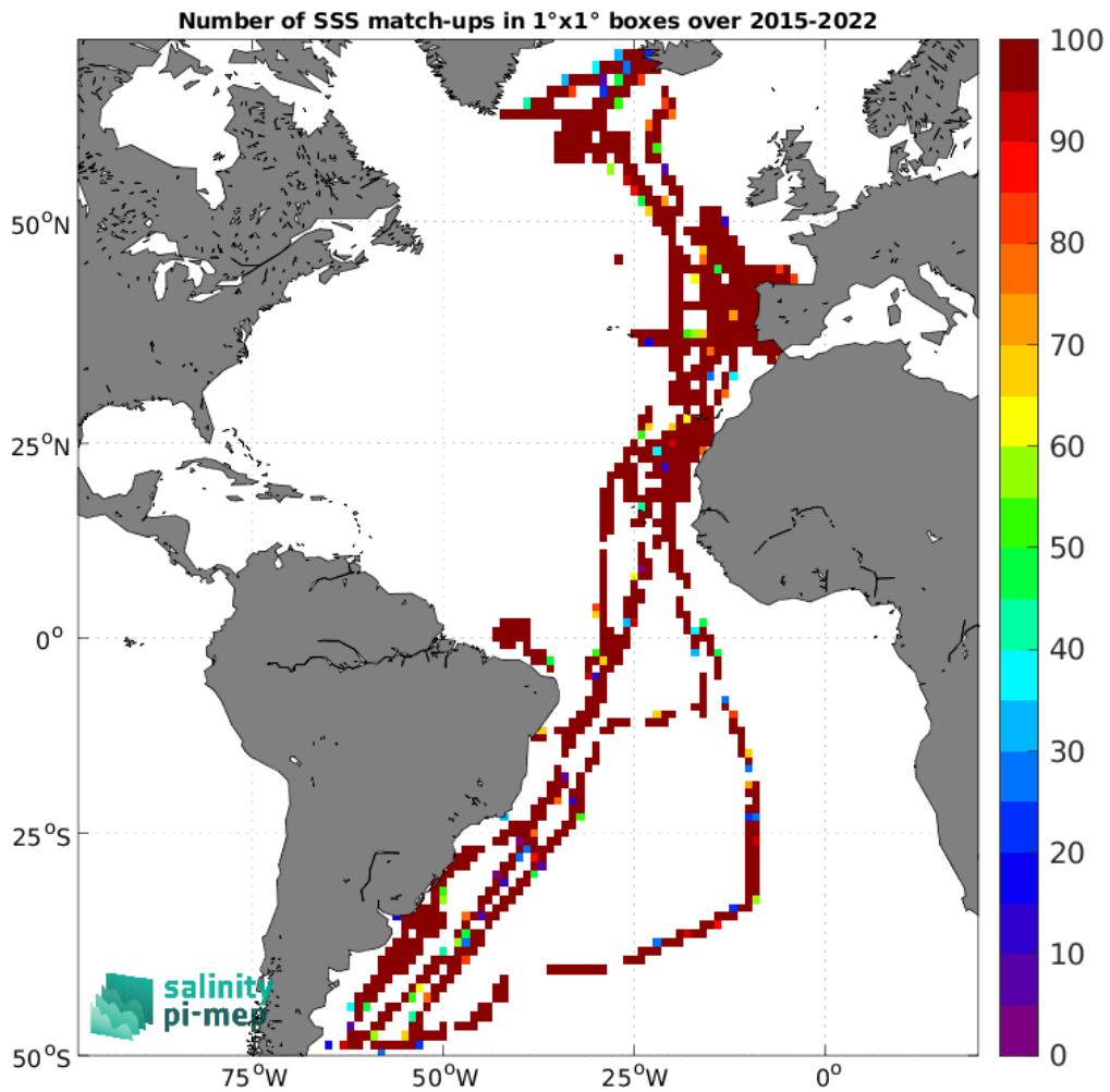
Figure 4: Number of SSS match-ups between TSG (CSIC-UTM) SSS and the SMAP SSS L2 v5.0 (JPL) SSS product for the Atlantic Ocean Pi-MEP region over 1°×1° boxes and for the full satellite product period.
